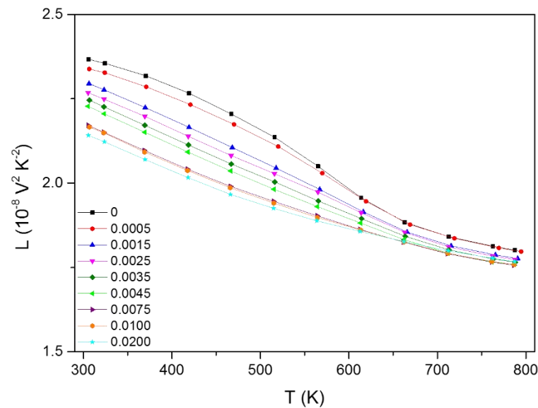
Figure 3.42: Temperature dependence of the Lorenz number L for the series \text{Sn}_{1.03-x}\text{In}_x\text{Te} calculated by a single parabolic band (SPB) model.
