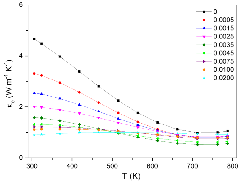
Figure 3.44: Electronic thermal conductivity \kappa_e evaluated by subtracting the lattice thermal conductivity \kappa_{ph} of the x = 0.02 sample from \kappa which is assumed to be constant across the series.
