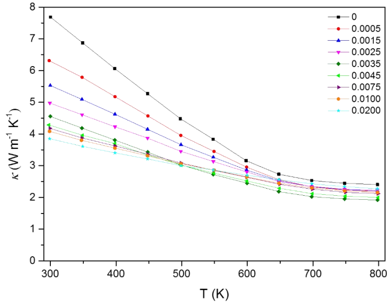
Figure 3.40: Total thermal conductivity \kappa as a function of the temperature for the series \text{Sn}_{1.03-x}\text{In}_x\text{Te} ( 0 \leq x \leq 0.02 ). The solid lines are guides to the eye.
