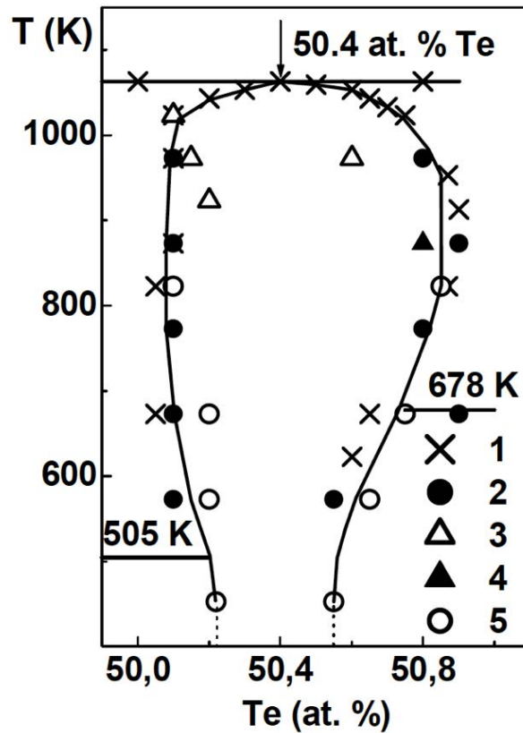
Figure 2.2: Homogeneity region of SnTe. 22
