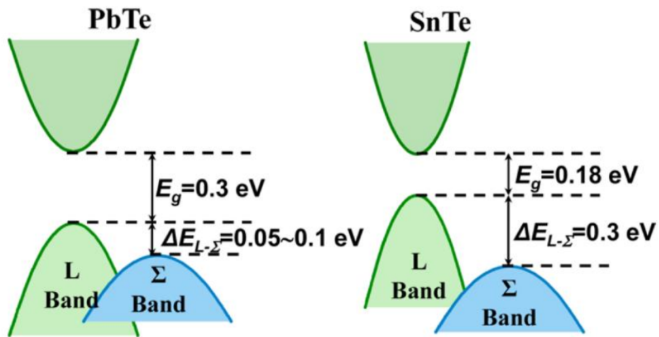
Figure 2.8: Electronic band structure comparison between PbTe and SnTe at 300 K. 55
