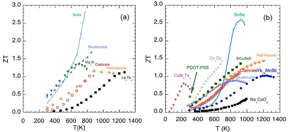
Figure 1.8: Temperature dependence of the ZT value for a) p-type and b) n-type advanced thermoelectric materials. 6
