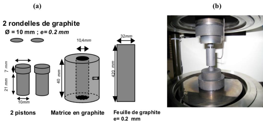
Figure A.2. a) Schematic details of graphite matrix and punches used in this thesis work b) Photograph of the die inside the SPS chamber. 3
