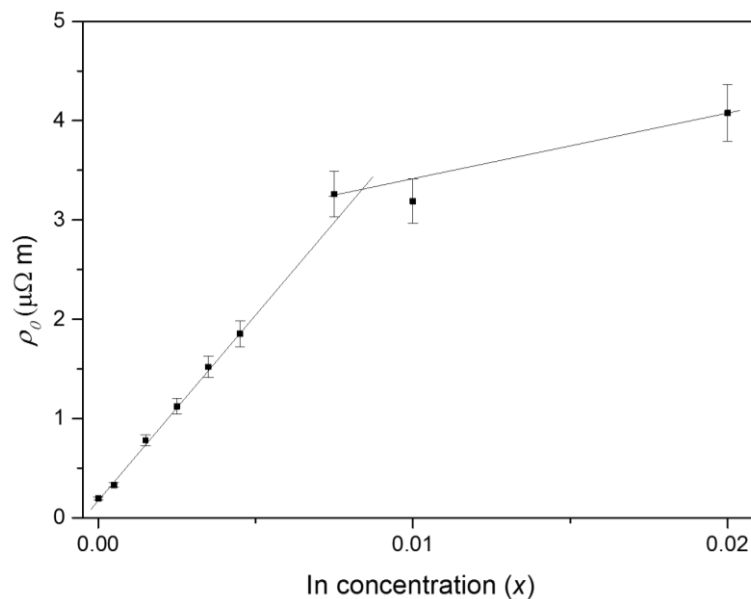
Figure 3.30: Residual electrical resistivity \rho_0 as a function of the In concentration x . The solid lines are guides to the eye.
