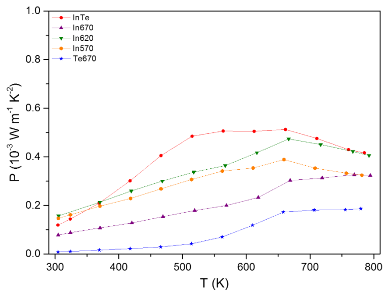
Figure 4.53: Temperature dependence of the power factor for the saturation-annealed polycrystalline samples on the In-rich and Te-rich side of the solidus.
