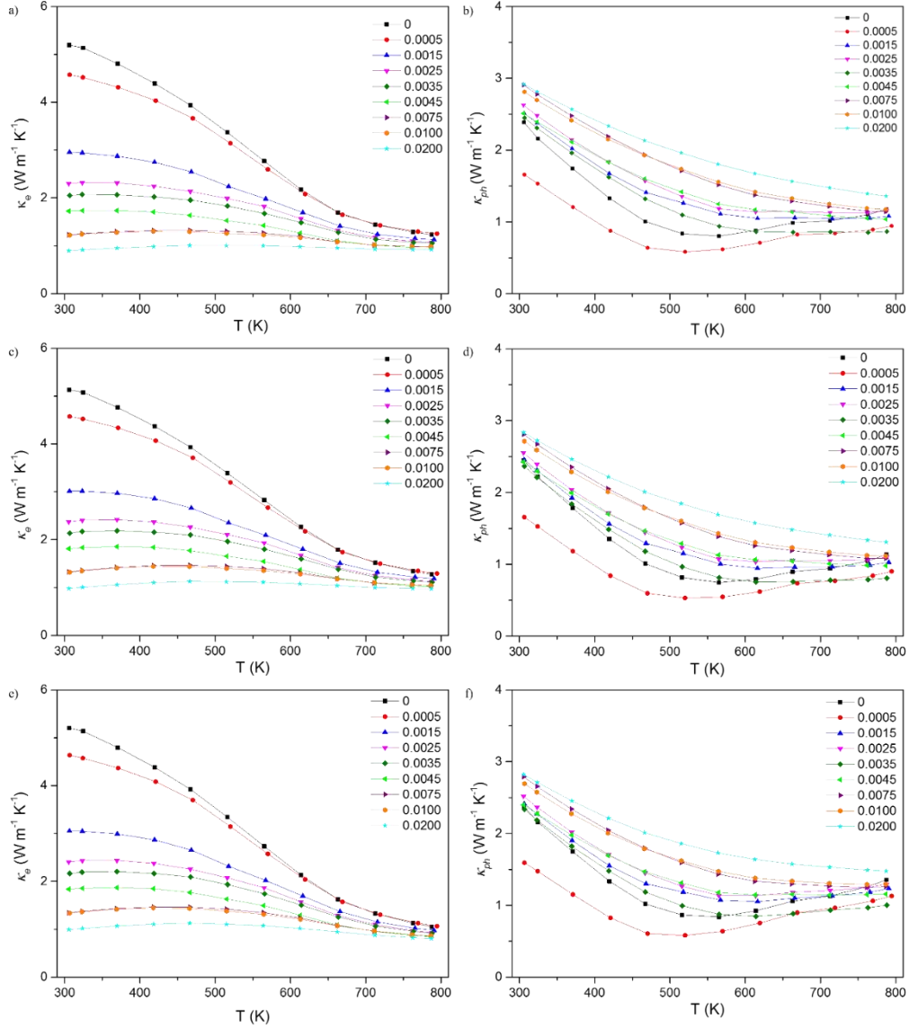
Figure 3.43: Temperature dependence of the a) electronic thermal conductivity \kappa_e (SPB model) b) lattice thermal conductivity \kappa_{ph} (SPB model) c) electronic thermal conductivity \kappa_e (TI-TVB model) d) lattice thermal conductivity \kappa_{ph} (TI-TVB model) e) electronic thermal conductivity \kappa_e (TD-TVB model) and f) lattice thermal conductivity \kappa_{ph} (TD-TVB model) of the series \text{Sn}_{1.03-x}\text{In}_x\text{Te} .
