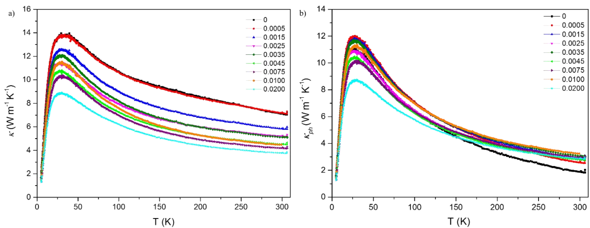
Figure 3.29: Temperature dependence of the a) total thermal conductivity \kappa for the series \text{Sn}_{1.03-x}\text{In}_x\text{Te} and b) lattice thermal conductivity \kappa for the series \text{Sn}_{1.03-x}\text{In}_x\text{Te} calculated using a single band model.
