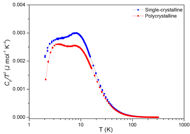
Figure 4.20: C_p/T^3 as a function of T for single-crystalline and polycrystalline InTe measured using the 4 He option of the PPMS system. No subtraction of the electronic contribution \gamma T has been performed.
