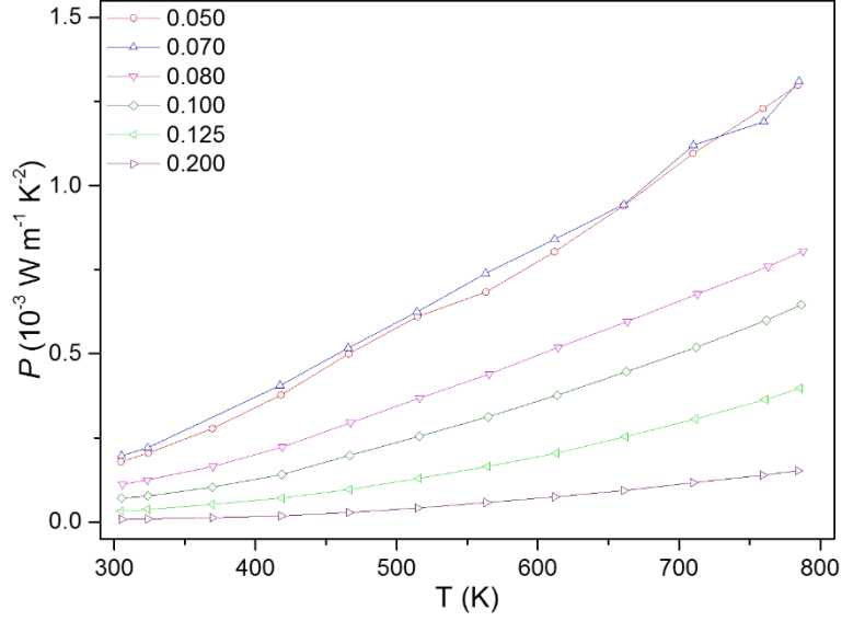
Figure 3.52: High temperature dependence of power factor for samples of \text{Sn}_{1-x}\text{In}_x\text{Te} series.
