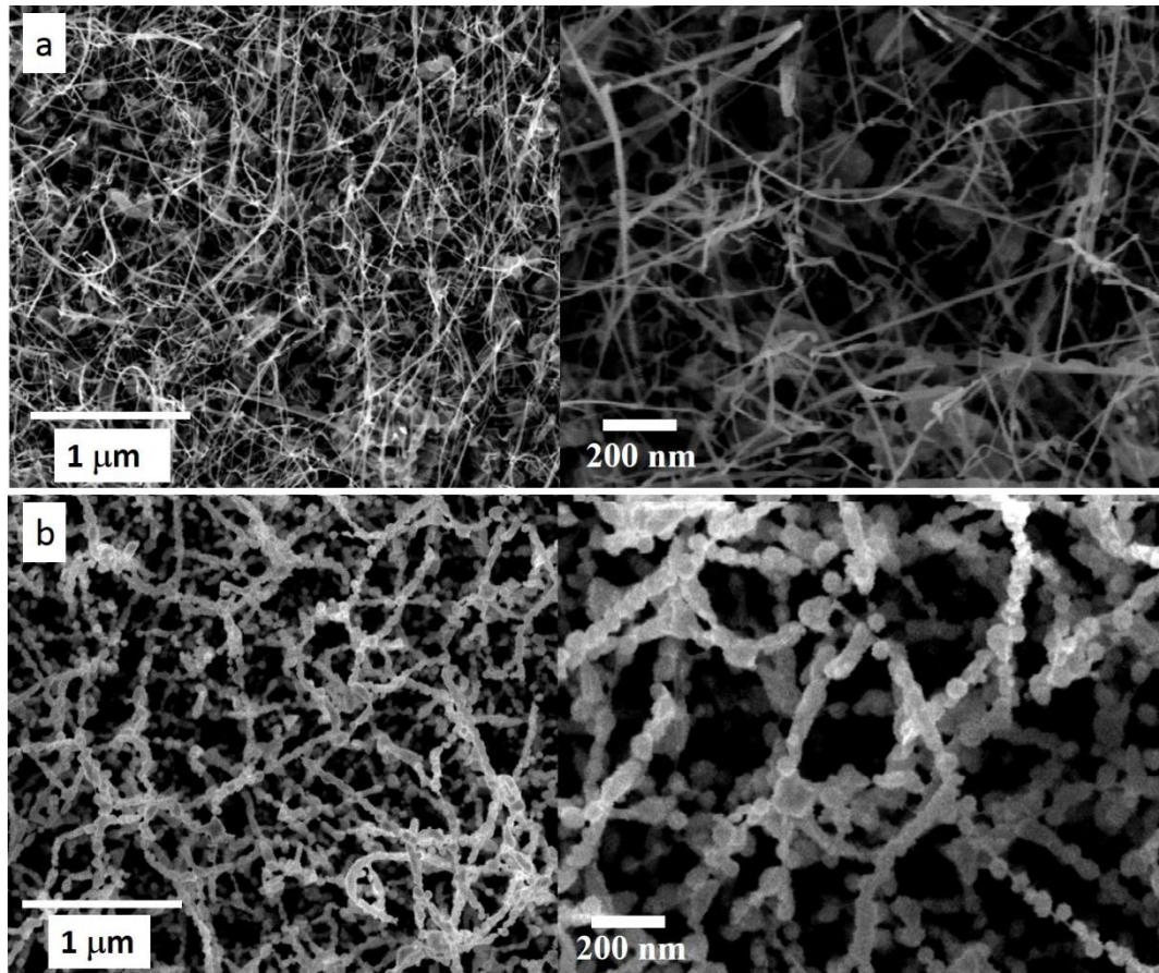
Figure 4.12. Top- view SEM micrographs of the as-grown ZnO nanowires (a) and after the deposition of the Cu NP by ALD (b). On the right, are presented magnified micrographs.
