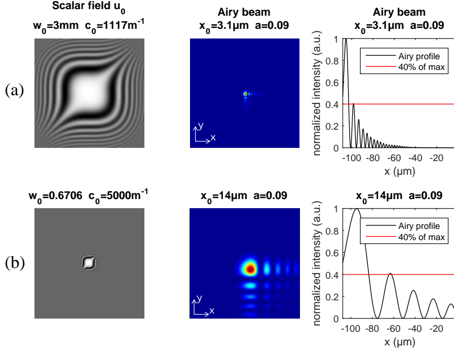
Figure 2.15: Two Airy beams of different size, each with a secondary lobe peak intensity equal to 40% of the main peak intensity. w_0 and c_0 are chosen as limit cases of condition 2.20.
