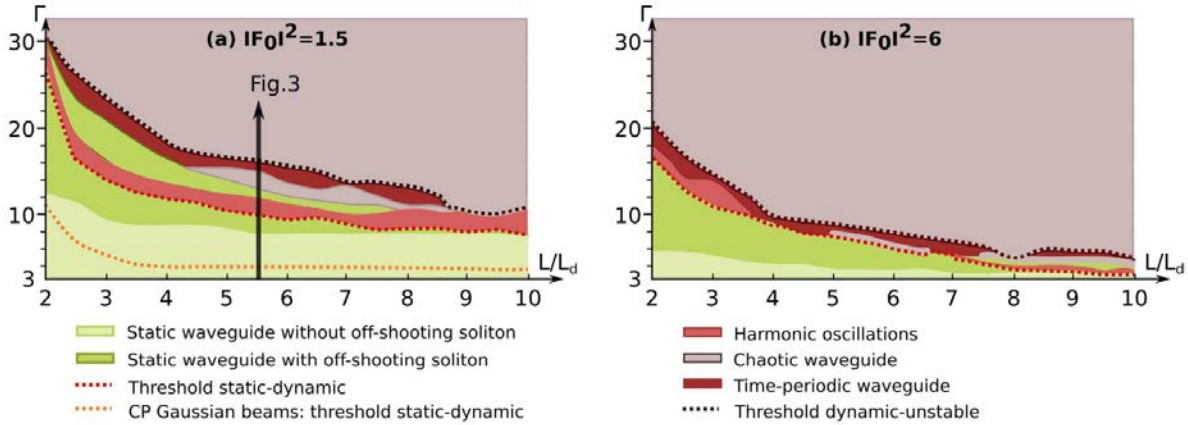
Figure 5.8: Typical dynamical behavior of counterpropagating Airy beams in the parameter plane (nonlinear strength \Gamma , crystal length L ): (a) with low input intensities (b) with higher input intensities.
