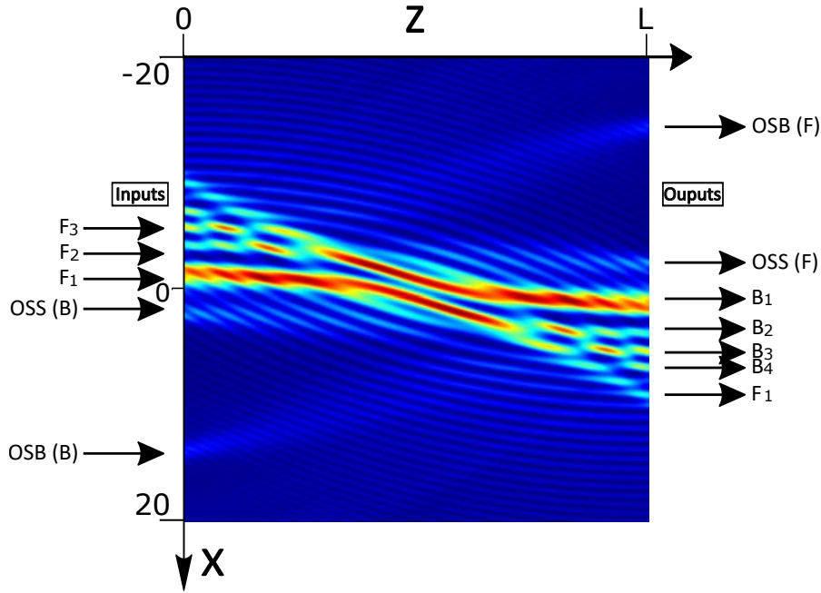
Figure 5.10: Intensity distribution of two counterpropagating antisymmetrical Airy beams in non-linear self-focusing conditions with d = 1 , \Gamma = 9 , F_0^2 = B_0^2 = 35 , L = 3 = 1.63cm .
