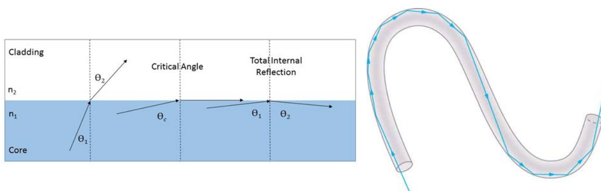
Figure 1.3: (Left) Refraction, critical angle and reflection at the interface of the core ( n_1 ) and the cladding ( n_2 ) of an optical fiber ( n_1 > n_2 ). Source fluxlight.com (Right) Example of light propagation inside an optical fiber Source lumenlearning.com .
