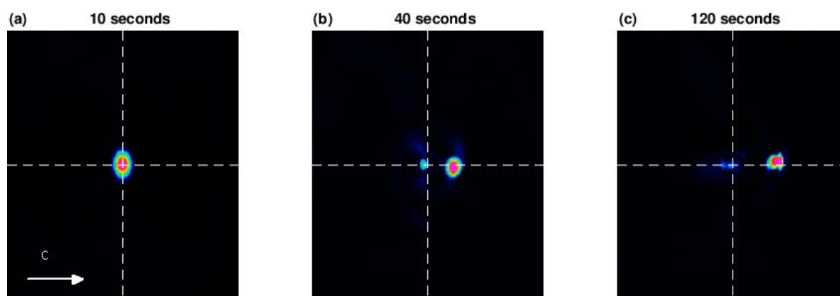
Figure 4.4: Transverse intensity distribution of a soliton over time propagating through a 2cm long SBN crystal and an externally applied voltage along the c-axis of the crystal of V = 2000V/cm . Injected Gaussian beam of 2\mu W , I_b = 35mW .
