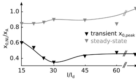
Figure 3.12: Influence of the background illumination on the transient and final self-focusing beam size x_0 normalized by the Airy beam main lobe size x_A . Extracted from [41]
