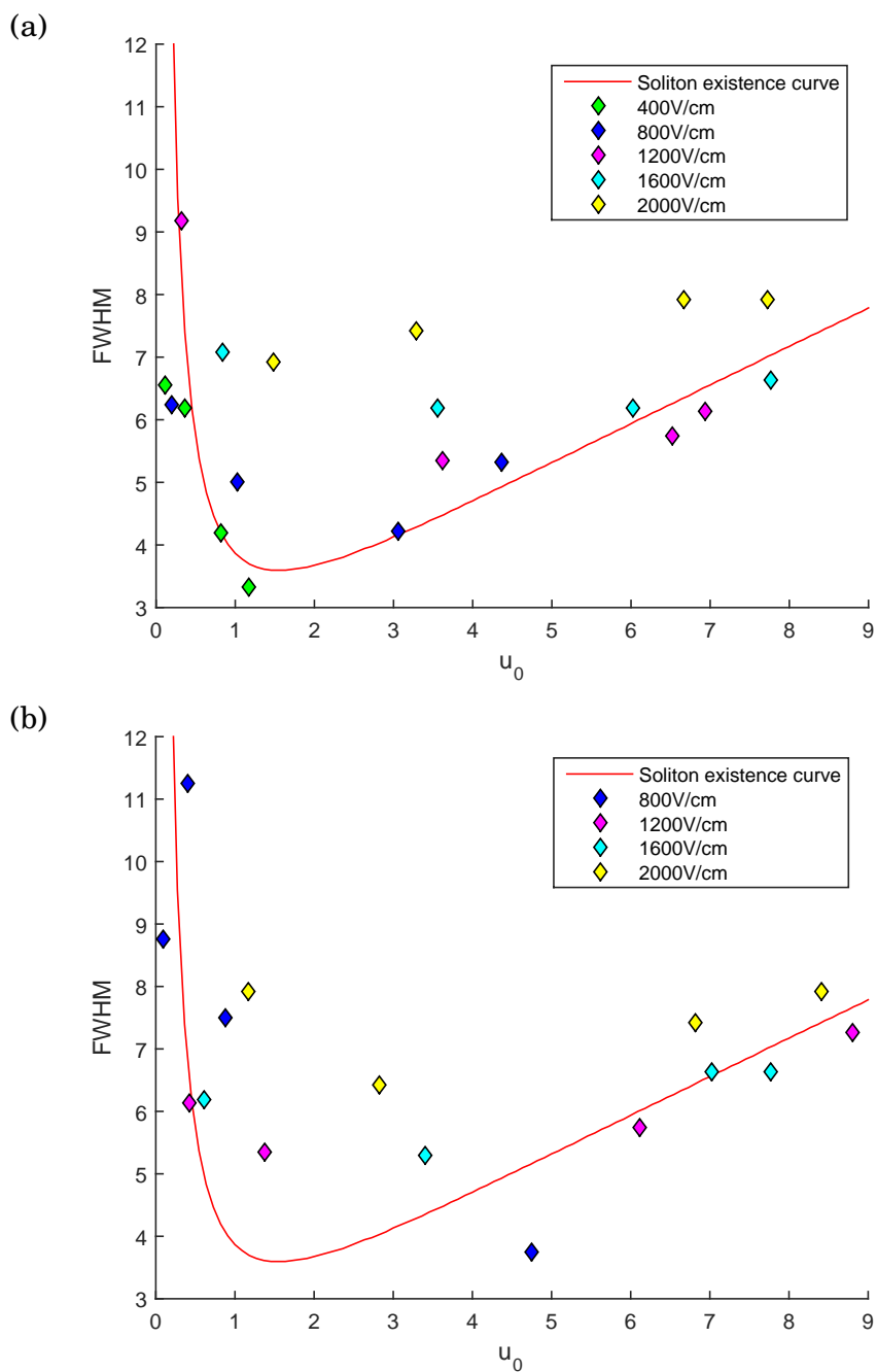
Figure 4.11: Theoretical soliton existence curve and experimental measures corresponding to Figure 4.7. (a) Airy beam of north-west acceleration. (b) Airy beam of south-east acceleration
