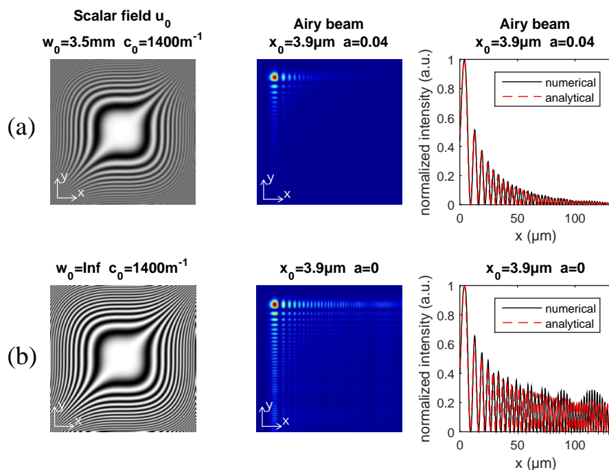
Figure 2.14: Numerical simulation of Airy beam generation showing border effects of the phase mask. (a) the phase mask of size 8.64\text{mm} * 8.64\text{mm} is illuminated by a Gaussian beam of waist w_0 = 3.5\text{mm} , and the numerical wave function matches with the analytic wave function. (b) the phase mask is illuminated by an infinitely large plane wave, and the numerical Airy beam function envelope shows oscillating patterns due to the square aperture of the SLM screen.
