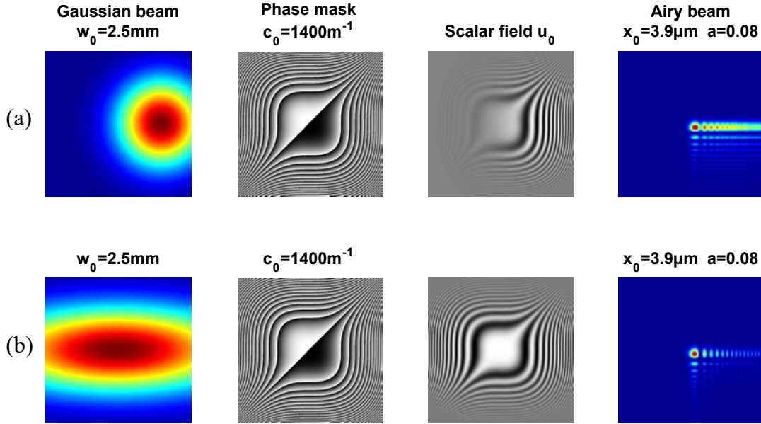
Figure 2.12: Numerical simulations of Airy beam with Gaussian misalignment (a) and Gaussian deformation (b). The resulting Airy beam has more lobes along the x-axis but only the case of misalignment presents additional blur. Columns are similar to figure 2.11.
