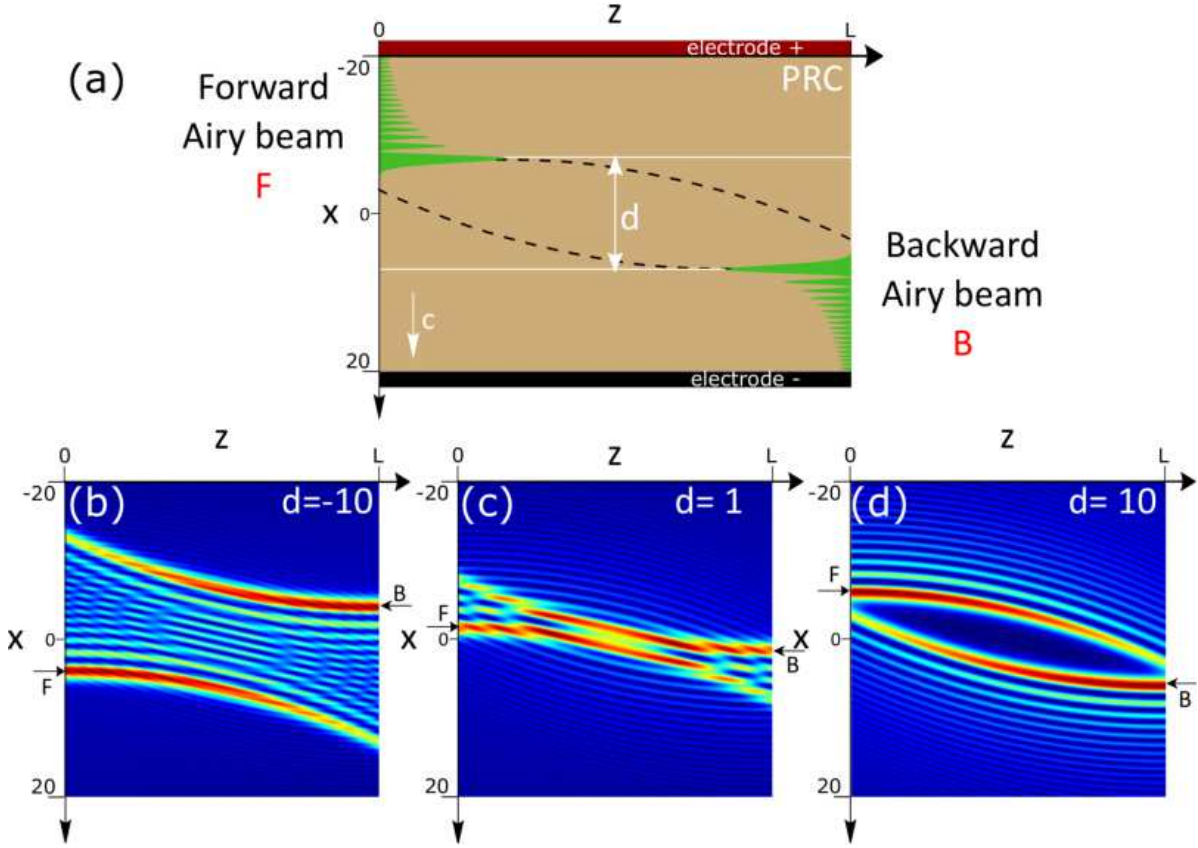
Figure 5.9: (a) Typical scheme of antisymmetric Airy beams' interaction in a PR crystal of length L . (b-c-d) Intensity distribution obtained for different values of shift d = -10 , d = 1 , d = 10 . ( F_0^2 = B_0^2 = 35 , x_0 = 10\mu m , a = 0.03 , L = 3 = 1.63cm .)
