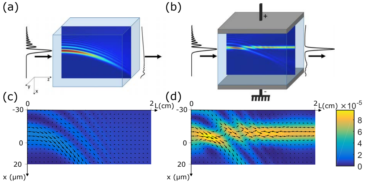
Figure 1.8: Propagation of a 1D Airy beam in a photorefractive crystal at steady state. (a) Linear propagation. (b) Nonlinear propagation in the presence of an external electric field leading to an OSS. (c), (d) Distribution of the refractive index change corresponding to (a) and (b) respectively. Arrows represent the Poynting vector.
