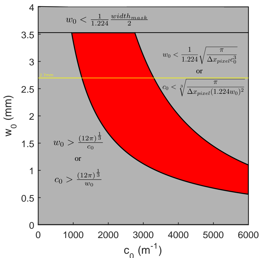
Figure 2.16: Plot representing in red the parameter range for the generation of analytical like Airy beams. w_0 is the Gaussian beam waist illuminating the phase mask and c_0 represents the phase shift within the mask.
