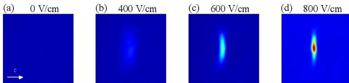
Figure 4.3: Experimental observation of soliton formation in a 2cm long SBN crystal for increasing applied electric voltages. Injected Gaussian beam of 2\mu W , I_b = 35mW .
