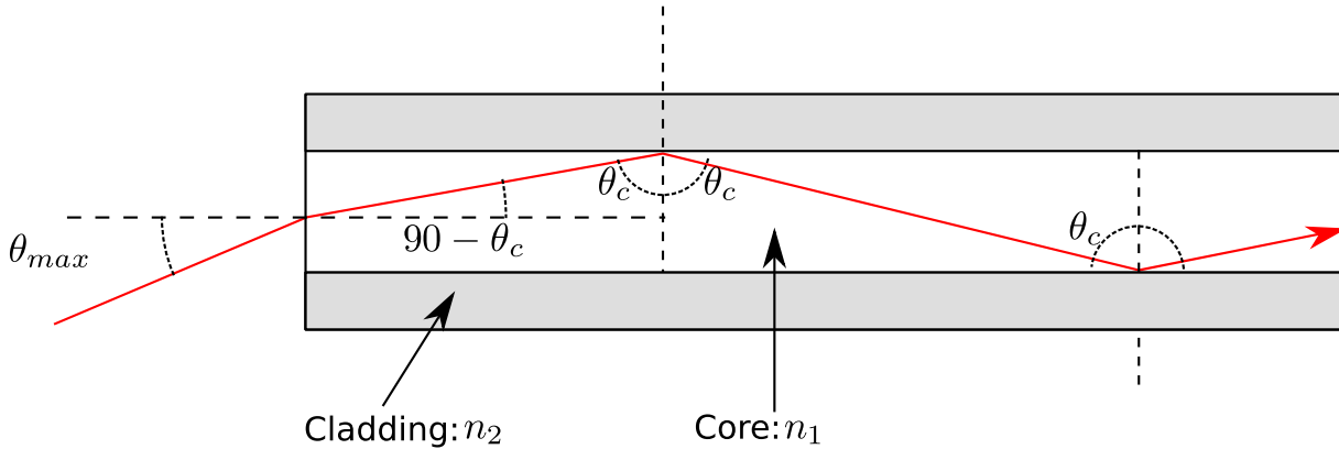
Figure 5.2: Schematic of waveguiding inside an optical fiber. The core refractive index n_1 is greater than the cladding refractive index n_2 causing total internal reflection.
