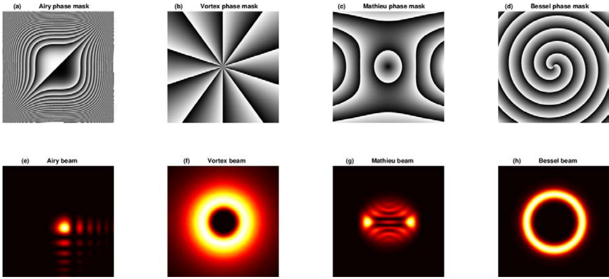
Figure 6.1: Phase masks (a-d) and corresponding beams (e-h) that can be generated using an SLM.
