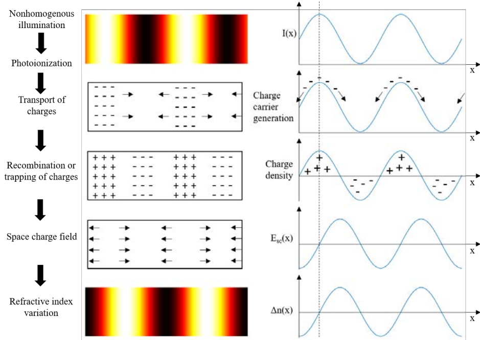
Figure 3.6: Schematic of the photorefractive effect in a crystal illuminated by light fringes.
