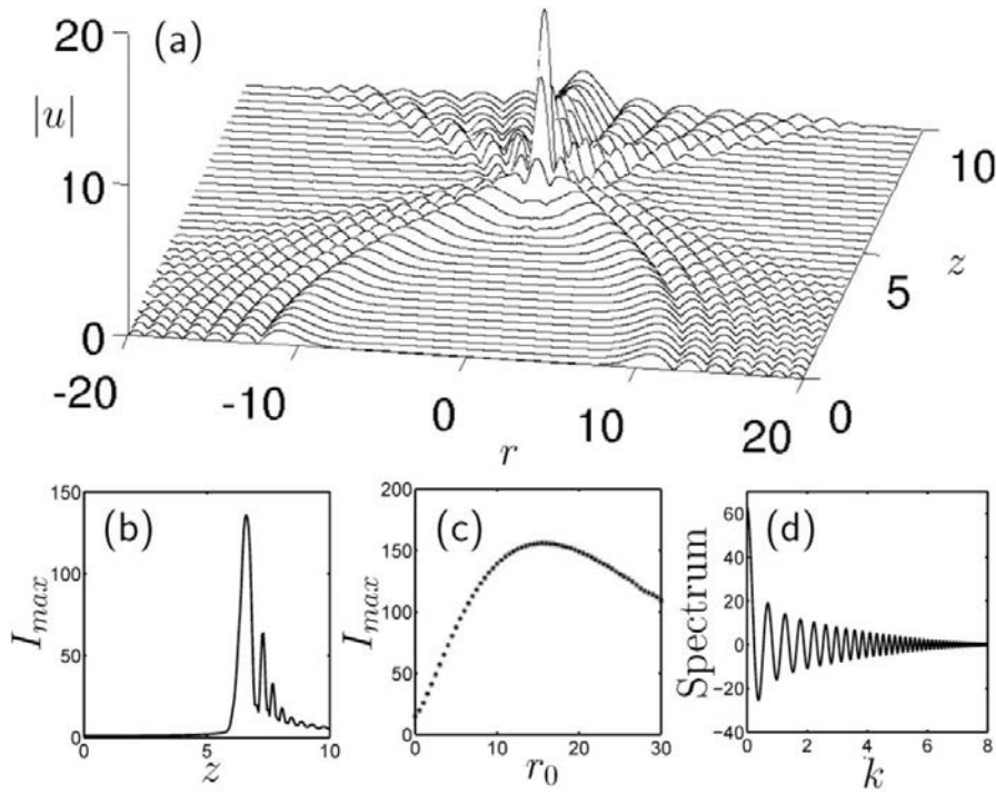
Figure 2.5: Dynamics of radially symmetric Airy beams for a = 0.05 , r is the normalized transverse scale, z is the normalized propagation scale, I is the intensity, r_0 is the initial radius of the main ring, and I_{max}(z = 0) = 1 . (a) Detailed plot of the central part of the propagation dynamics. (b) Maximum intensity as a function of z . (c) Maximum intensity that the Airy beam reaches during propagation for different values of the initial radius r_0 . (d) Hankel transform 1 of the initial condition. Extracted from [61]
