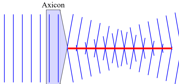
Figure 1.6: Bessel beam formed (in red) using an axicon to make two plane waves interfere.
