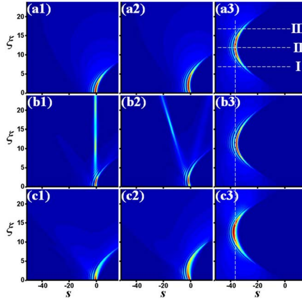
Figure 3.10: Propagation of an Airy beam under different conditions: (a) linear, (b) nonlinear self-focusing, and (c) nonlinear self-defocusing. The panels from left to right correspond to different shifting of the cubic phase mask. Extracted from [46]
