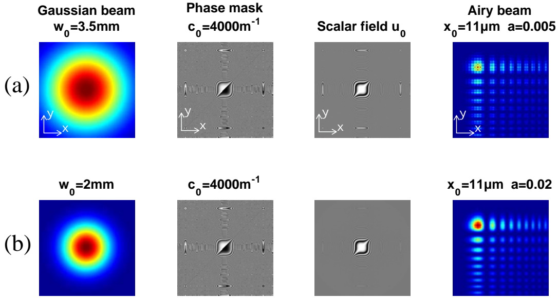
Figure 2.13: Numerical simulation of Airy beam aliasing. Columns are similar to figure 2.11. Simulation (a) shows an aliased Airy beam due to a high value c_0 = 4000 . Simulation (b) shows the aliasing is reduced by adapting the Gaussian beam size.
