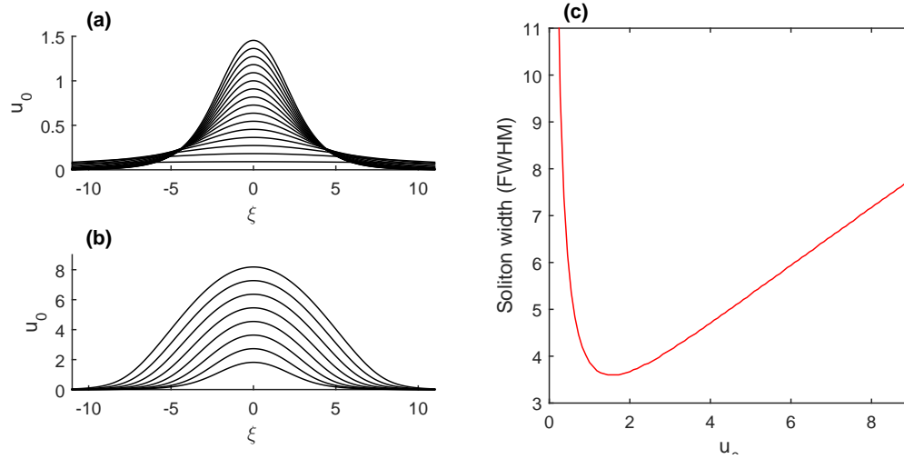
Figure 3.8: Photorefractive spatial soliton profiles for values of u_0 < 1.5 (a) and u_0 > 1.5 (b). Soliton existence curve (c), plots the corresponding width of the soliton in function of its peak amplitude in normalized transverse scale.
