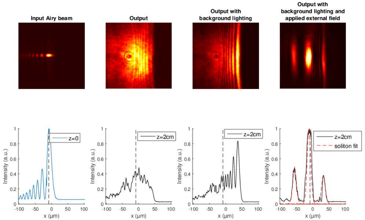
Figure 3.15: Input (a) and output (b-d) images of the transverse intensity profile of a 2\mu\text{W} Airy beam ( x_0 = 9.1\mu\text{m} a = 0.06 ), propagating through a 2cm SBN crystal. From (b) to (c) background lighting I_b = 35\text{mW} has been turned on. From (c) to (d) the externally applied field 800\text{V/cm} has been turned on. The second row is the transverse profile along the horizontal axis.
