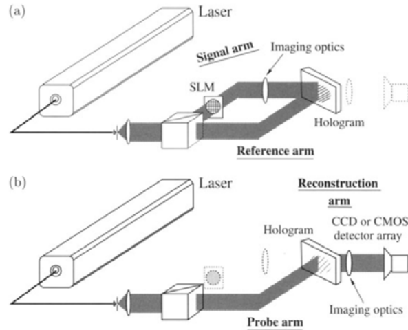
Figure 5.1: Holographic memory architecture: (a)storage arrangement; (b)retrieval arrangement. extracted from reference [120].
