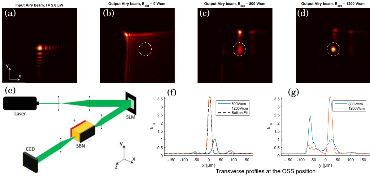
Figure 4.6: (a) Transverse intensity profile of the input Airy beam, 2.8 \mu\text{W} . (b-d) Transverse intensity profile of the output for different applied external field (b) E_{ext} = 0 \text{ V/cm} , (c) E_{ext} = 800 \text{ V/cm} , and (d) E_{ext} = 1200 \text{ V/cm} , the OSS position is represented by a dotted white circle. (e) Schematic of the experimental setup. (f-g) Intensity profile cross sections along the x and y axis at the OSS position
