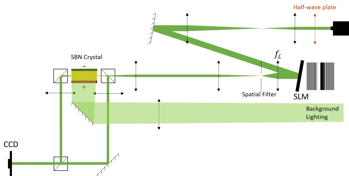
Figure 3.13: Schematic of the experimental setup
