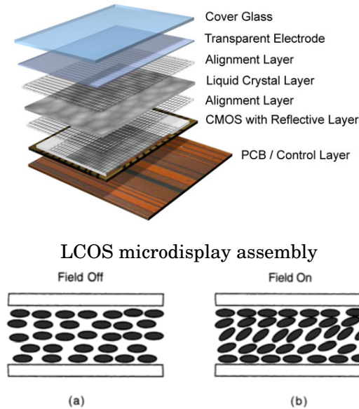
The alignment layer is treated to orient the liquid crystal molecules parallel to the surfaces, while the electric field tends to align the director perpendicular to the surfaces. (a) field below threshold value. (b) field above threshold value. Extracted from [74]
