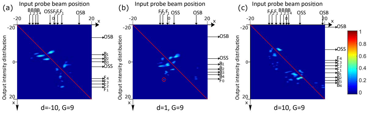
Figure 5.13: Intensity distribution of the probe beam at the output of the PR crystal for different input positions of the probe beam. ( \Gamma = 9 , F_0^2 = B_0^2 = 35 , L = 3 ). (a) Shift d = -10 . (b) Shift d = 1 . (c) Shift d = 10 .
