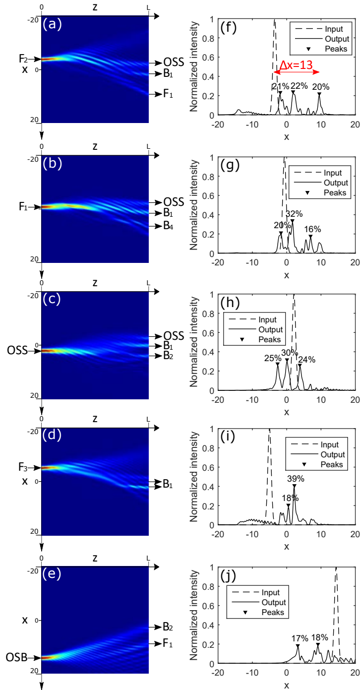
Figure 5.11: Linear probe beam propagation in the waveguide structure of figure 5.10 ( d = 1 , \Gamma = 9 , F_0^2 = B_0^2 = 35 , L = 33 = 1.63\text{cm} .) (a-e) Intensity distribution. (f-j) Transverse intensity profiles of a Gaussian beam guided from different input positions ( F_2 , F_1 , OSS , F_3 , OSB ) respectively.
