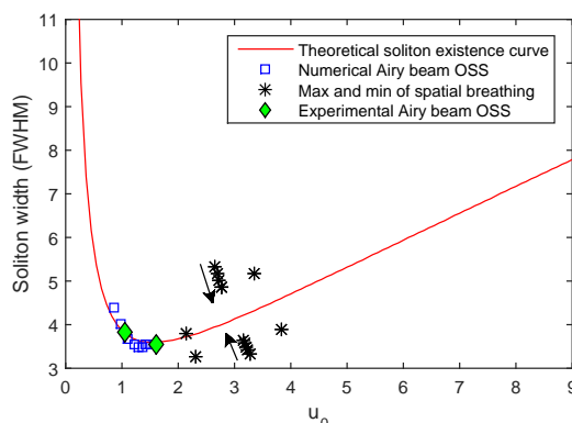
Figure 3.19: Full width at half maximum (FWHM) in dimensionless units ( \xi ) in function of soliton amplitude. In red the theoretical curve from Ref. [98], in blue squares the Airy beam OSS at 2 cm propagation from our numerical model, in black stars the maximum and minimum of the observed spatial breathing and the arrows show the evolution when propagating greater distances. In green diamonds, the experimental OSS observed in Fig. 1.
