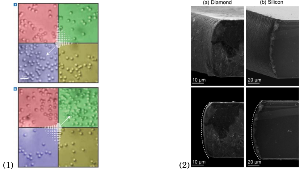
The micrometre-scale 'snowblower' at work. The white arrow indicates the deflection of the beam's main spot during propagation. (b) Subsequently to the micrograph shown in (a) the Airy beam was rotated by 180°. Extracted from reference [56]
