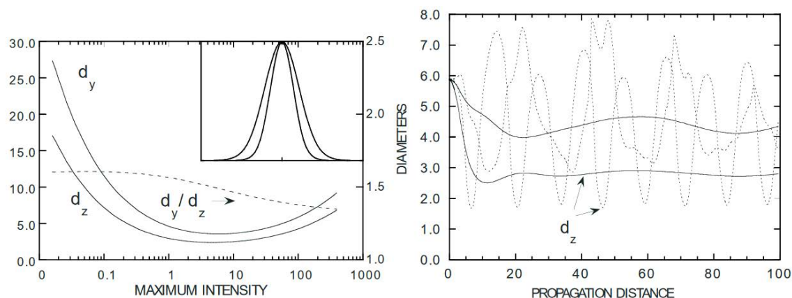
Figure 4.1: (Left) Both transverse diameters of the elliptic soliton solution (solid) and their ratio vs. its maximum intensity (dashed). The insert shows the soliton intensity cross-sections for maximum intensity equal to 5. (Right) Evolution of diameters of an initially round Gaussian beam for low intensity (solid) and high intensity (dashed curves). Extracted from reference [109].
