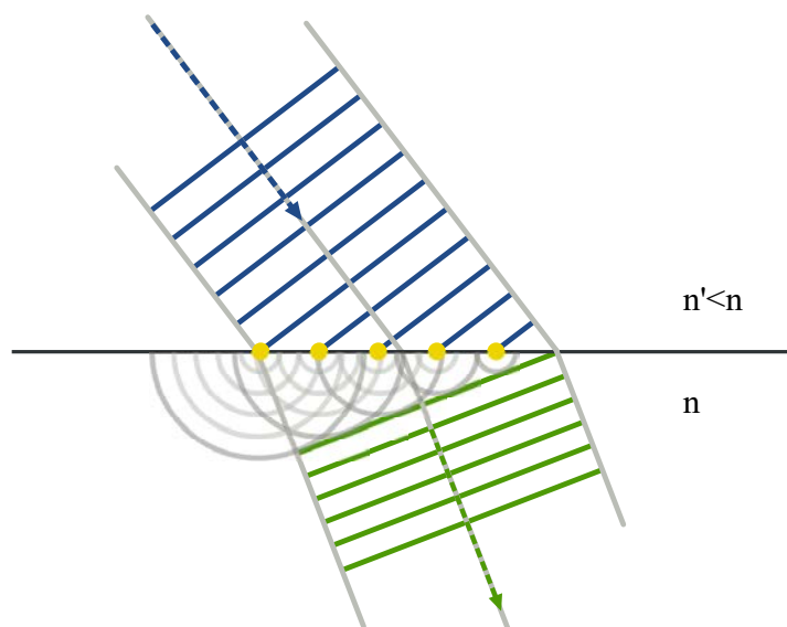
Figure 1.5: Refraction using the Huygens-Fresnel principle. Source wikipedia
