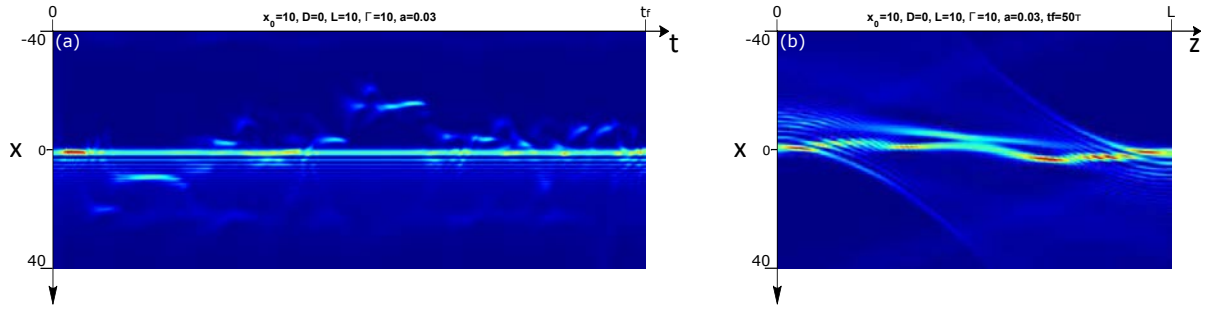
Figure 6.2: Instability of numerical counterpropagating Airy beam interactions. (a) Temporal evolution of the transverse output intensity profile at z = L . (b) Undergoing nonlinear interaction of two counterpropagating Airy beams in an externally biased photorefractive crystal at t = t_f = 50\tau . \tau is the relaxation time of the crystal
