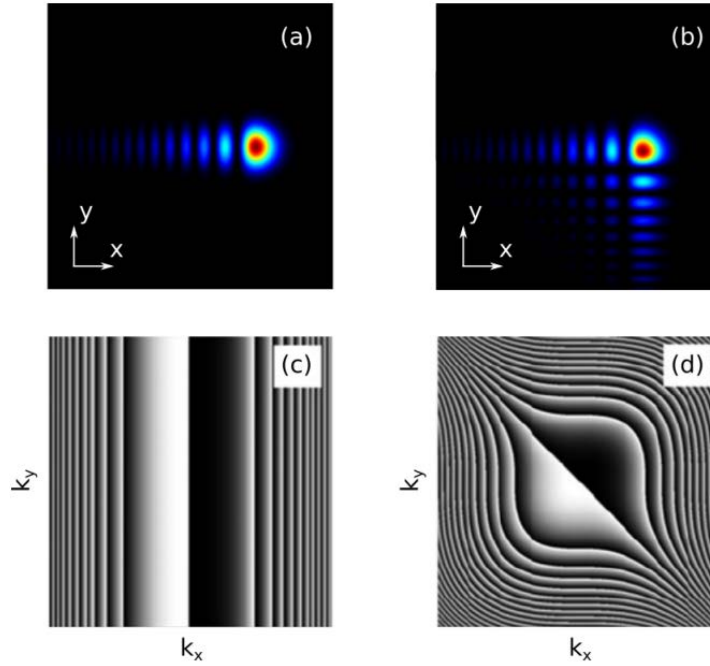
Figure 2.7: Transverse intensity distribution of a (a) 1 D-Airy beam and (b) 2 D-Airy beam. Phase mask on the spatial light modulator for the generation of a (c) 1 D-Airy beam and (d) 2 D-Airy beam. [14]
