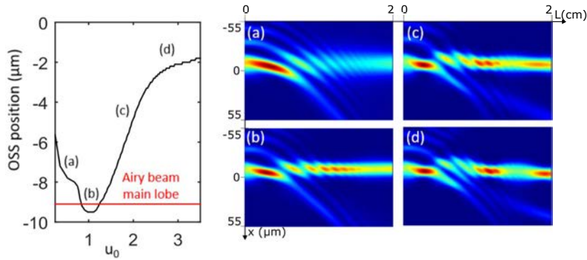
Figure 3.18: Position of the Airy beam OSS as function of OSS maximum amplitude for \Gamma = 10 , F_0 = 1 to 7.5 or u_0 = 0.25 to 3.5 , x_0 = 10\mu\text{m} , a = 0.1 and t_f = 20\tau_0 . (a to d) Corresponding numerical simulation inside the crystal for (a) u_0 = 0.5 , (b) u_0 = 1.04 , (c) u_0 = 1.9 , (d) u_0 = 2.9
