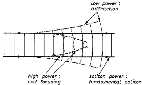
Figure 3.3: Propagation of a limited plane wave in nonlinear Kerr medium. At low power the beam spreads under diffraction. At high power the beam self-focuses. At soliton power the beam propagates without variation of the transverse dimension. Extracted from [33].
