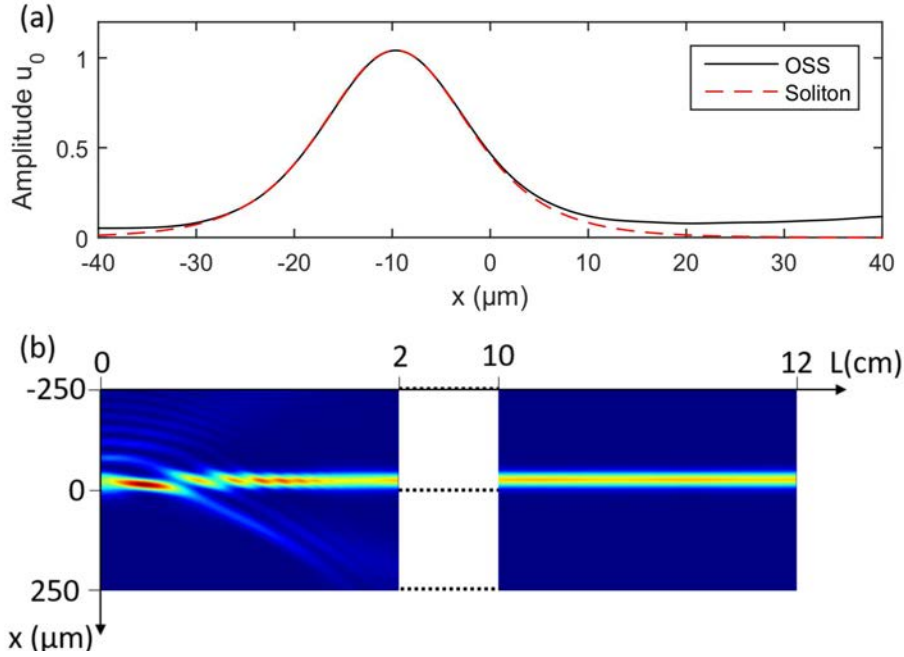
Figure 3.17: (a) Numerical profile of the Airy beam OSS in Fig. 3.16(b) and corresponding theoretical soliton at L=2\text{cm} . (b) Propagation of the OSS over long distances at steady state. ( \Gamma = 10 , F_0 = 1.95 , x_0 = 10\mu\text{m} , a = 0.1 , u_0 = 1.04 ).
