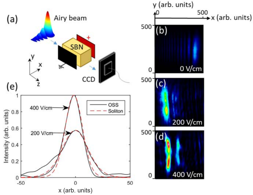
Figure 3.14: (a) Schematic of the experimental setup: 1D Airy beam propagating in a 2 cm long SBN crystal. ( x_0 = 10 , a = 0,1 ) (b) Observation of the Airy beam at the crystal output face on camera with no electric field E_{ext} applied. (c)-(d) Observation of the OSS at the crystal output face on the CCD camera ( E_{ext} = V/l = 200 and 400 V/cm). (e) Corresponding experimental Airy beam OSS profile extracted from the camera and theoretical classic soliton fit ( E_{ext} = 200 or 400 V/cm and P_A = 50\mu W ).
