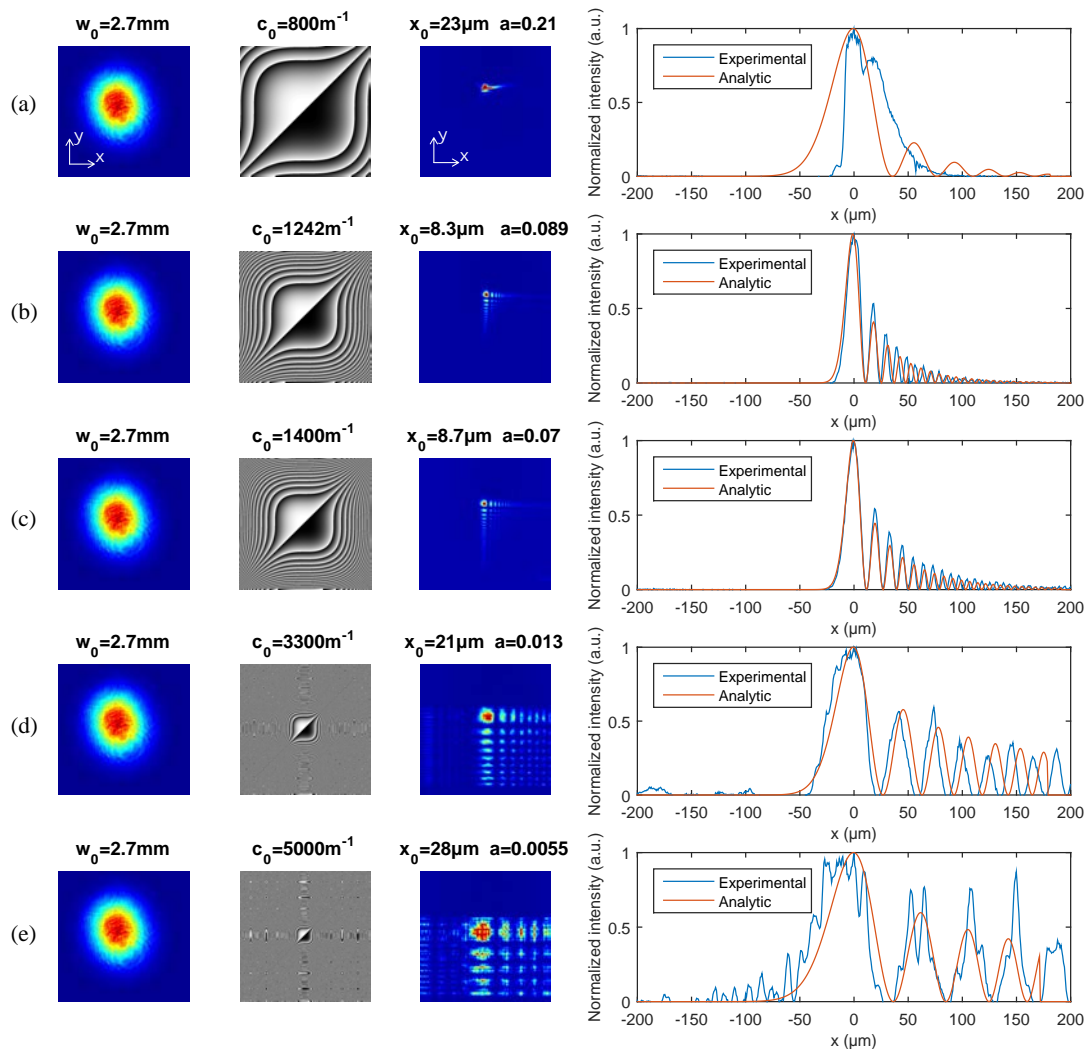
Figure 2.17: Experimental generation of Airy beams with w_0 = 2.7\text{mm} . The phase mask's phase shift c_0 is increased one row to the next. (a) phase shift too low to yield an Airy beam with secondary lobes. (b) limit case scenario when the Airy beam's secondary lobes are significantly formed (deduced from equation 2.20). (c) example of an Airy beam generated in the red parameter range from figure 2.16. (d) limit case scenario when the Airy beam starts showing aliasing (deduced from equation 2.16). (e) high phase shift leads to aliasing of the Airy beam. First column : Gaussian beam illuminating the phase mask. Second column : Illuminated phase mask on the SLM. Third column : Transverse intensity profile of the resulting Airy beam in the image focal plane of the Fourier transform lens. Fourth column : Intensity profile of the experimental Airy beam along the horizontal x-axis vs the Airy beam analytic profile.
