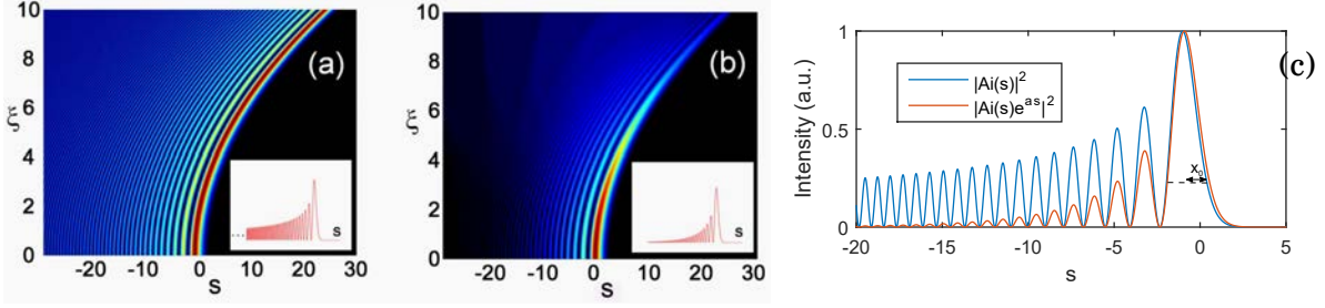
Figure 2.1: Propagation dynamics of (a) a diffraction-free infinite-power Airy beam and (b) a finite-power Airy beam when a=0.05 . Extracted from [14] (c) Transverse profile of the infinite-power Airy beam and finite-power Airy beam at \xi = 0
