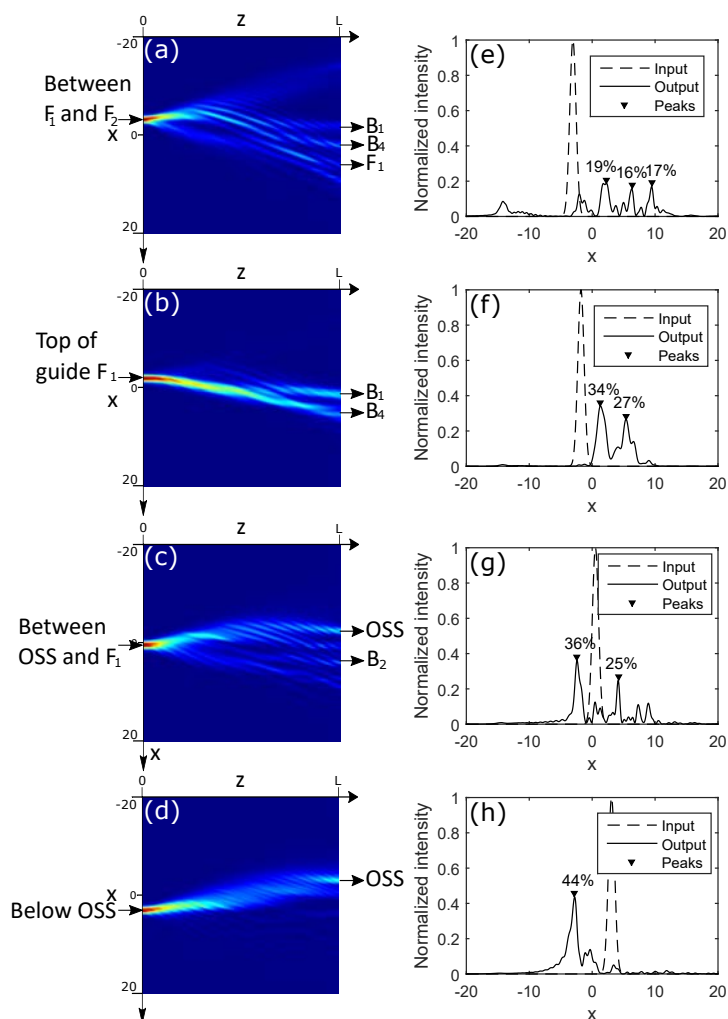
Figure 5.12: Linear probe beam propagation in the waveguide structure of figure 5.10 ( d = 1 , \Gamma = 9 , F_0^2 = B_0^2 = 35 , L = 3 )
