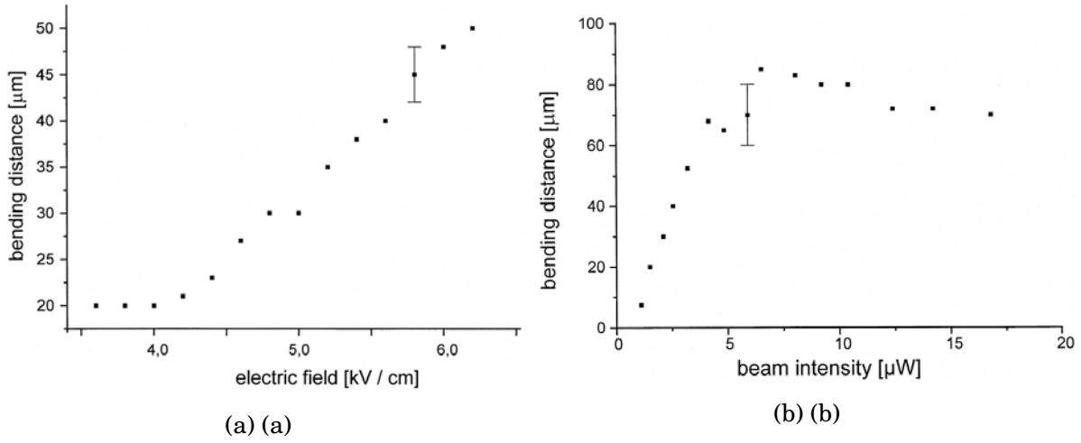
Figure 4.2: (a) Beam bending distance depending on the applied electric field. For a beam intensity of 8.1\mu W , diameter 17\mu m and I/I_b = 1 . (b) Beam bending distance depending on the the beam intensity. Applied electric field of 5.4kV/cm , beam diameter 12\mu m . Extracted from [118].
