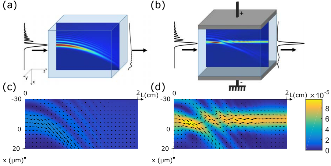
Figure 3.16: Propagation of a 1D-Airy beam in a 2cm long photorefractive crystal at steady state. (a) Linear propagation ( \Gamma = 0 ). (b) Nonlinear propagation in presence of an external electric field leading to an OSS. ( \Gamma = 10 , F_0 = 1.95 , x_0 = 10\mu\text{m} , a = 0.1 ). (c-d) Distribution of the refractive index change versus x and z at steady state. Arrows represent the Poynting vector. (c) \Gamma = 3 . (d) \Gamma = 10 .
