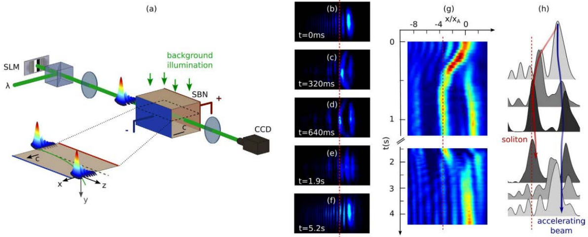
Figure 3.11: (a) Experimental setup. (b-f) Transverse intensity profile of the output beam under nonlinear focusing conditions for increasing times. (g) 1D intensity profile along time. (h) Top-view sketch of the accelerating beam interacting with the off-shooting soliton, superimposed with their intensity profiles along time. Extracted from [41]
