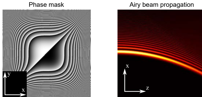
Figure 1.7: (Left) Phase mask on the SLM that creates an Airy beam after diffraction. (Right) Airy beam propagating along the z -axis.
