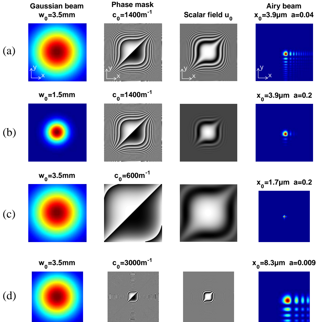
Figure 2.11: Numerical simulations of Airy beam generation. First column: Gaussian beam illuminating the phase mask. Second column: Illuminated phase mask on the SLM. Third column: Scalar field in the object plane of the Fourier transform lens. Fourth column: Transverse intensity profile of the resulting Airy beam in the image focal plane of the Fourier transform lens.
