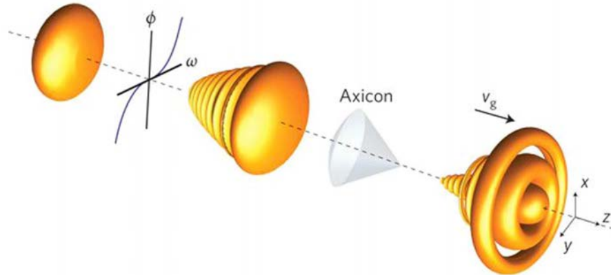
Figure 2.6: Experimental generation of an Airy-Bessel light bullet. 3D plots comprising iso-intensity contour plots of Gaussian-Gaussian (initial profile), Airy-Gaussian (after adding a large cubic spectral phase) and Airy-Bessel (after the axicon) wave packets. \phi , \omega , and v_g are phase, optical frequency and group velocity respectively. Extracted from [18]
