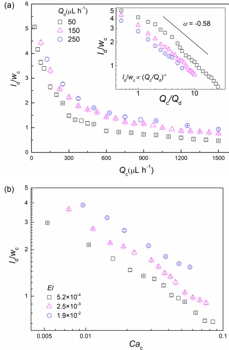
Fig. 3-11 Effect of various factors on the dimensionless size of droplets. (a) The two-phase flow rates, inset: effects of the two-phase flow rate ratio, 100 K PEO solution, El = 5.2 \times 10^{-4} . (b) The capillary number of the continuous phase, Q_d = 100 \mu\text{L} \cdot \text{h}^{-1} .
