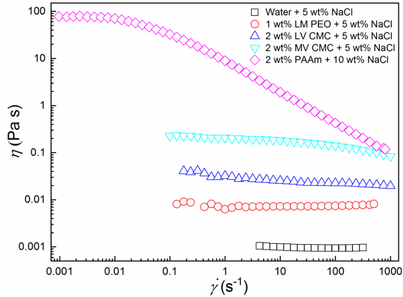
Fig. 6-3 Rheological properties of all the working liquids.
