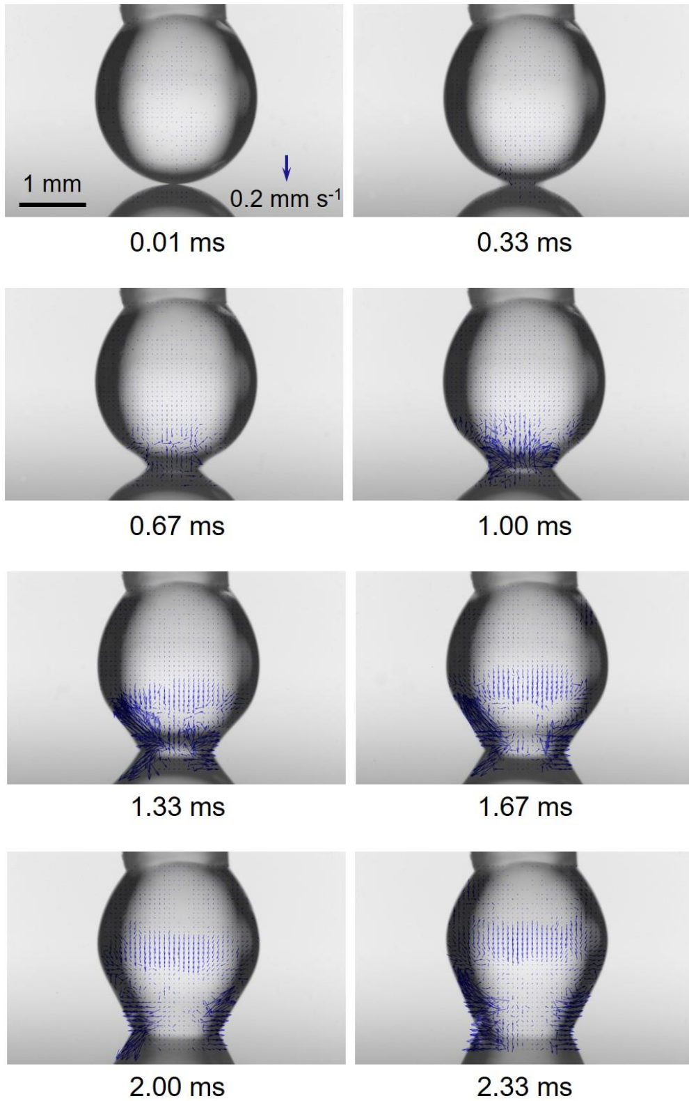
Fig. 6-10 Velocity fields in the drop during the initial contact and spreading. 2 wt% LV CMC solution with 5 wt% NaCl. v_0 = 0.29 \text{ mm}\cdot\text{s}^{-1} . 3000 velocity fields per second. The scale bars for length and velocity indicate 1 mm and 0.2 \text{ mm}\cdot\text{s}^{-1} , respectively.
