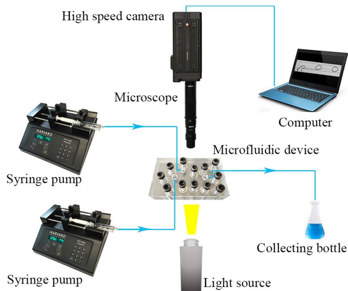
Fig. 3-1 Scheme of the experimental setup.
