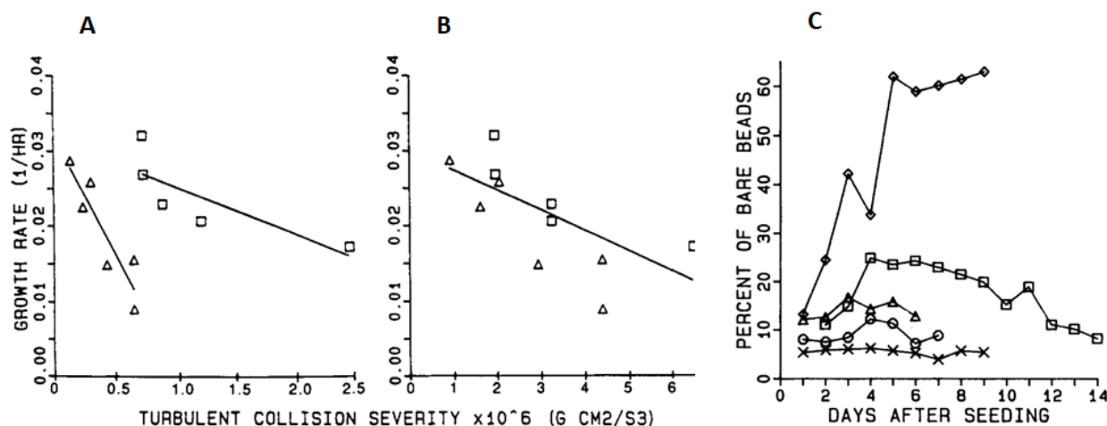
Figure 1.31 – Effects of turbulent collision severity on BEK cell growth rates (A) and (B) in function of the impeller diameter ( \square ) 6cm impeller ( \Delta ) 4cm impellers. (C) Impact of the impeller speed on the empty microcarriers concentration ( \times ) 45 rpm, ( \square ) 60 rpm, ( \circ ) 80 rpm, ( \Delta ) 100 rpm, ( \diamond ) 136 rpm (Cherry and Papoustakis [174]).
