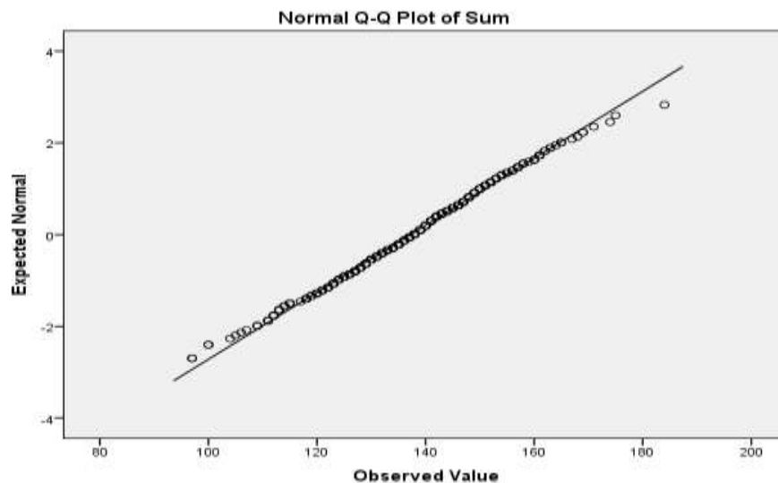
Figure 4: Normal plot Q-Q of our sample generated by SPSS 22.0
