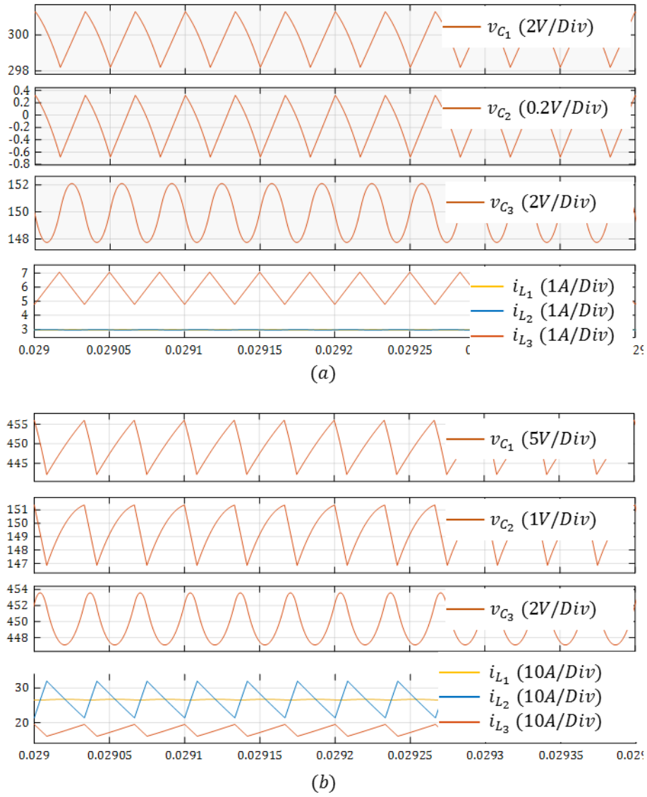
Fig. 2.25 QZSBC (a) and SEPIC (b) waveforms with the capacitance and inductance values specified in Table 2.5 and the operating point in Table 2.3 ( V_o = 450V ).
