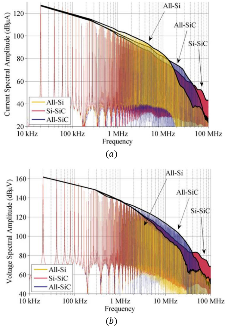
Fig. 1.18 Current (a) and voltage (b) spectra across the switching devices for the double pulse test performed in [50].
