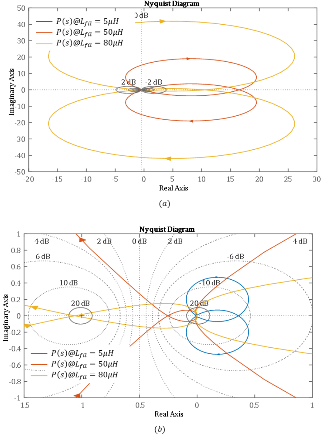
Fig. 4.26 Study of the Nyquist plot of \chi(s) (a), zoomed around the point (-1,0) in (b), by varying L_{fil} ( V_{in} = 270V , V_o = 350V , C_o = 20\mu F , L = 500\mu H , P_o = 3000W , f_s = 20kHz , w_e = 12.5k \frac{rad}{s} , C_{fil} = 20\mu F , DCR_{fil} = 0.01 \Omega , L_{fil} = 5\mu H, 50\mu H, 80\mu H ).
