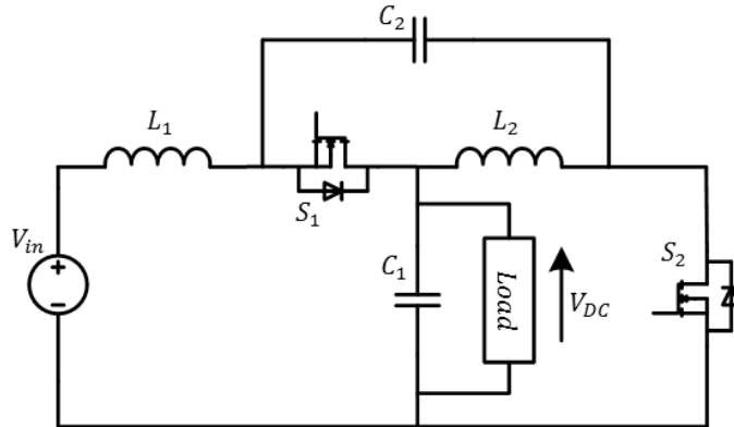
Fig. 2.6 Alternative version of Quasi Z-Source converter [71].
