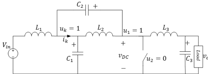
Fig. 2.14 QZSBC configuration during Conduction Mode ( u_1 = 1, u_2 = 0, u_K = \overline{u_1} \cdot \overline{u_2} = 1 ).
