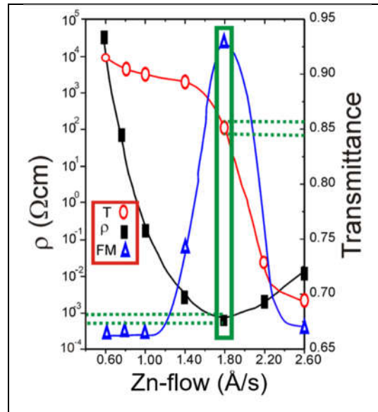
Figure 4.5 Variation of resistivity, transmittance (at 700 nm) and figure of merit (quality criteria \Phi_{Tp} ) of ZnO thin films as a function of Zn-flow.
