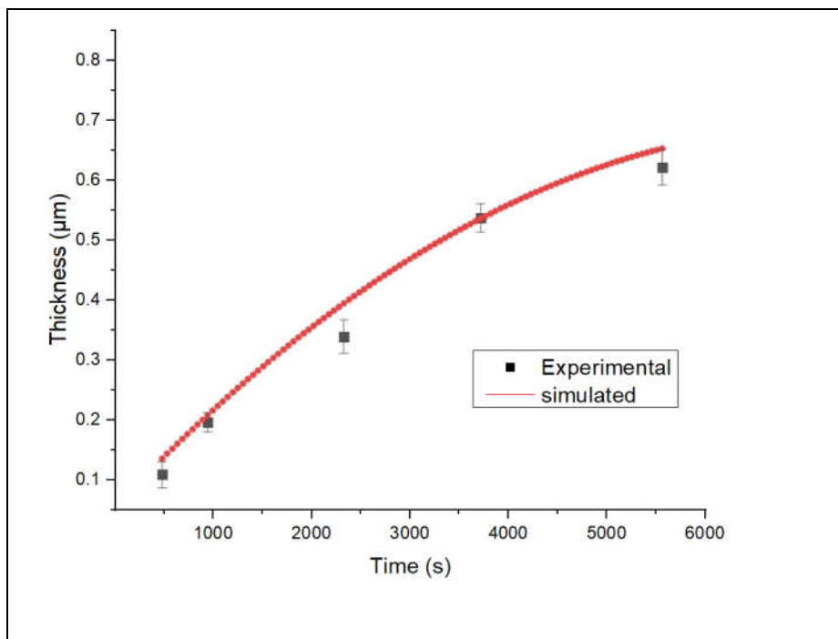
Figure 3.7 Comparison of the experimental measurements of the thickness of ZnO films prepared by reactive evaporation in dependence of the deposition time, with their corresponding simulated values.
