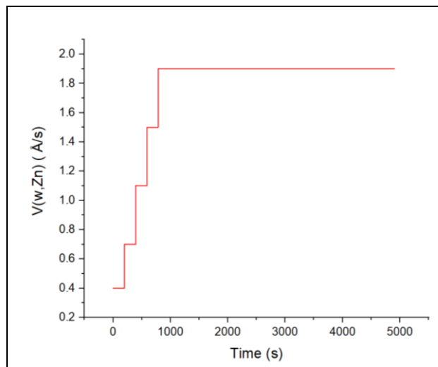
(c) Nu = 25
