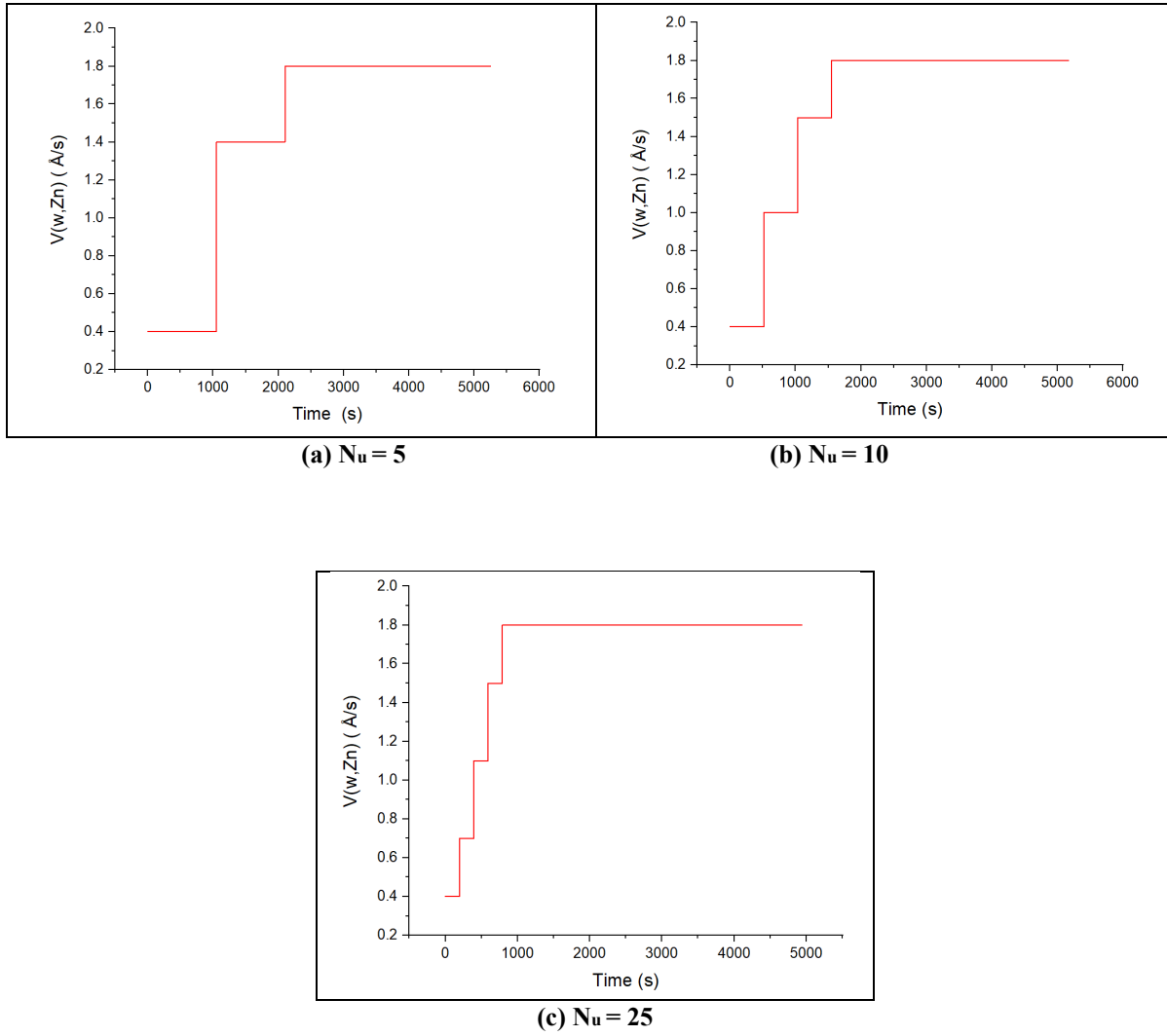
Figure 5.3 Optimal Zn flow profile for the time minimization
