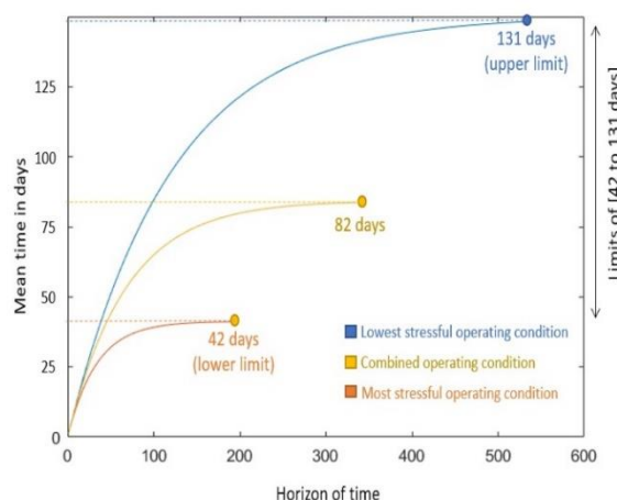
Fig. 40: Mean time RUL for known inputs
