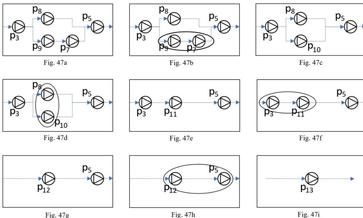
Fig. 47: The steps of model constructions
