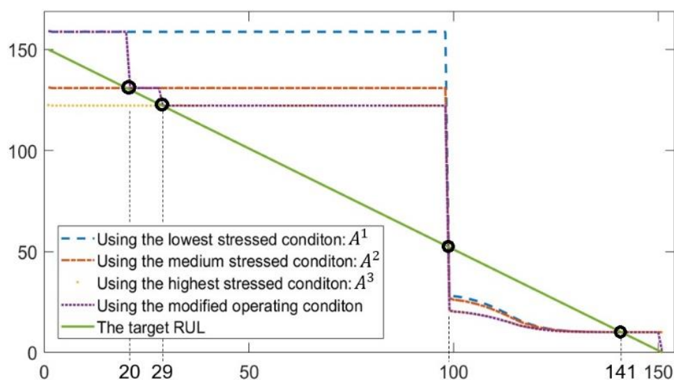
Fig. 28: Online RUL matching with the target RUL [y-axis: days; x-axis: days]
