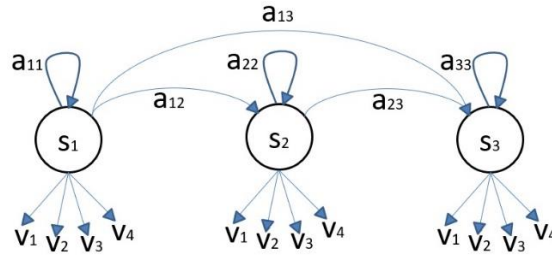
Fig. 8: Left-right model HMM model
