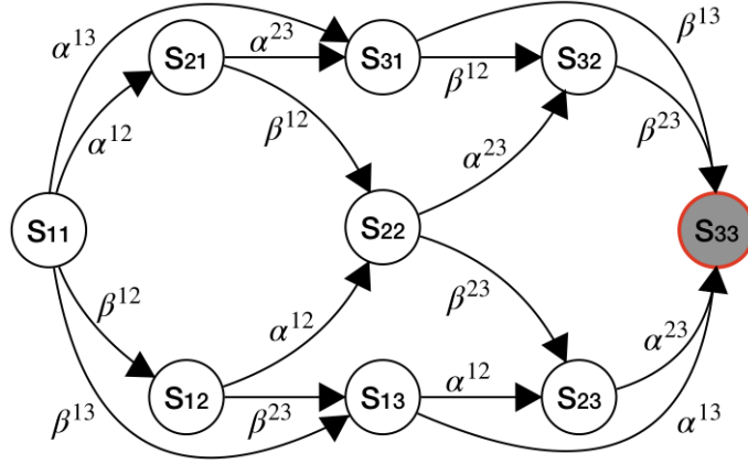
Fig. 45. Transition graph of two parallel components
