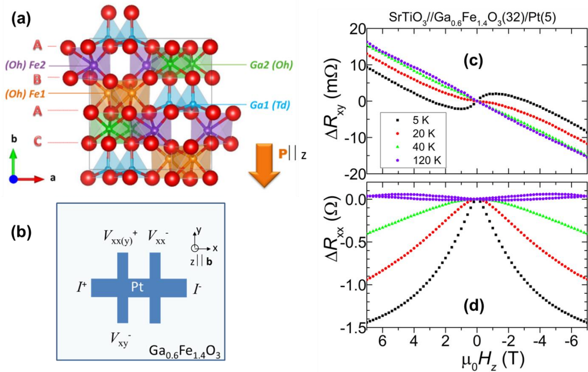
Figure VI.3 Towards confirmation of the magneto-electric effect in \text{Ga}_{2-x}\text{Fe}_x\text{O}_3 . (a) The \text{Pc}21n orthorhombic structure of \text{Ga}_{2-x}\text{Fe}_x\text{O}_3 (GFO), showing the double hexagonal close-packed stacking of oxygens (ABAC), and the 3 octahedral and 1 tetrahedral cationic sites. The orange arrow stands for the electrical polarization \mathbf{P} , which is perpendicular to the film plane. Adapted from [258]. (b) Schematic of a double-cross Hall bar of Pt patterned on top of GFO thin film. The connections for the longitudinal and transverse electrical measurements are shown together with the coordinate axis used. (c) Transversal and (d) longitudinal resistivities as function of perpendicular magnetic field. The variation of longitudinal resistance as function of H_x and H_y has the same behavior as for H_z . We can observe in both R_{xx} and R_{xy} that a transition occurs below 120 K
