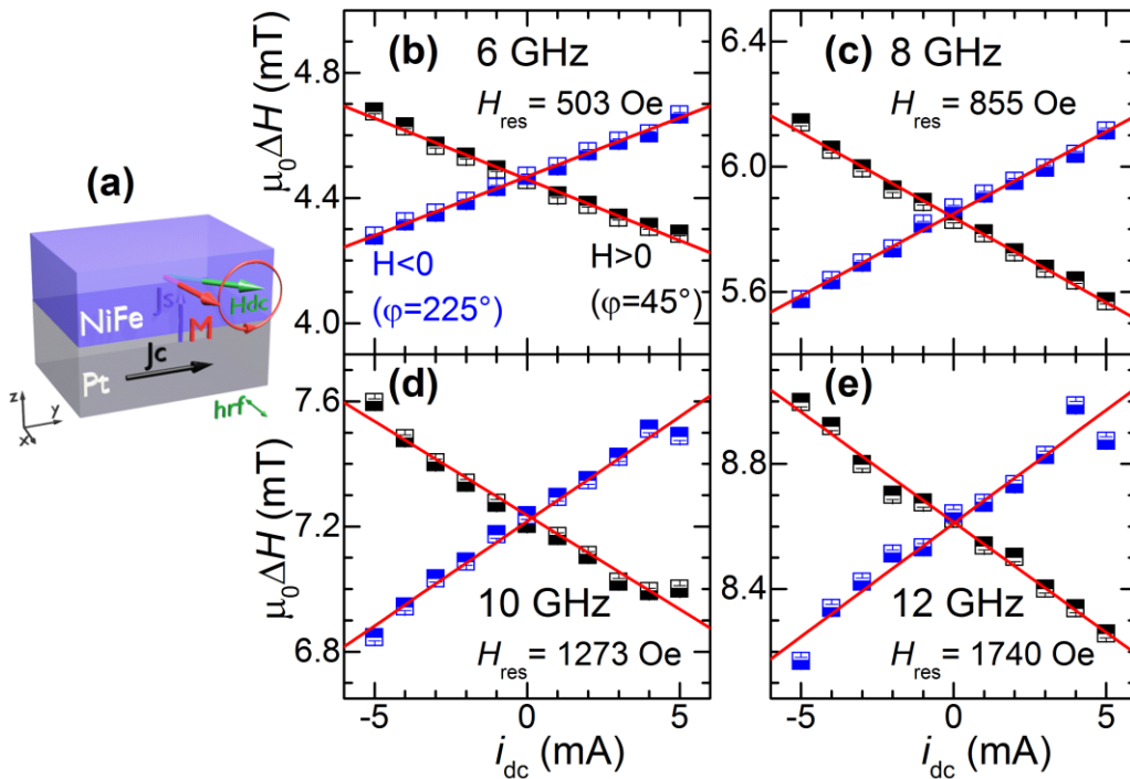
Figure IV.5 Variation of NiFe linewidth vs. total current I_{\text{dc}} added in the STFM experiment at different frequencies between 6 and 12 GHz. The analysis, eq. (4.10), yield an average
