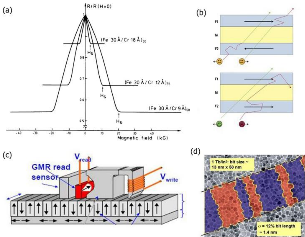
Figure I.1 Discovery of GMR. (a) GMR in Fe/Cr(001) multilayers [1]. With the current definition of the magnetoresistance ratio, MR=100 \times [R_{AP} - R_P/R_P] , MR= 85\% for the Fe 3 nm/Cr 0.9 nm multilayers. GMR effects were observed at about the same time with Fe/Cr/Fe trilayers by the team of Peter Grünberg at Jülich [2]. (b) Schematic of the mechanism of the GMR. In the parallel magnetic configuration (bottom), the electrons of one of the spin directions can go easily through all the magnetic layers and the short-circuit through this channel leads to a small resistance. In the antiparallel configuration (top), the electrons of each channel are slowed down every second magnetic layer and the resistance is high. (c) Schematic of a GMR write/read head in HDD. (d) Example of magnetic bits on the HDDs of today. Taken from ref. [9].
