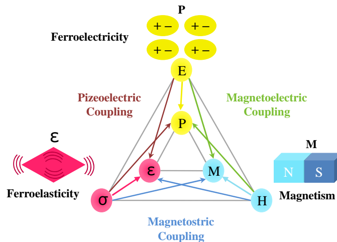
Figure 1.6: The electric field E , magnetic field H , and stress \sigma control of the electric polarization P , magnetization M , and strain sv , respectively. In a ferroic material, P , M , or e are spontaneously formed to produce ferromagnetism, ferroelectricity, or ferroelasticity, respectively. In a multiferroic, the coexistence of at least two ferroic forms of ordering cause additional interactions. In a magnetoelectric multiferroic, a magnetic field can control P or an electric field can control M [2].
