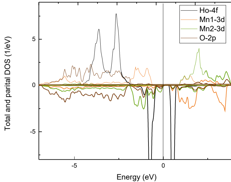
Figure 4.4: Total and partial density of states obtained within (GGA þ Spin Orbit)
