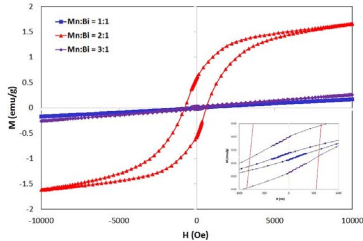
Figure 1.5: Hysteresis loop of MnBi particles under pressure n the ratio Mn:Bi = 1:1, 2:1 and 3:1 after sintering at 1000 řC
