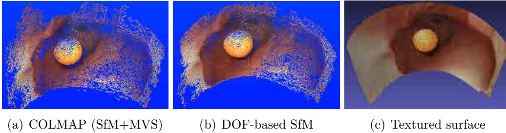
Figure 5.3: Internal phantom reconstruction results (same viewpoint as in Fig. 5.1(b)). (a) Point cloud given by COLMAP [SF16]. (b) Point cloud obtained with the proposed SfM method. (c) Textured triangle mesh obtained with the point cloud in (b).
