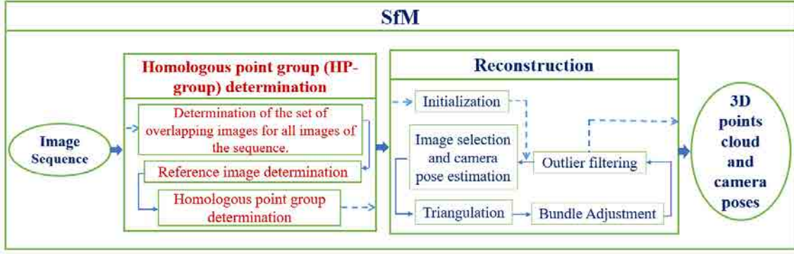
Figure 3.13: DOF-based SfM pipeline used in this thesis.
