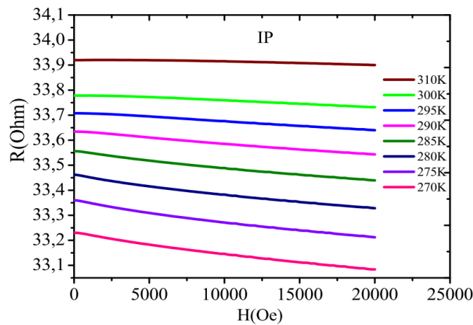
FIGURE V.2: Variation of the electrical resistivity as a function of the magnetic field, for I=2\text{mA} .
