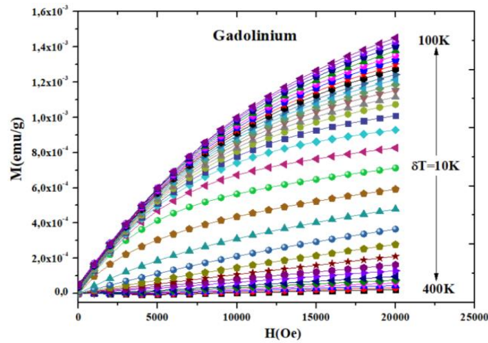
FIGURE V.4: Magnetic isotherms of the studied Gd_{100nm} thin film as a function of the applied magnetic field from 0 to 20 kOe with a sweeping rate of 250 Oe/s.
