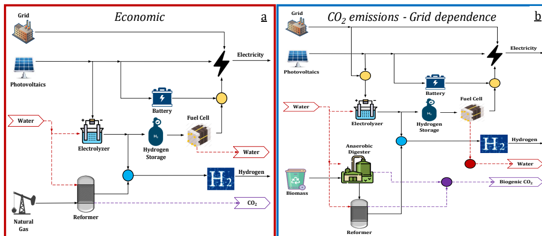
Figure 4-2: Optimal energy system configuration for the extreme points of the Pareto fronts. Objective function (a) total annualized cost, and (b) \text{CO}_2 emissions and grid dependence.
