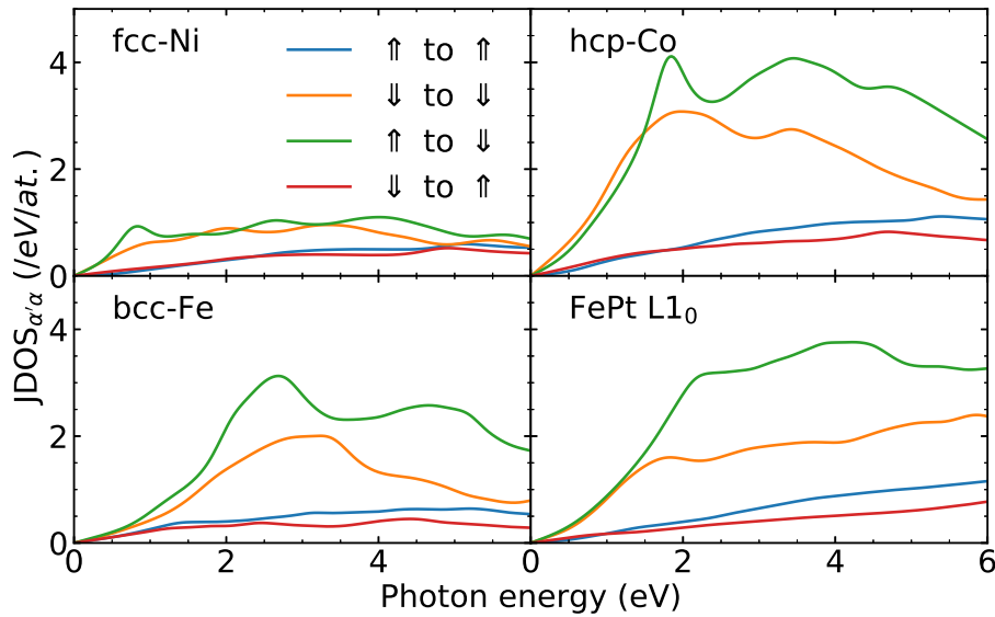
FIGURE 6.3: Joint density of states of fcc-Ni, hcp-Co, bcc-Fe and FePt L1 0 broken down into the different initial and final magnetic states involved, as defined in Eq. 6.6.
