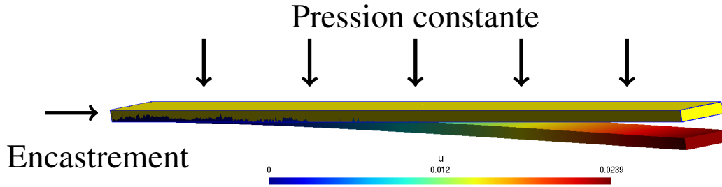
FIGURE A.1 – PoutreEncastrée
