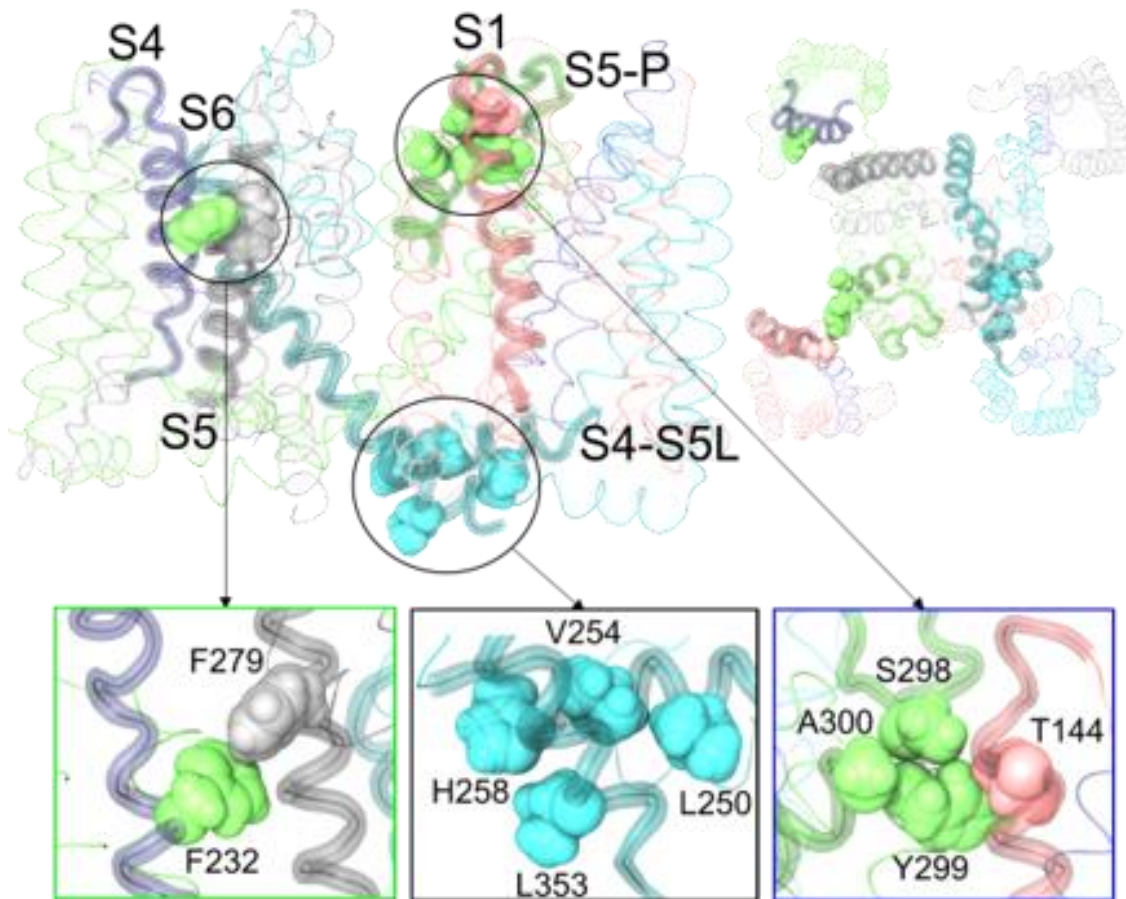
Figure III.1.1.3: State-dependent pairs of Kv7.1 neighbor residues.
