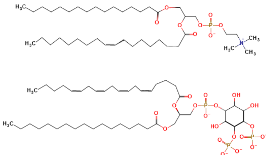
Figure II.2.2.1: Membrane lipids used in MD systems.
