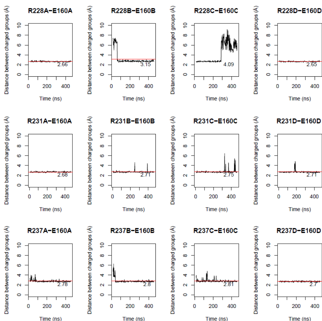
Figure III.1.1.2: State-dependent VSD salt-bridges involving E160 (E1) in Kv7.1 MD simulations. This figure displays the graphs of interatomic distances involving E1 and S4 gating charges R228 (upper panel) in RC model, R231 in IO model, and R237 in AO model, all throughout their respective MD trajectories. On each graph, the distance average value is shown in the lower right corner, and depicted as a red line when the value is below the threshold of 3.5 Å.
