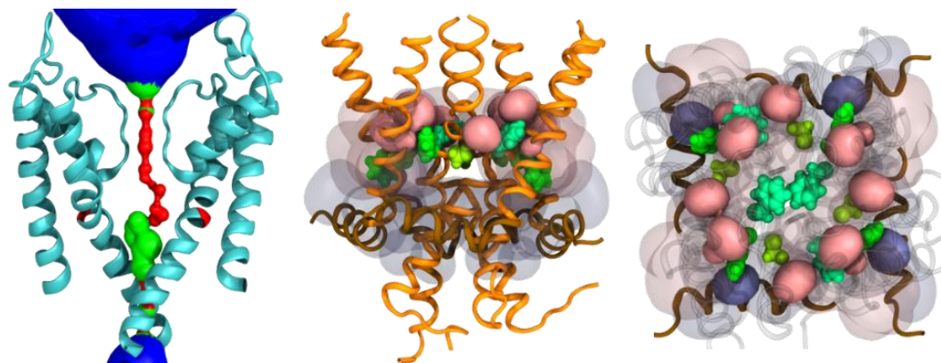
Figure III.2.3.3: Conformations of F340 side chains in KCNQ1 EM structure and Kv7.1 AC model.
