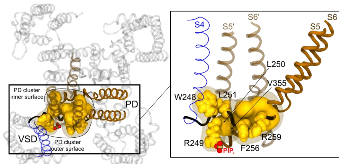
Figure III.2.1.10: Structural mapping of PD cluster residues in Kv7.1 3D model
