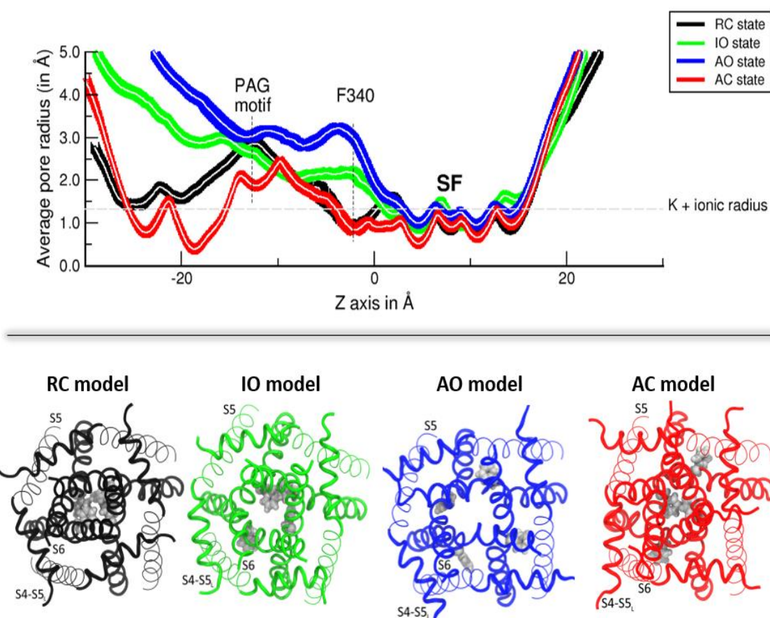
Figure III.1.3.4: Pore size calculations of Kv7.1 models.
