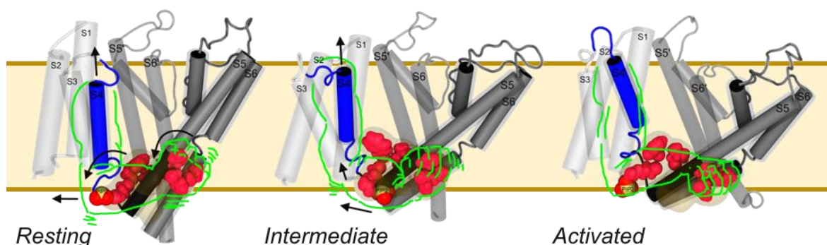
Figure III.2.1.14: Hand-and-elbow model for Kv7.1 state-dependent VSD-PD coupling mechanism. This figure shows a cartoon representation of Kv7.1 transmembrane segments, including one entire subunit on the foreground with the VSD (transparent light gray) S4 (blue), S4-S5L (black) and PD segments (solid gray) along with the PD segments of an adjacent subunit (transparent gray). The “elbow” residues W248 R249 L251 and the “hand” residues H258 L262 I346 L347 are depicted in pink spheres. PIP 2 phosphate groups, in state independent interaction with the elbow (R249) is shown in red spheres. The entire arm that models the whole conformational changes is drawn in green. The motions of both the elbow and the arm during RC-IO and IO-AO transitions are depicted by black arrows.
