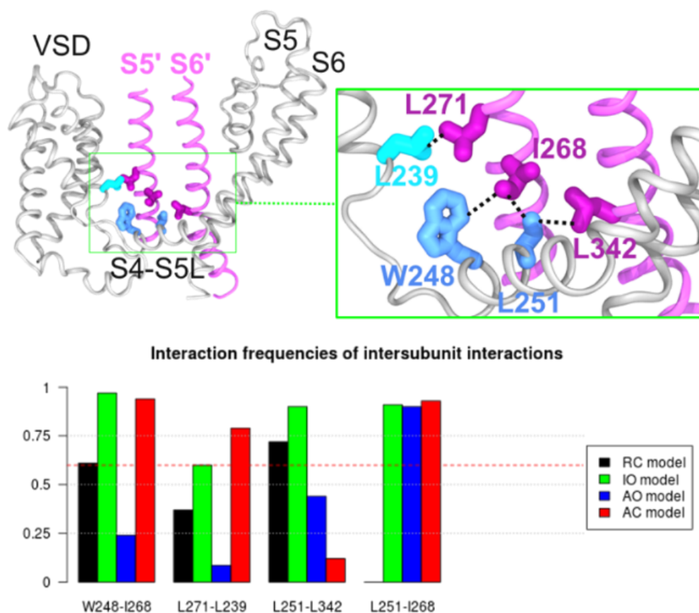
Figure III.2.1.8: MD simulation results shows the crucial interactions for Kv7.1 IO state coupling. The top panel shows cartoon representations of the IO state of Kv7.1. An entire subunit in the foreground (in gray) as well as S5 and S6 segments of an adjacent subunit (in purple) are shown with insets of enlarged structures of the boxed area. The color code is similar as Figure III.2.1.7. The bottom panel displays the interaction frequencies of IO model specific residue pairs including four S4c residues and thirteen S4-S5 L and PD residues throughout the MD trajectories obtained for Kv7.1 RC, IO, AO, and AC models. L251 and I268 show high interaction frequencies in both IO and AO. The frequency threshold of 0.6 is marked by a red dashed line.
