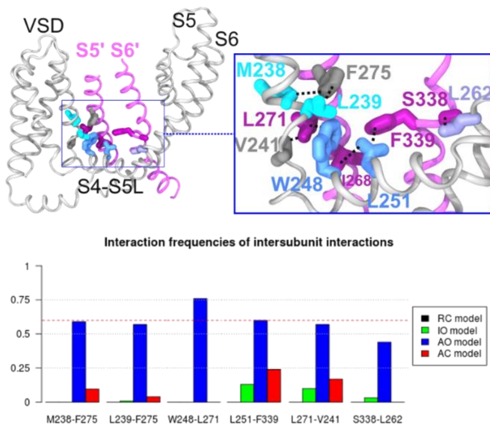
Figure III.2.1.7: MD simulation results show the crucial interactions for the Kv7.1 AO state coupling. The top panel shows cartoon representations of the AO state of Kv7.1. An entire subunit in the foreground (in gray) as well as S5 and S6 segments of an adjacent subunit (in purple) are shown with insets of enlarged structures of the boxed area. Residues in S4c are colored in cyan, S4-S5L in blue, and S5 and S6 segments from the adjacent subunit in purple. Residues V241 and F275, which are identified in MD simulations as possibly involved in sidechain interactions, but mutations do not alter AO states are colored in dark grey. Each pair of residues is represented by a black dashed line connecting their respective sidechains. The bottom panel displays the interaction frequencies of AO model specific residue pairs including four S4c residues and thirteen S4-S5L and PD residues throughout the MD trajectories obtained for Kv7.1 RC, IO, AO, and AC models. The frequency threshold of 0.6 is marked by a red dashed line.
