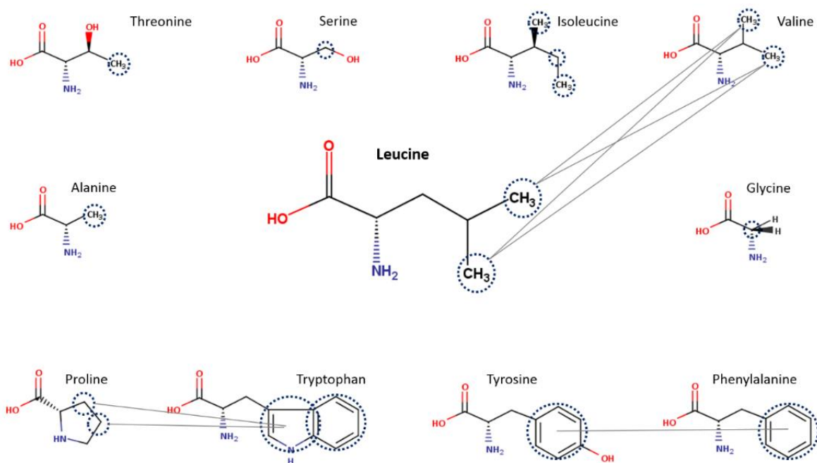
Figure II.3.3: Computed distances for assessing hydrophobic interactions.
