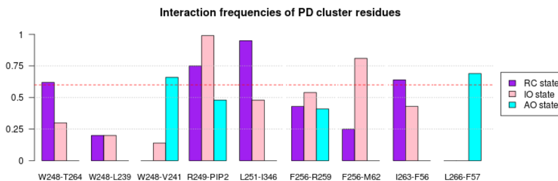
Figure III.2.2.2: Interactions of PD cluster outer surface residues in IKs models.
