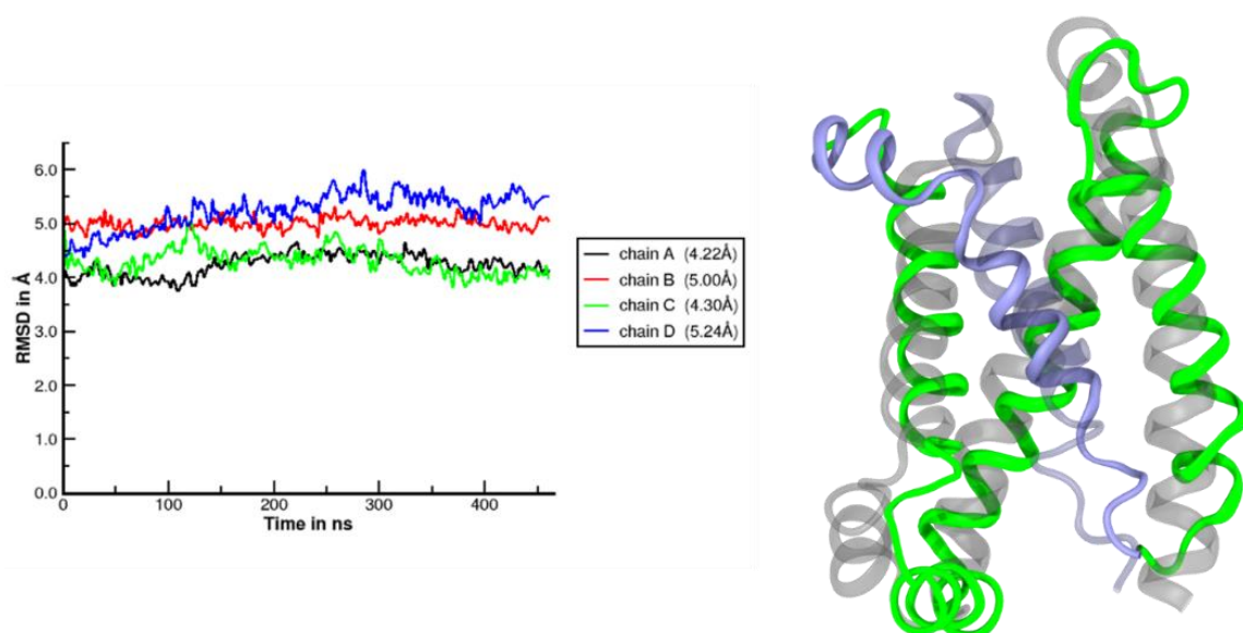
Figure III.1.4.3: Comparison of Kv7.1 IO model with NMR structure of human Kv7.1 VSD.
