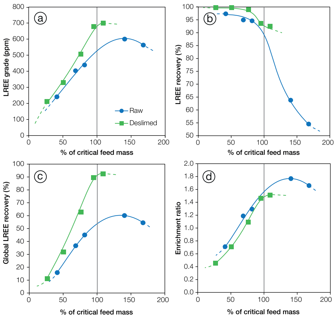
Figure 6.7: Effect of bowl saturation on Falcon UF separation performance on raw and deslimed -53\ \mu\text{m} residue samples. (a) Effect of bowl saturation on concentrate LREE grade. (b) Effect of bowl saturation on final LREE recovery. (c) Evolution of global LREE recovery with increasing bowl saturation. (d) Effect of bowl saturation on LREE enrichment ratio.
