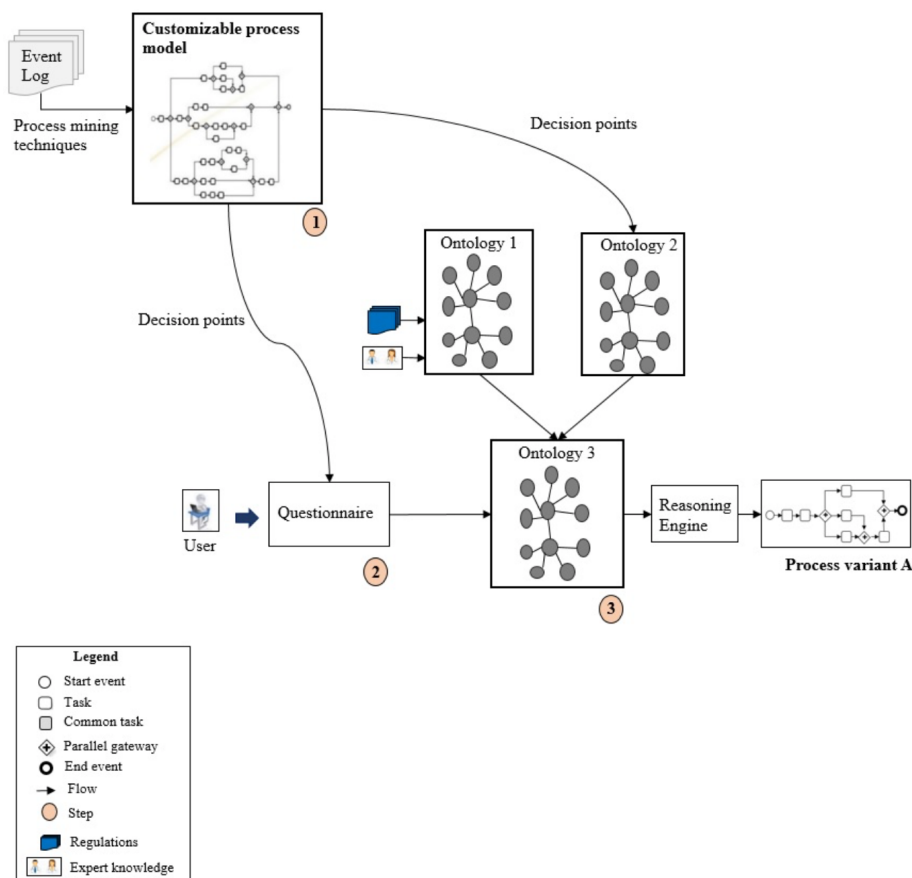
Figure 12 Framework for customize process variants from [15]
