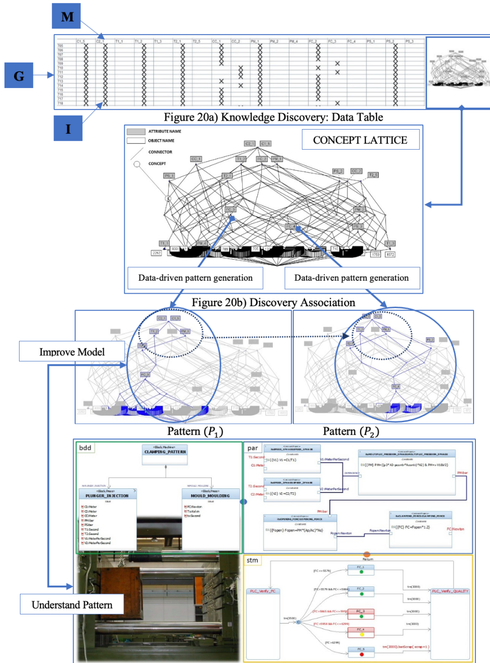
Figure 20c) SysML Model: Knowledge Extraction
