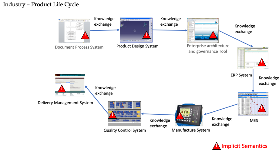
Figure 2 – Implicit semantics and semantic interoperability problem
