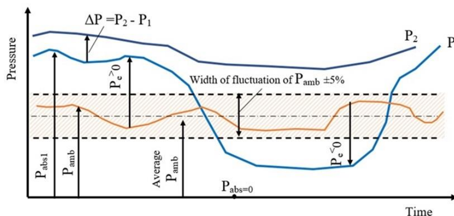
Figure H-1: Types of pressure: absolute pressure, gauge pressure, differential pressure (adapted from en.wika.com).
