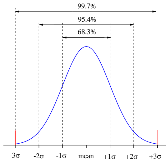
Figure 4.4: Gaussian distribution law
