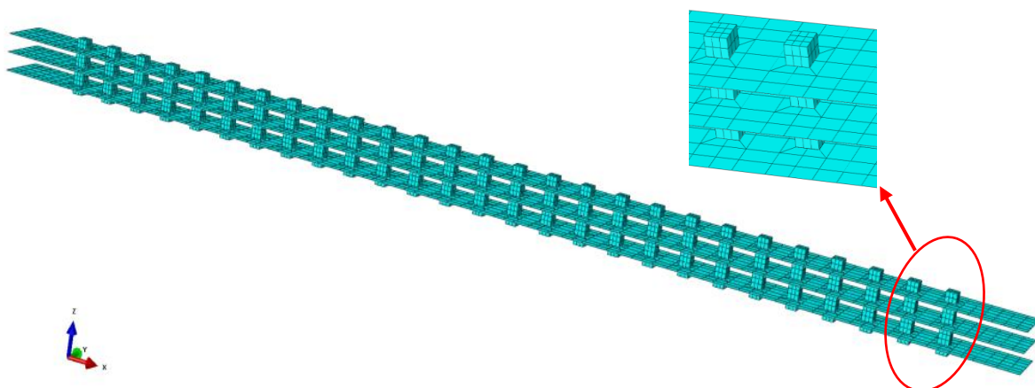
Figure 3.37: Proposed simplified FE model of AFLB
