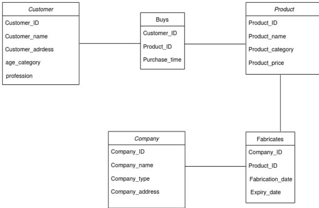
FIGURE 1.1 – Relational database
