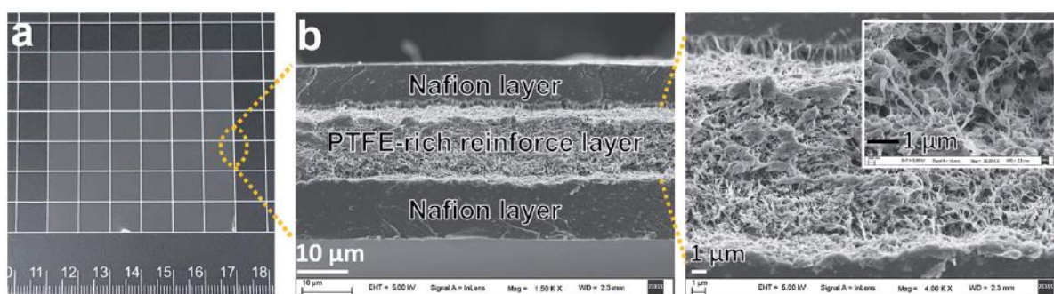
Figure 1.8 - (a) photograph and (b) cross-section SEM micrographs with different magnification of the Nafion™ XL morphology [91].
