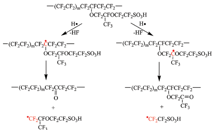
Figure 1.35 – Mechanism of H • radical attack on Nafion™ main chain and side chain suggested by Danilczuk et al. [258].
