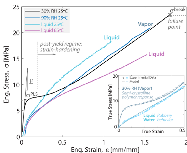
Figure 1.17 - Stress-strain response of a Nafion™ membrane under various environmental conditions. The inset illustrates the mechanical behavior of the membrane as a function of the nature of the sorbed water [77].
