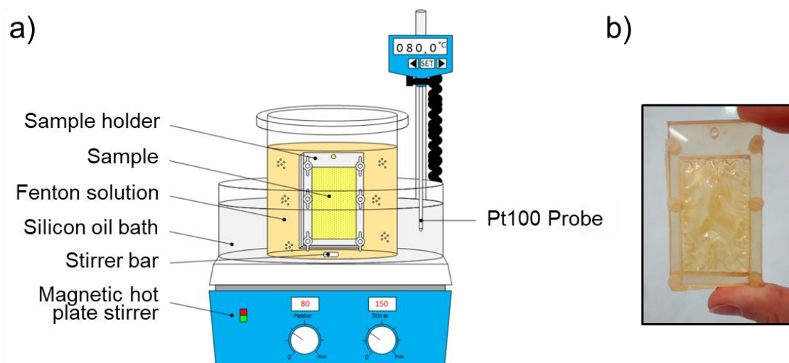
Figure 3.2 – (a) schematic representation of the ex-situ chemical degradation setup and (b) photograph of the polycarbonate frame holding a membrane sample.
