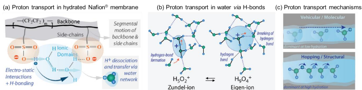
Figure 1.15 - Representation of the proton transport in hydrated Nafion ™ membranes as illustrated by Kusoglu et al. [77]: (a) Nafion ™ chemical structure and -SO_3H dissociation mechanism leading to the proton transport, (b) role of Zundel- and Eigen-ions in the proton transfer via H-bonds and (c) illustration of vehicular and hopping transport mechanisms.
