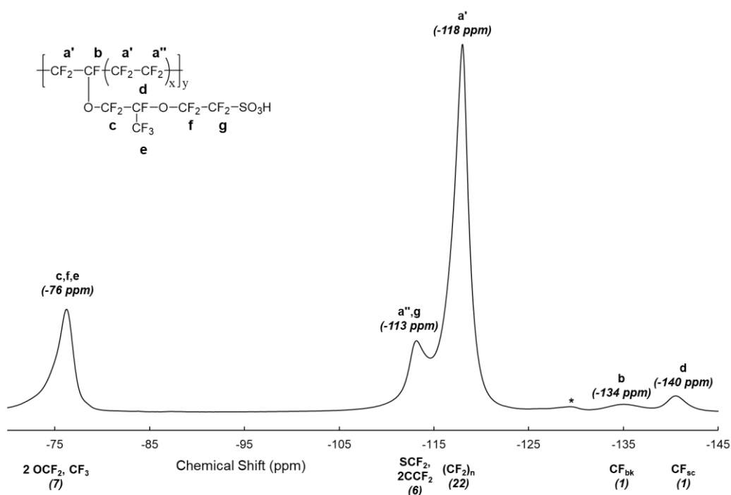
Figure 2.3 – solid-state ^{19}\text{F} -NMR spectra attribution for Nafion™ NR211 membrane and the corresponding peak areas predicted by Chen and Schmidt-Rohr [12]. The resonance peak with an asterisk designates a spinning sideband.
