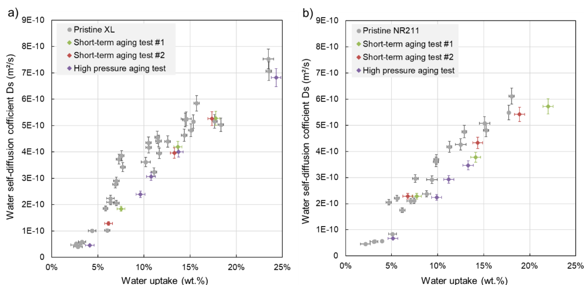
Figure 5.10 – Water self-diffusion coefficient evolution after various aging tests as a function of water uptake in (a) XL and (b) NR211 membranes (diamond symbols) in comparison with pristine membranes (circles).
