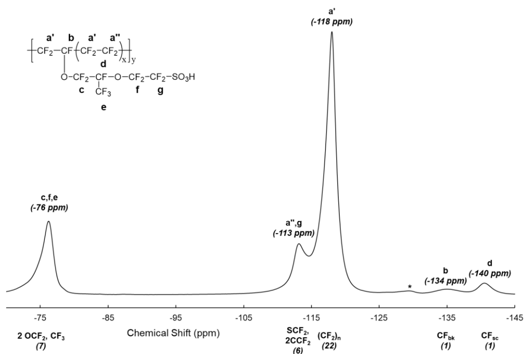
Figure 2.3 – solid-state 19 F-NMR spectra attribution for Nafion™ NR211 membrane and the corresponding peak areas predicted by Chen and Schmidt-Rohr [12]. The resonance peak with an asterisk designates a spinning sideband.
