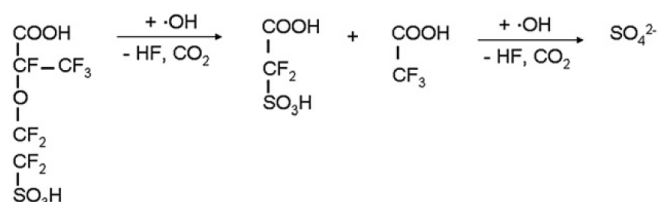
Figure 1.32 – Product A degradation via unzipping reaction [211].
