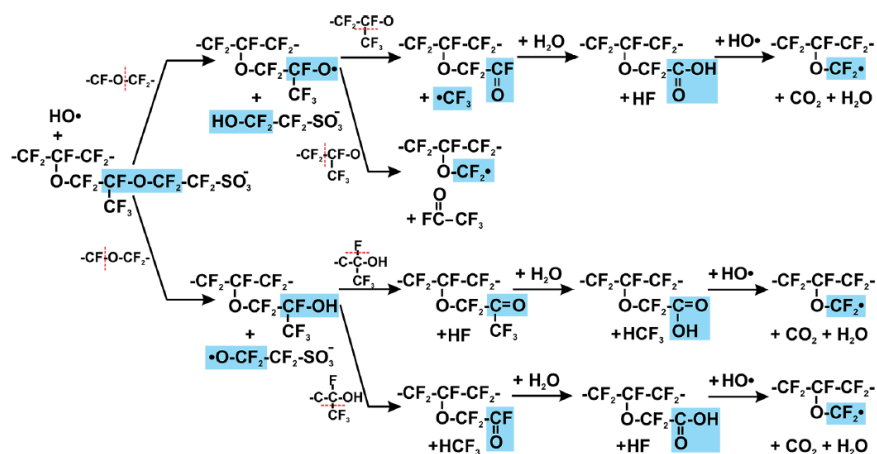
Figure 1.34 – Mechanism of \text{HO}^* radical attack on ether linkage proposed by Ghassemzadeh et al. [266].
