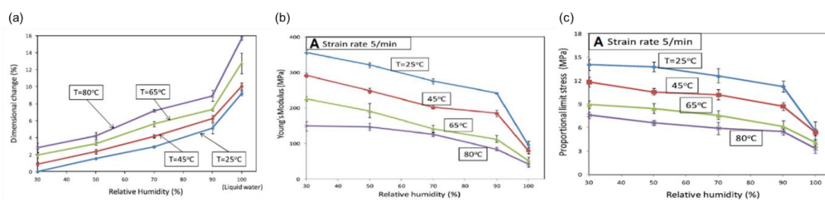
Figure 1.18 - Evolution of (a) in-plane swelling, (b) Young's modulus, (c) proportional limit stress of Nafion™ NR211 membrane as a function of relative humidity for various temperature [147].
