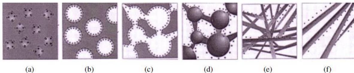
Figure 1.10 - Schematic representation of the Nafion™ structural evolution: (a) dry membrane , (b) swollen membrane, (c) percolation, (d) structure inversion, (e) connected network of polymer rods, (f) colloidal dispersion of rod-like particles (Adapted from ref. [103]).
