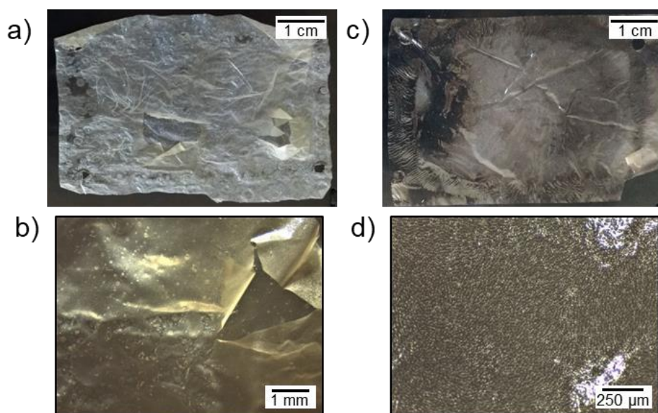
Figure 3.4 – Macroscopic changes after experiment #6 conducted with a high H 2 O 2 concentration (20 vol.%) and low Fe 2+ concentration (4 ppm) for Nafion™ XL, (a) without magnification and (b) with 8x magnification, as well as with Nafion™ NR211, (c) without magnification and (d) with 35x magnification.
