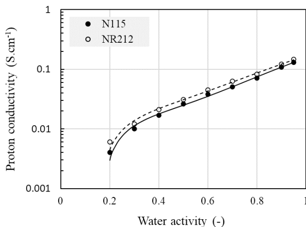
Figure 1.16 - Proton conductivity vs. water activity at 80°C for N115 and NR212 Nafion™ membranes (Adapted from ref. [125]).
