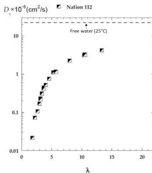
Figure 1.14 - Evolution of the water self-diffusion coefficient in Nafion™ N112 membrane at 25°C (Adapted from ref. [131]).
