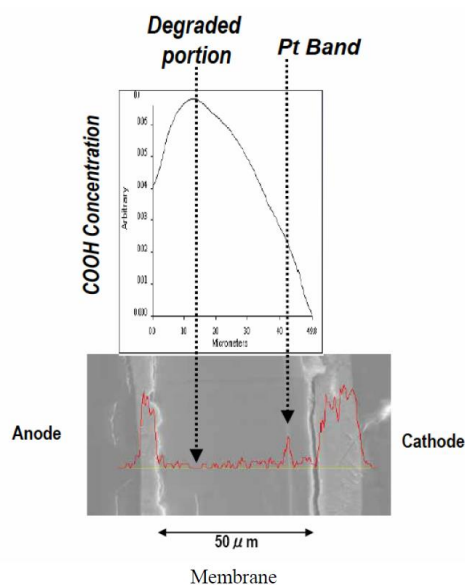
Figure 1.29 – COOH concentration profile in the cross-section of membrane degraded under OCV conditions thanks to electron probe microanalyzer (EPMA) and FTIR analyses [257].
