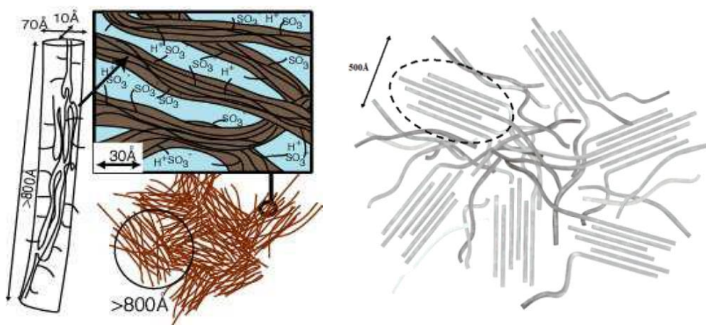
Figure 1.11 - Model of cylindrical polymeric aggregates proposed by Rubatat et al. [105,106].
