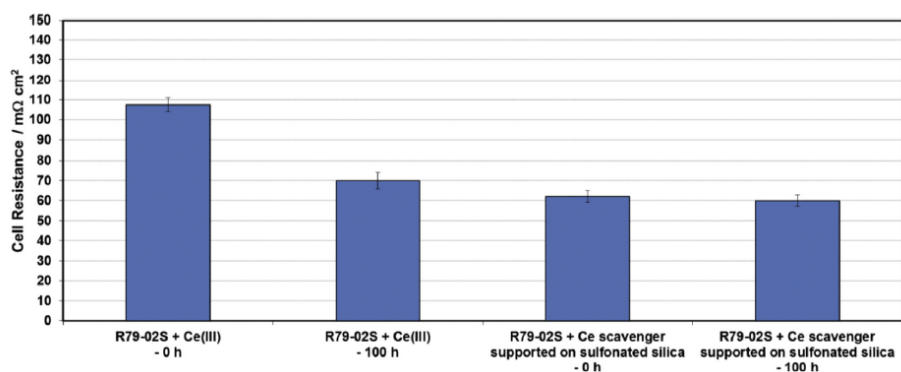
Figure 1.37 – Comparison of the cell resistance for MEA containing reinforced Aquivion ® PFSA membrane + Ce(III) ions or Ce scavenger supported on sulfonated silica at various operating time [296].
