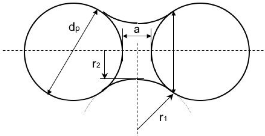
Figure 2.5 Liquid bridge between two identical spherical particles [59].
