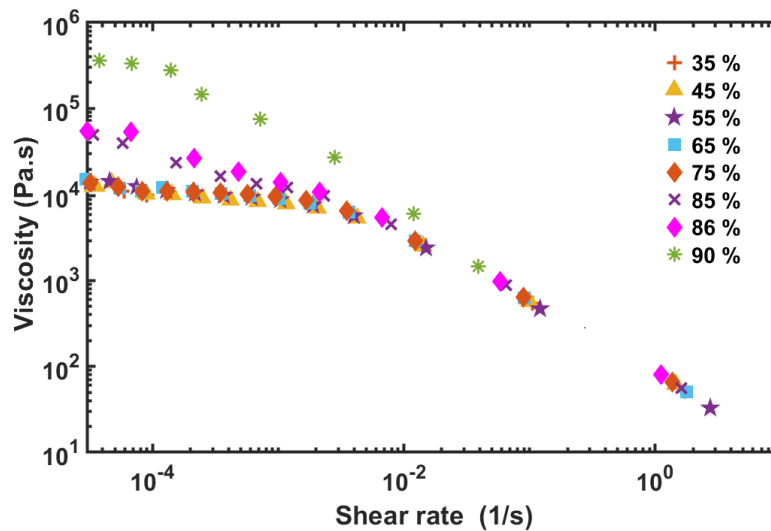
Figure 5.3 Flow curve of 100 \mu\text{m} glass bead for different values of humidity 35-90 % under 60 Hz of vibration stress. The amplitude of vibration is 100 \mu\text{m} .
