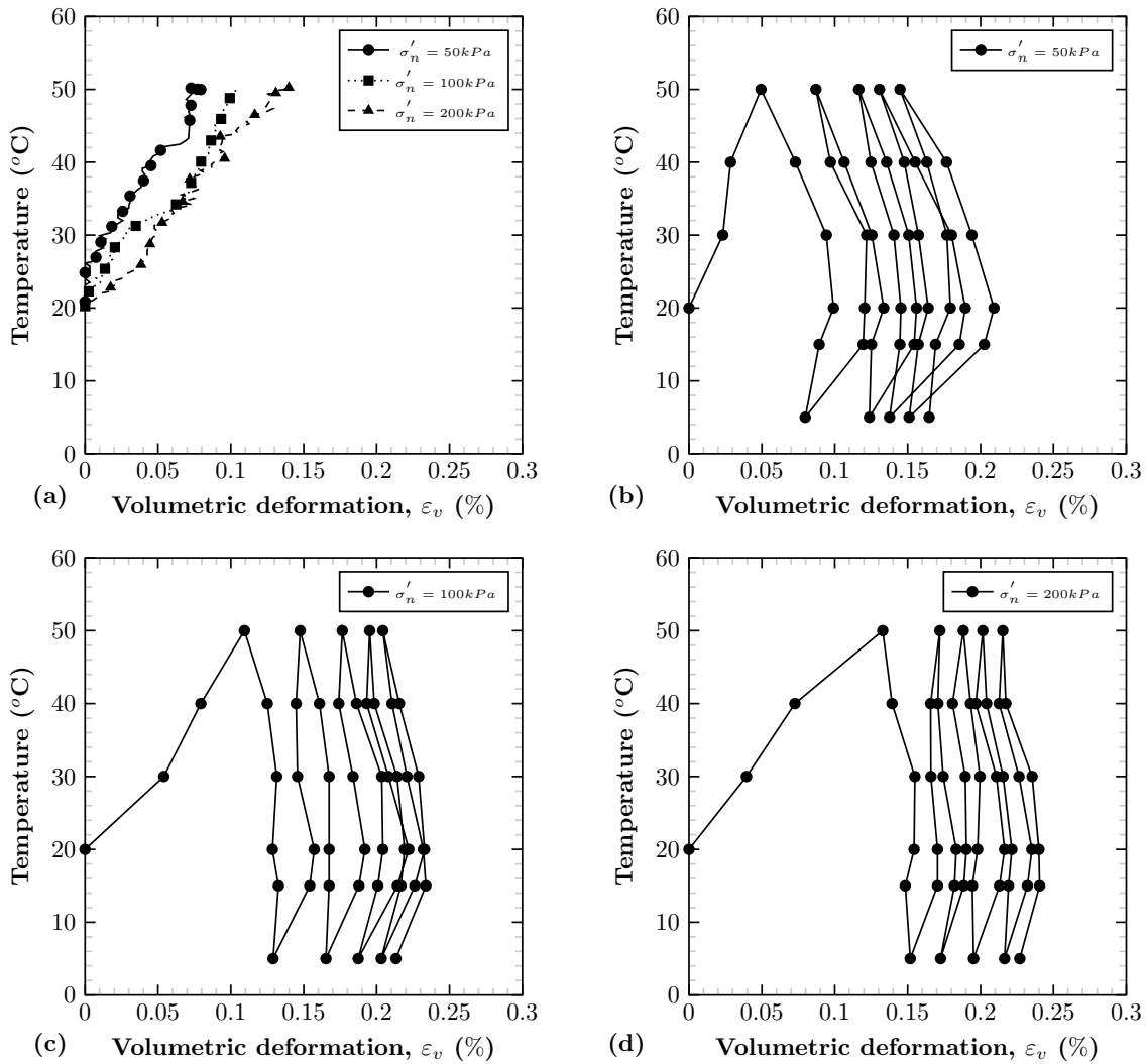
Figure 3.11: Thermal volumetric deformation (a) during heating from 20 to 50 °C (b), (c) and (d) during 5 thermal cycles at \sigma'_n = 50, 100 and 200 respectively.
