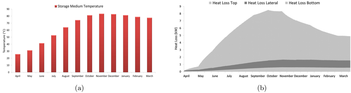
Figure 1.30: (a) temperature variation of storage medium during the one year (b) heat loss from the underground storage medium (Jradi et al. 2017).
