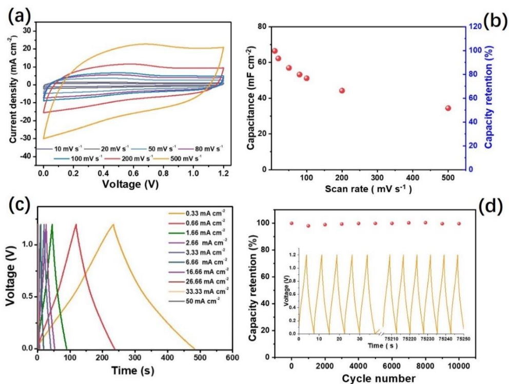
Figure 15. (a) The energy storage performance of EG@Fc-MS//EG hybrid pseudocapacitor in 1M H 2 SO 4 (a) CV curves at various scan rates (from 10 to 500 mV s -1 ); (b) Capacity values calculated from CV curves as a function of scan rate; (c) Galvanostatic charge-discharge curves of the device; (d) Cycling performance at constant current density of 13.3 mA cm -2 (initial and final five charge-discharge curves);
