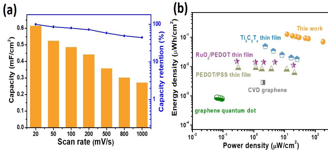
Figure 16. (a) The capacities of the Fc-MS//graphene devices on the basis of CV curves at various scan rates; (b) the Ragone plot of this device Ragone plots of this device and \text{PEDOT}/\text{PSS} , [127] \text{RuO}_2/\text{PEDOT} , [128] \text{Ti}_3\text{C}_2\text{T}_x , [135] Graphene quantum dot, [136] CVD graphene. [137]
