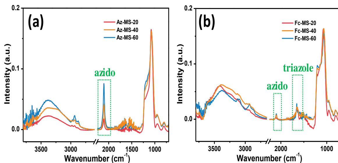
Figure 4. (a) IR spectra of Az-MS-20, Az-MS-40 and Az-MS-60; (b) IR spectra of Fc-MS-20, Fc-MS-40 and Fc-MS-60 (i.e., after click coupling of Az-MS samples). All spectra have been normalized based on the characteristic silica band at 1070 \text{cm}^{-1} .
