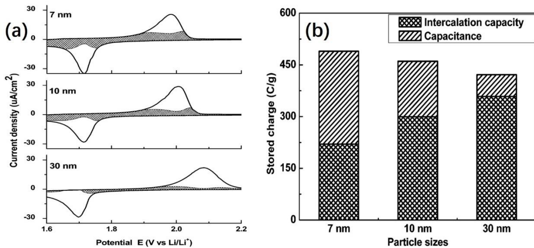
Figure 8. (a) Cyclic voltammograms of three TiO 2 films with different particle size (7nm, 10nm, 30nm) at scan rate of 0.5 mV s -1 . The total current (solid line) is obtained experimentally and the capacitive currents (shaded regions) are determined from fitting the data with the equation: i = k_1v + k_2v^{0.5} ; (b) the different contributions of battery-type current and capacitive current from different TiO 2 particle sizes (7 nm, 10 nm, 30 nm).[51]
