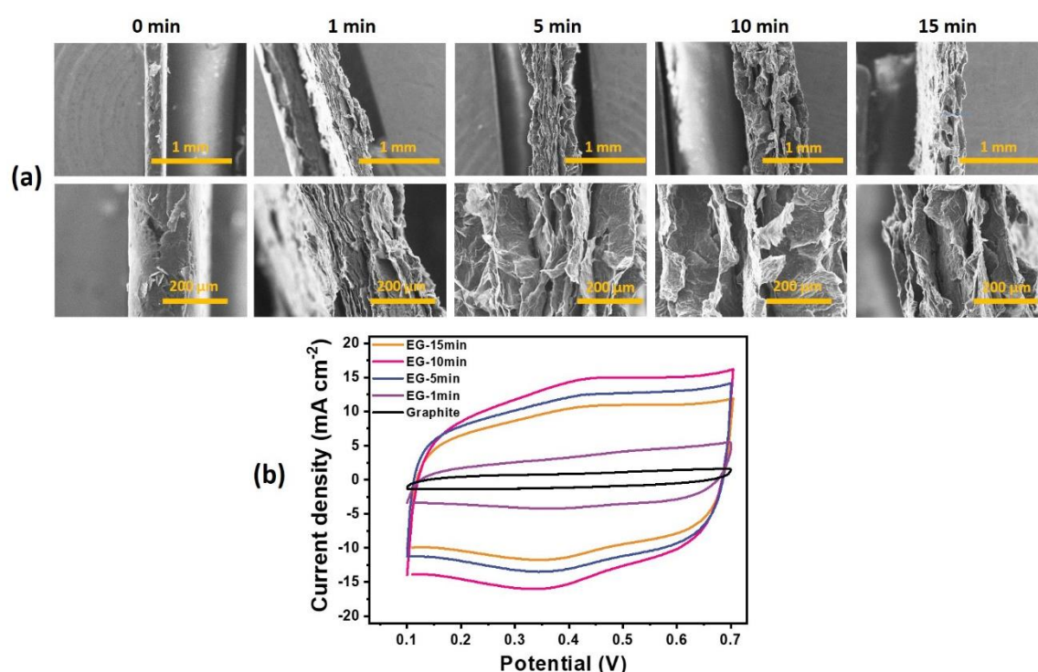
Figure 3. (a) The morphology evolution of graphite during the exfoliation process as a function of time; (b) the corresponding CV curves at a scan rate of 100 \text{ mV s}^{-1} in 1\text{M H}_2\text{SO}_4 electrolyte.
