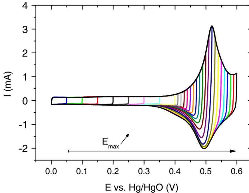
Figure 5. Cyclic voltammetry ( 10 \text{ mV s}^{-1} ) of an electroplated \text{Co}_3\text{O}_4 thin film annealed at 300 \text{ }^\circ\text{C} , using different upper potential limits, in 1 \text{ M KOH} electrolyte.
