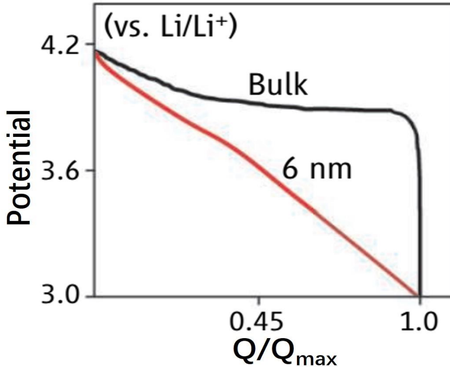
Figure 6. Difference of charge-discharge curves between bulk \text{LiCoO}_2 and nanosized (6 nm) \text{LiCoO}_2 .
