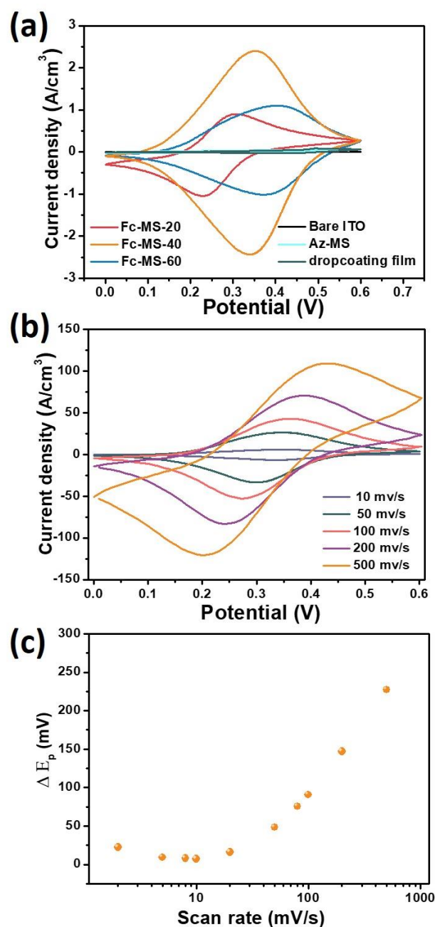
Figure 5. (a) Comparison of the CV curves recorded at of 5 \text{ mV s}^{-1} in 1 \text{ M LiCl} using bare ITO and ITO electrodes coated with Fc-MS-20, Fc-MS-40, Fc-MS-60, Az-MS and a ferrocene-functionalized film prepared from drop-coating method; (b) CV curves of the Fc-MS-40 film at scan rates varying from 10 to 500 \text{ mV s}^{-1} ; (c) Variation of the anodic-to-cathodic peak separation for Fc-MS-40 as a function of the potential scan rate (in the 2 \text{ mV s}^{-1} to 500 \text{ mV s}^{-1} range).
