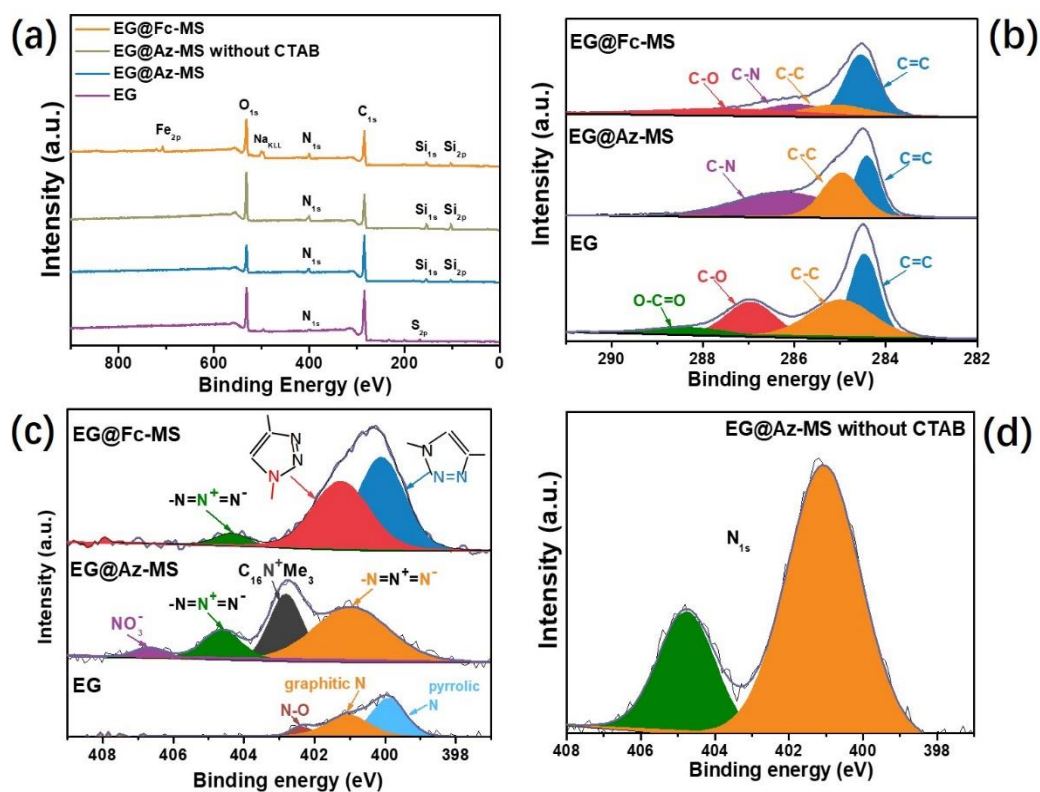
Figure 6. (a) XPS survey scan spectra of EG, EG@Az-MS (before and after CTAB removal) and EG@Fc-MS; (b) High resolution \text{C}_{1s} spectrum of EG, EG@Az-MS, and EG@Fc-MS; (c) High resolution \text{N}_{1s} spectrum of EG, EG@Az-MS, and EG@Fc-MS; (d) The high resolution \text{N}_{1s} spectrum of EG@Az-MS (after CTAB removal).
