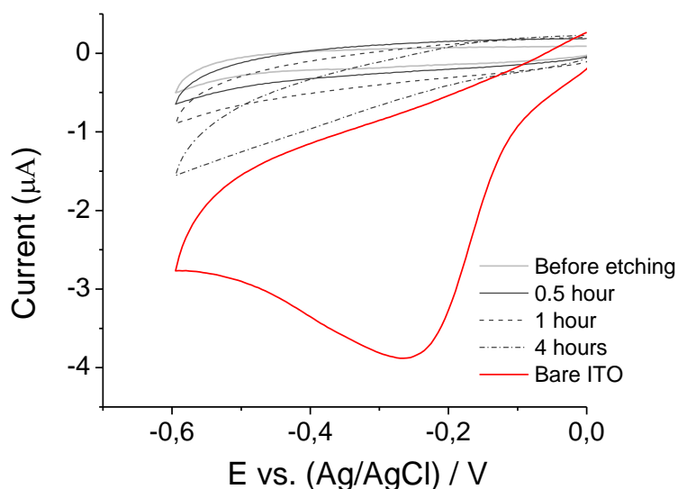
Figure 46 – Permeability of (A) gEXTR and (B) gCTAB MSF samples established by CV using 5 \mu\text{M} Hb deoxygenated solution in 0.1 M PBS (pH 5) before (grey bold line) and after etching with 0.05 M \text{NH}_4\text{F} for defined time (black lines). Comparison with the signal recorded on the bare ITO electrode (red line)
