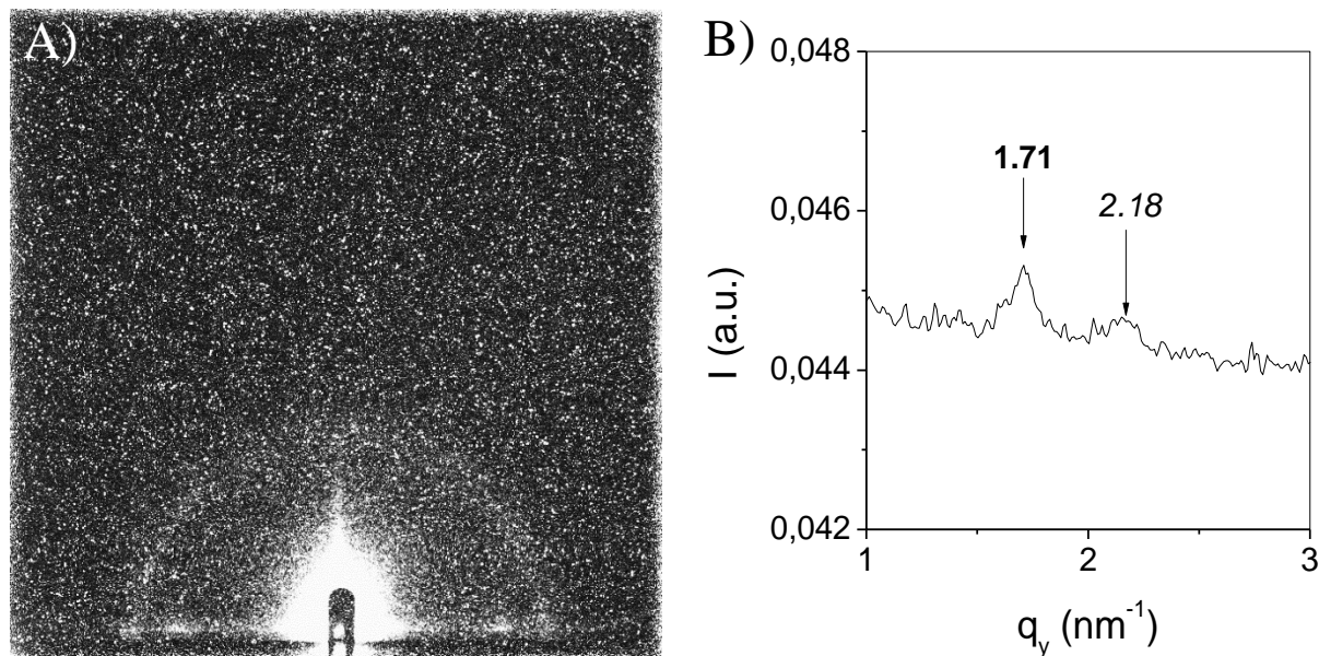
Figure 52 – (A) GISAXS pattern and (B) its integration recorded for gCTAB film after etching for 30 minutes in 0.10 M NH 4 F solution
