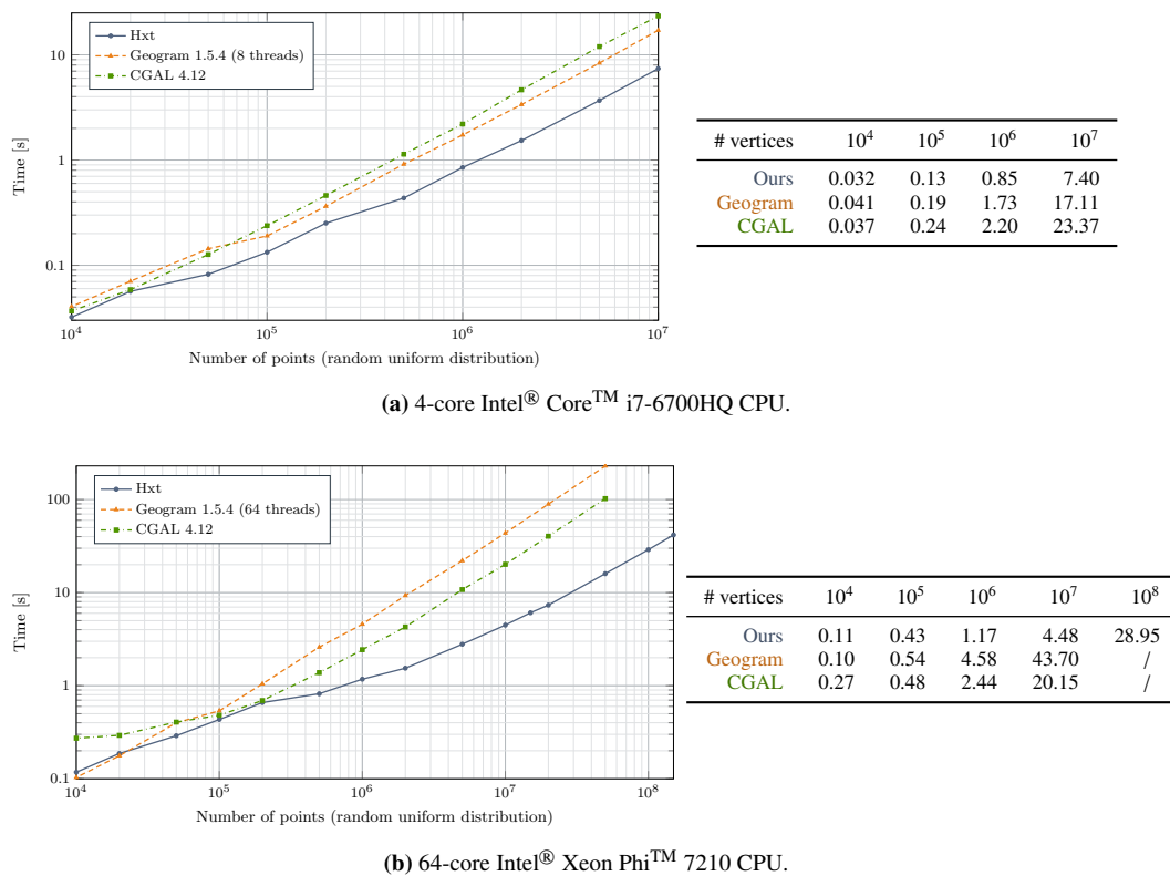
Figure 4.9: Comparison of our parallel implementation with the parallel implementation in CGAL (The CGAL Project 2016) and Geogram (Levy 2016) with on a high-end laptop (a) and a many-core computer (b). All timings are in seconds.
