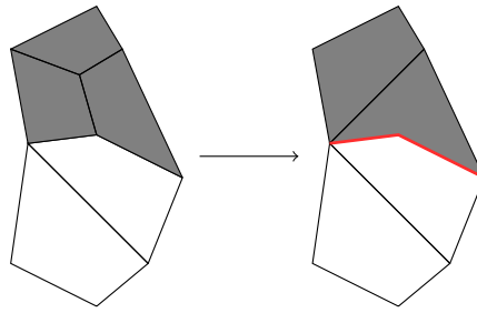
Figure 8.10: Replacing the cavity with a valid mesh sharing the same boundary still produces an invalid mesh by creating two quadrangles sharing two edges.
