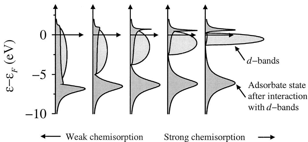
Figure 1.2: Newns–Anderson model of adsorbate–surface interactions [49, 52] : the local density of states projected onto an adsorbate state interacting with the d -bands at a surface. The strength of the adsorbate–surface coupling is kept fixed as the center of the d bands \epsilon_d is shifted up toward the Fermi energy ( \epsilon_F = 0 ).
