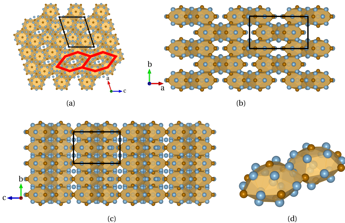
Figure 1.15: Bulk structure of m\text{-Al}_{13}\text{Fe}_4 : (a) along [010] (the hexagonal clusters are drawn in red), (b) along [001], (c) [100] and (d) two Al–Fe Henley-type clusters. Al and Fe atoms are drawn in light blue and dark orange, respectively.
