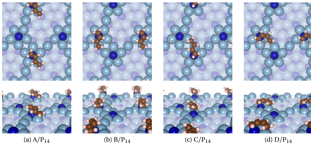
Figure 4.5: Adsorption sites of butadiene on P_{14} (top and perspective views). Al and Co atoms are drawn in light blue and dark blue, respectively.
