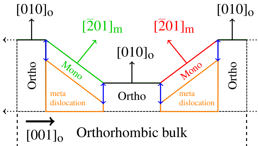
Figure 5.9: Schematic of the suggested surface model based on the experimental ob- servations. Orthorhombic flat terraces and monoclinic facets coexist in this model and are drawn in black and red/green (two different twin domains), respectively. Monoclinic/ orthorhombic interfaces are represented in blue. Metadislocations are displayed in or- ange.
