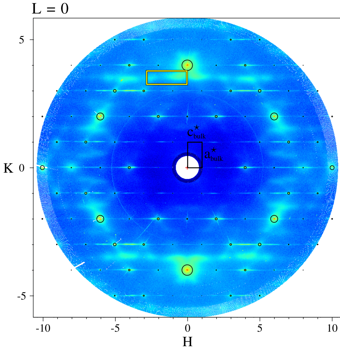
Figure 5.5: In-plane (H, K) reciprocal space map of o\text{-Al}_{13}\text{Co}_4 . The diffraction spots of the orthorhombic phase are indexed with black circles. The region presented in Fig. 5.7 is highlighted in yellow.
