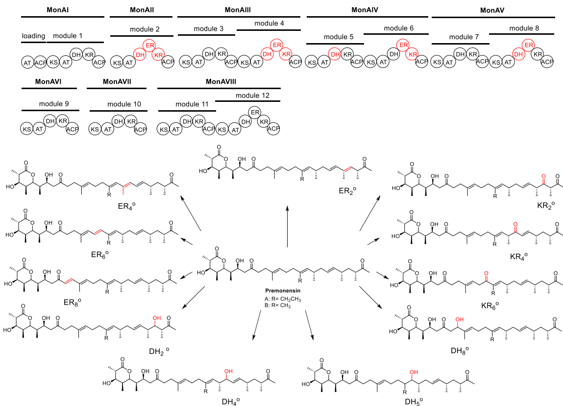
Figure 1.13 6-deoxyerythronolide (6-dEB) analogues generated by DEBS domain manipulation. The introduced modification include inactivation, deletion, and insertion of the tailoring domains KR, DH and ER (compounds 1–7), mutation, trans -AT complementation and replacement of AT domains (compounds 8–16), and relocation of the TE domain (compounds 17–20). The modified moieties in the analogues relative to 6-dEB have been highlighted in accordance with the color of their respective modules.
