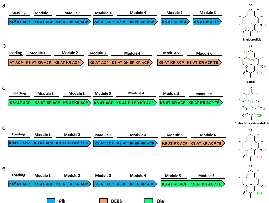
Figure 1.20 Modular arrangement of the native PKSs that produce narbonolide (a), 6-dEB (b) and 8, 8a-deoxyoleandolide (c), and the whole subunit swapped chimeric PKSs (d and e) that produce hybrid 14-membered macrolides. The main differences between the structure of these macrolides are highlighted in a manner consistent with the color of their respective assembly lines. KS Q indicates a KS domain whose catalytic cysteine is replaced by a glutamine residue. Adapted from reference [63].
