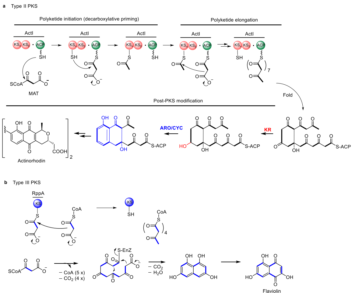
Figure 1.8 Examples of type II PKS and type III PKS involved in the biosynthesis of actinorhodin and flaviolin, respectively. a) The chain length factor (CLF also named KS_{\beta} as shown here) and ketosynthase ( KS_{\alpha} ) form a heterodimer. A malonyl-CoA:ACP transacylase (MAT) primes the ACP with a malonate unit. The biosynthesis begins with the decarboxylation of a malonyl unit tethered to the KS_{\alpha} , followed by Claisen condensation with an activated malonyl unit attached to the ACP. Seven rounds of Claisen condensation takes place overall to reach the required chain length. Upon release, the product undergoes processing by KR and CYC/ARO and additional enzymes to produce actinorhodin. b) Synthesis of flaviolin by a type III polyketide synthases/chalcone synthase. The growing chain is shown attached to a single KS-like enzyme (RppA). The malonyl-CoA starter unit is condensed iteratively with four additional malonyl-CoA units, followed by aromatization to the final product. Adapted from reference [64].
