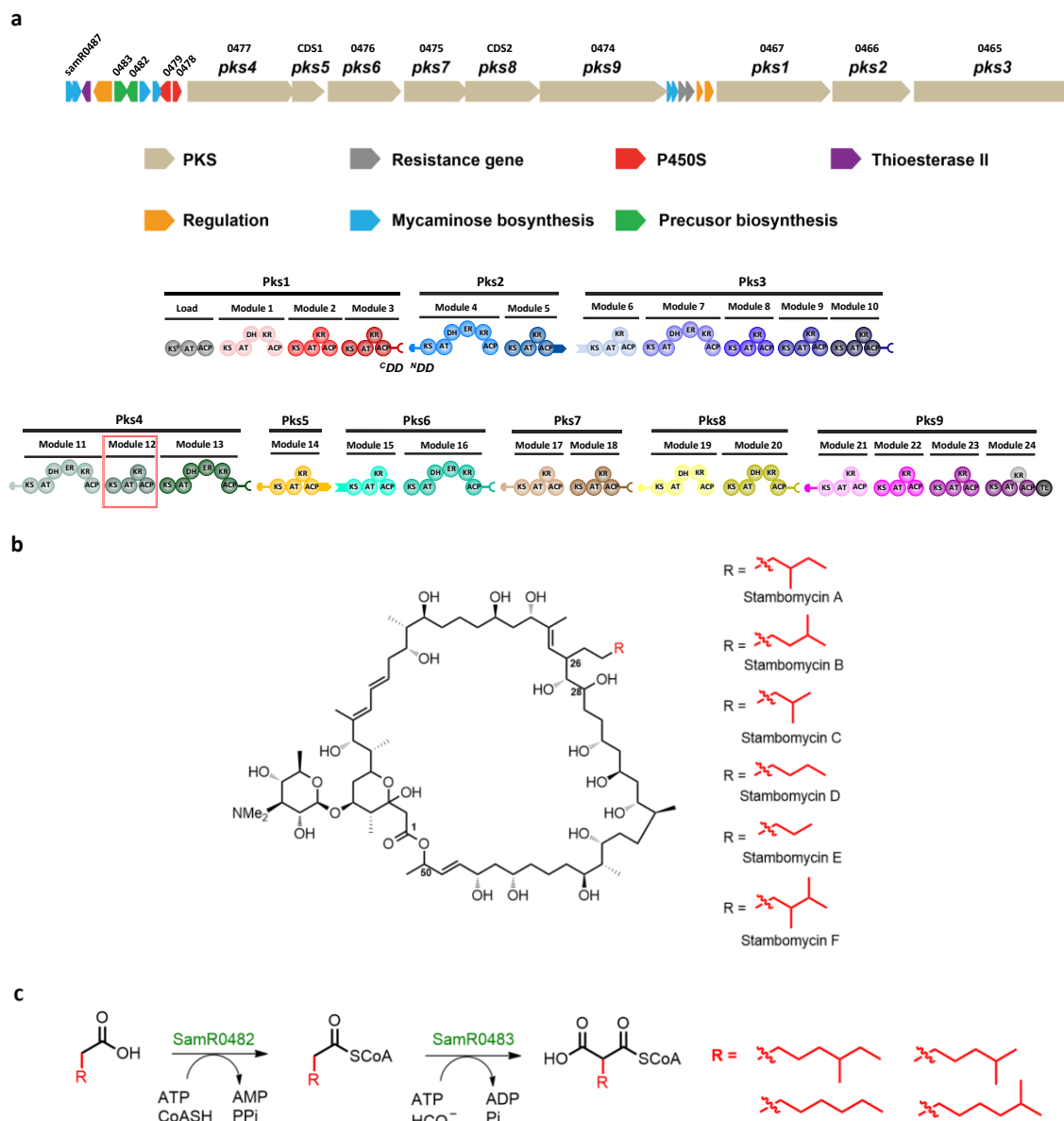
Figure 1.36 Biosynthesis of the stambomycins in S. ambifaciens ATCC23877. a) Organization of the stambomycin biosynthetic gene cluster showing the domains, modules, subunits and docking domains. The AT domain of PKS module 12 (red boxed) recruits six alternative extender units, resulting in the small family of stambomycins. The last KR domain on module 24 (grey) is inactive. b) Structures of the stambomycins A–F, showing the differences in their side chains at C-26. The configurations of the \alpha - and \beta -stereocenters generated by each KR domain was predicted based on Keatinge-Clay's model [166]. c) The elucidated biosynthetic pathway to the unusual stambomycin PKS extender units. SamR0482, an acyl-CoA synthetase, catalyzes the activation of precursor originating from fatty acid metabolism using the cofactor ATP and coenzyme A. SamR0483, an acyl-CoA carboxylase, catalyzes the subsequent ATP-dependent carboxylation reaction, resulting in the final extender units. Adapted from reference [85, 160, 161].
