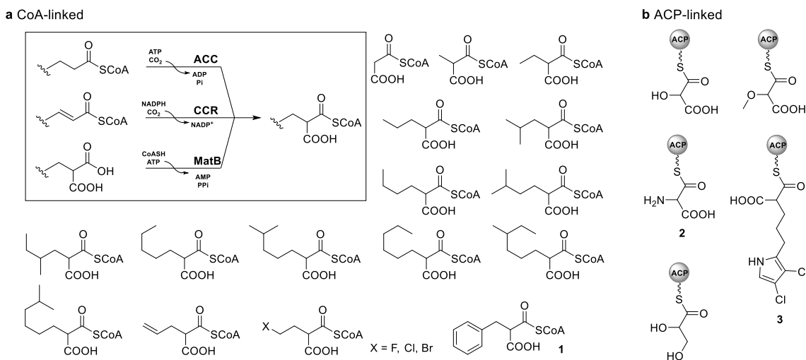
Figure 1.9 Structures of natural polyketide extender units. Benzylmalonyl-CoA ( 1 ), aminomalonyl-ACP ( 2 ), and dichloropyrrolymalonyl-ACP ( 3 ) are notably derived from amino acids. Adapted from reference [81].
