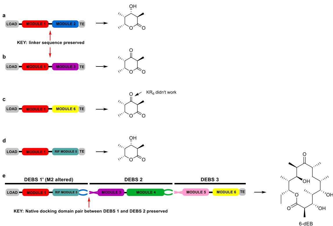
Figure 1.17 Whole module swapping as an engineering approach. a ) DEBS 1-TE mini PKS model system and its triketide lactone product. b, c ) Variants of DEBS 1-TE containing heterologous module 2s, and their respective triketide lactone products. Communication between module 1 of DEBS and two non-cognate modules from the DEBS system (3 and 6) was achieved by preserving the native intermodular linker between modules 1 and 2. d ) The same strategy resulted in successful cross-talk between DEBS module 1 and module 5 from the rifamycin (RIF) PKS. e ) By preserving the native docking interaction between subunits 1 and 2,
