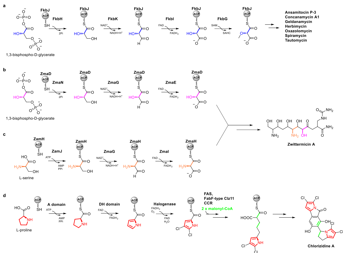
Figure 1.12 Biosynthetic pathway to ACP-tethered extender units and their corresponding polyketide products. a ) In S. hygroscopicus , a five-gene set encodes the enzymes responsible for (2 R )-methoxymalonyl-ACP in the FK520 biosynthetic pathway. Homologues of these genes are present in the BGCs for concanamycin A1, geldanamycin, herbimycin, oxazolomycin, spiramycin and tautomycin. b ) Pathway to (2 R )-hydroxymalonyl-ACP, for which the FkbG-homologue is absent. c ) A novel pathway from serine to aminomalonyl-ACP involving an FkbI-homologue (ZmaI), FkbK-homologue (ZmaG), carrier protein ZmaH, and a special enzyme ZmaJ with specificity for L-serine. Both (2 R )-hydroxymalonyl-ACP and aminomalonyl-ACP are utilized as extender units in zwittermicin A biosynthesis. d ) Biosynthesis of L-proline derived monomers dichloropyrrolyl-ACP and dichloropyrrolylpropylmalonyl-ACP in the biosynthesis of chlorizidine A. The biosynthesis starts from the loading of L-proline onto an ACP by an adenylation (A) domain, followed by FAD-dependent oxidation (dehydrogenase), which converts the prolyl ring to a pyrrole. Subsequent halogenation by an FADH 2 -dependent halogenase (Hal) then installs two halogens on the pyrrole ring, resulting in dichloropyrrolyl-ACP, which is used as a starter unit to prime the biosynthesis of chlorizidine A (top red pyrrole ring). Extension of dichloropyrrolyl-ACP with malonyl-CoA is then carried out by Clz11, a FabF-type enzyme, a FAS and a CCR in parallel, giving rise to dichloropyrrolylpropylmalonyl-ACP, which is then incorporated into the chlorizidine A scaffold as an extender unit (bottom red pyrrole ring). Adapted from reference [79, 80].
