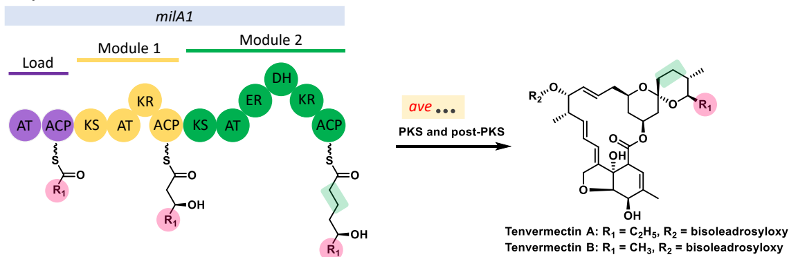
Figure 1.21 Generation of tenvermectins by exchanging the subunit AveA1 for MilA1. The differences between the parent avermectin and milbemycin structures are shown with highlighted colors, as well as the structure of the hybrid tenvermectins [120].
