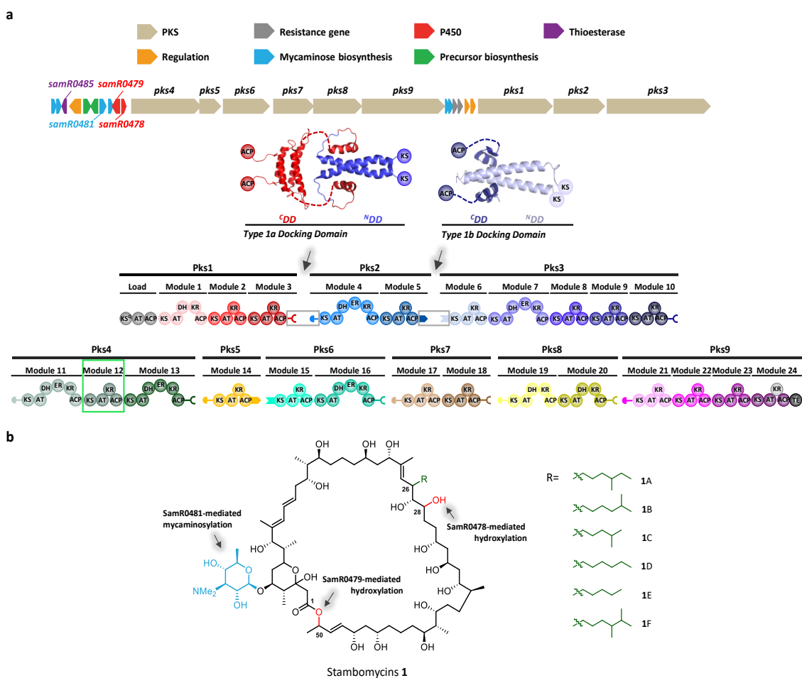
Fig. 1 Stambomycin polyketide synthase (PKS) and structures of stambomycin derivatives produced by S. ambifaciens ATCC23877. a Organization of the stambomycin biosynthetic gene cluster, and schematic of the encoded PKS subunits (Pks1–Pks9) showing the component modules and domains, as well as the intersubunit docking domains. The DDs belong to two distinct structural classes (type 1a and type 1b), for which representative NMR structures of complexes are shown 22,27 . The AT domain of PKS module 12 (green box) is responsible for recruiting six alternative extender units, resulting in a small family of stambomycins. The last KR domain of module 24 (grey) is inactive. b Structure of stambomycins 1 (A–F), which differ from each other in the alkyl functionality (R group) at position C-26
