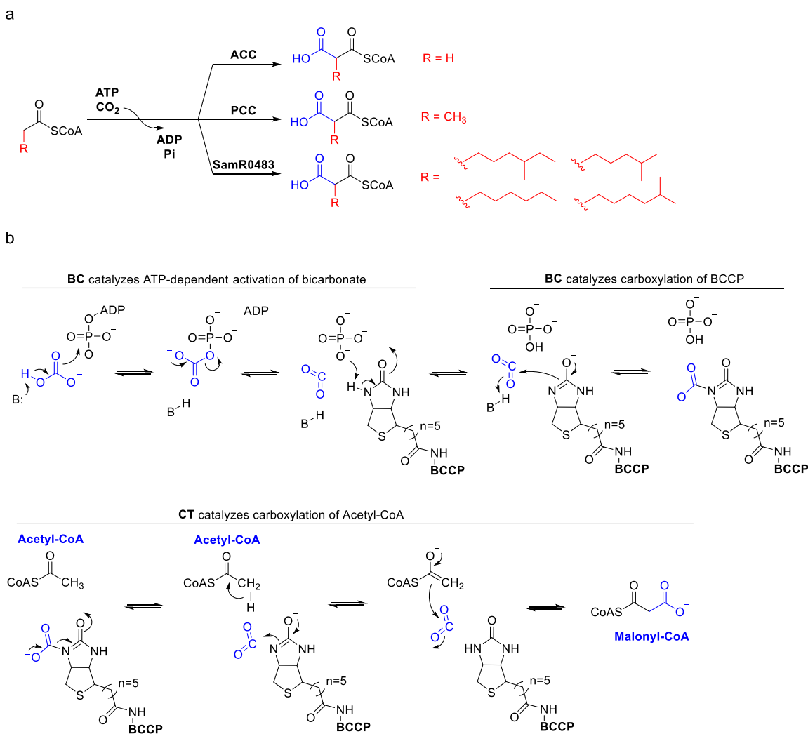
Figure 1.10 Biosynthesis of CoA-linked extender units by ACC/PCC/SamR0483-dependent pathways. a) ACC/PCC/SamR0483-catalyzed reactions. b) Mechanism of the ATP- and biotin-dependent reactions, exemplified by the ACC pathway. Adapted from reference [79]
