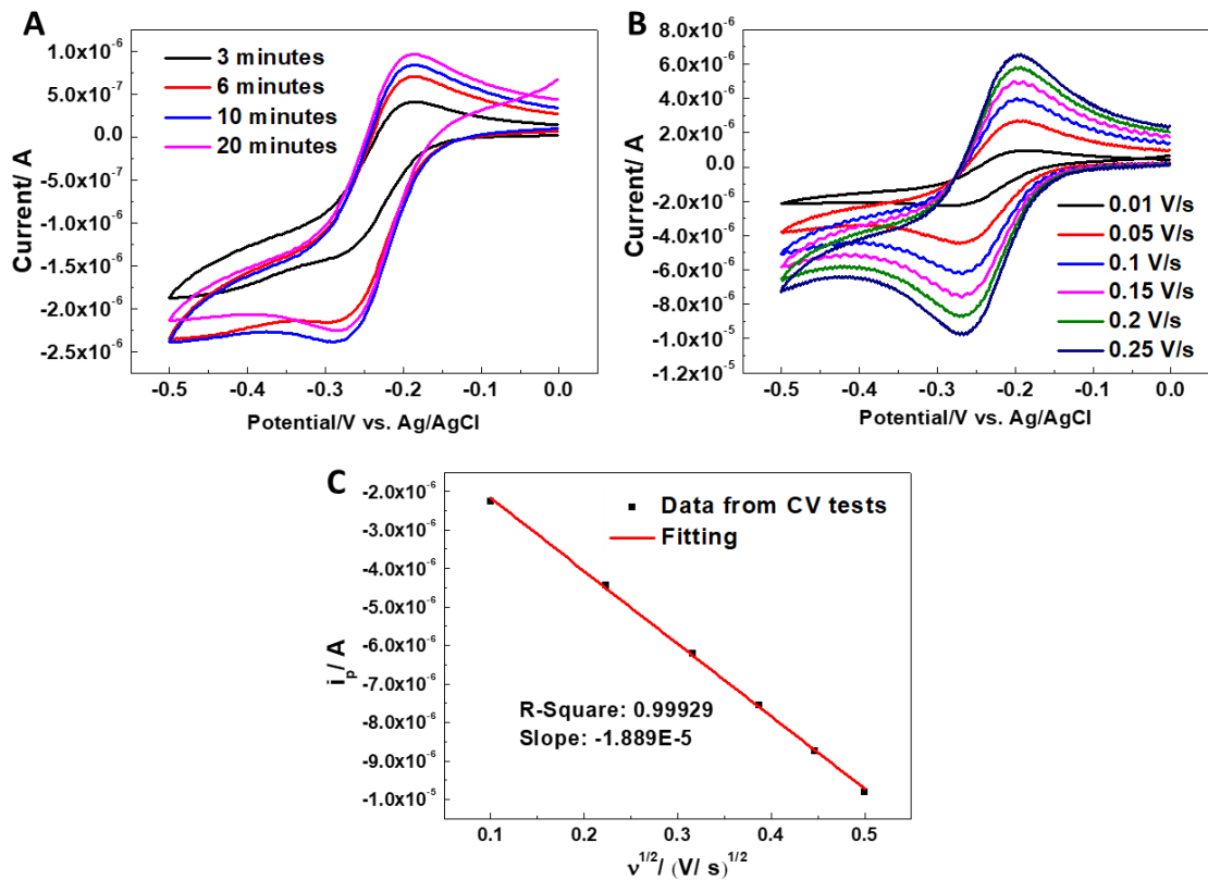
Figure A10 CV test of cross-linked hydrogel on planar electrode in 0.1mM \text{Ru}(\text{NH}_3)_6\text{Cl}_3 solution after different immersion time (scan rate:10mV/s)(A), CV test of cross-linked hydrogel in 0.1mM \text{Ru}(\text{NH}_3)_6\text{Cl}_3 solution at different scan rate (B), linear fitting of peak current in Figure A10B with scan rate (C).
