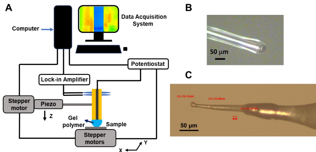
Figure 1.19 Scheme of the SGECEM setup (A), gel probe fabricated on a micro-disk electrode (B), gel probe fabricated on an etched metal wire (C).
