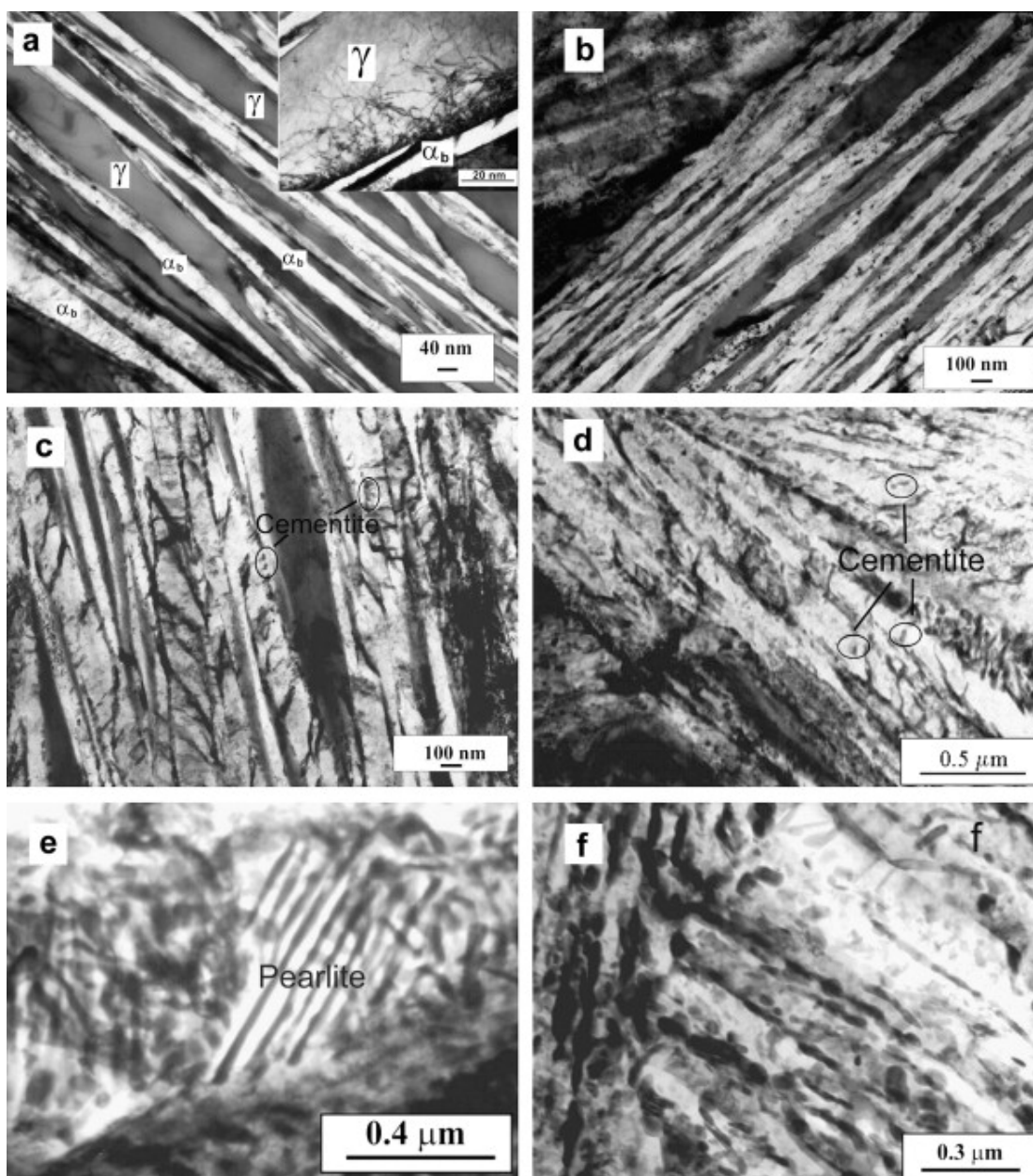
Figure I.14 – TEM micrographs showing the microstructural evolution during tempering of Fe-0.98C-1.46Si-1.89Mn-0.26Mo-1.26Cr-0.09V wt.% steel: a) initial, b) 400°C 1 hour, c) 450°C 30 minutes, d) 500°C 30 minutes, e) 550°C 1 hour and f) 600°C 30 minutes [105].
