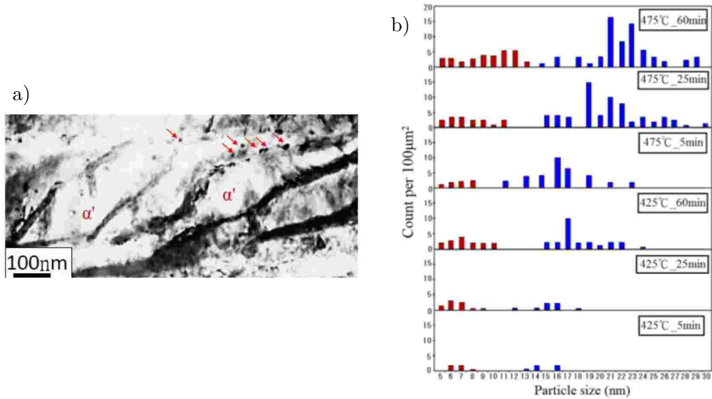
Figure I.18 – a) BF TEM micrograph of nano-bainite after tempering during 1 hour at 475°C showing carbide between the ferrite laths (red arrows) and b) carbide size distribution in two different regions, red for ferrite and blue for between ferrite laths, for different tempering conditions [119].
