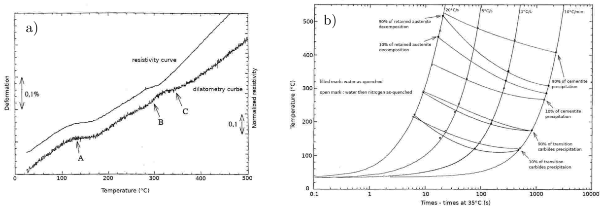
Figure I.5 – a) dilatometric and resistivity curves during a continuous heating ( 10^\circ\text{C/s} ) from a as-water-quenched state (8% retained austenite). Label A represents the precipitation of transition carbides, B the beginning of retained austenite decomposition, and C cementite precipitation. b) continuous heating diagram obtained from two as-quenched state for a 70MnCr5 steel [10].
