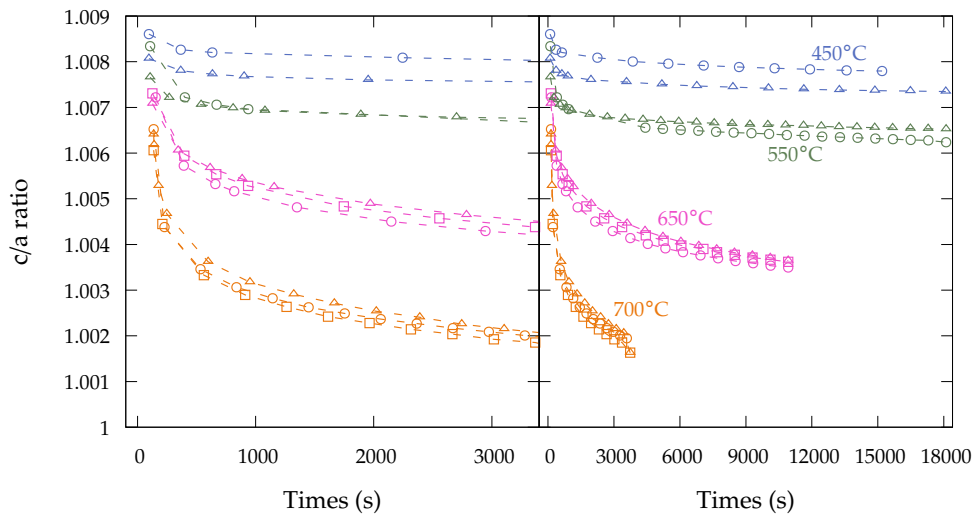
Figure IV.21 – Martensite/bainitic ferrite tetragonal ratio ( c/a ) evolutions as function of time during the tempering of the three initial microstructures at 450, 550, 650 and 700°C. Squares, circles, triangles for LNM, RTM and NB respectively; 700°C: orange, 650°C: pink, 550°C: green and 450°C: blue.
