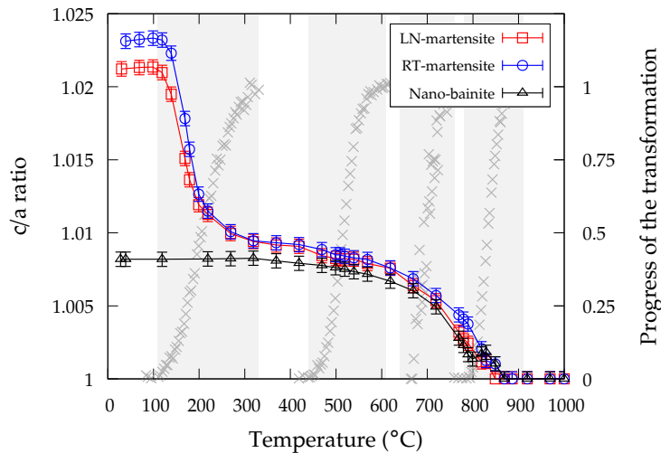
Figure IV.8 – Tetragonal ratio ( c/a ) evolution of martensite/bainitic ferrite during the continuous heating treatment 1^\circ\text{C/s} for the three initial microstructures. The grey curves represent the precipitation kinetics (progress of the transformation) extracted from dilatometry for LNM microstructure (see figure IV.1), and grey areas are the temperature ranges of each precipitation kinetics.
