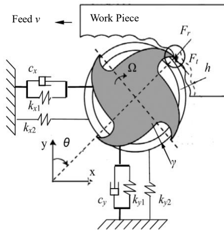
Figure 5. 1 Dynamic model of the milling process with bearing clearance fault [1].
