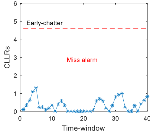
Figure 5.21 Missing alarm caused by the decrease in the background noise.
