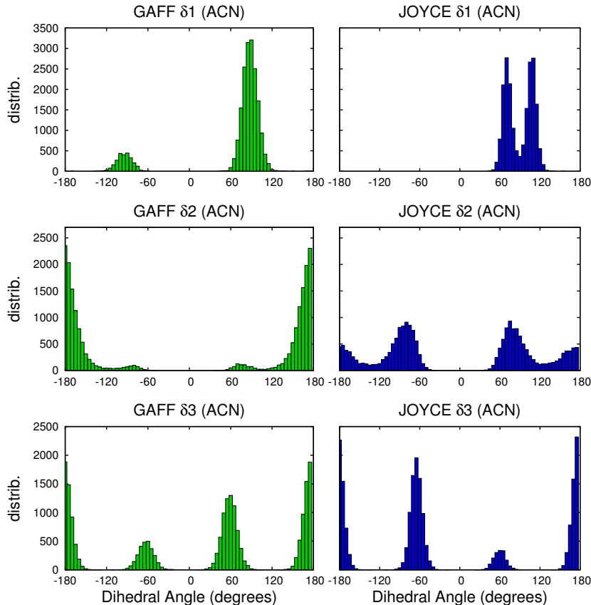
Figure 2.18: Dihedral distributions computed from the PDI@ACN MD runs by using the GAFF FF and the JOYCE FF. The labels of the flexible dihedrals are given in Figure 2.16.
