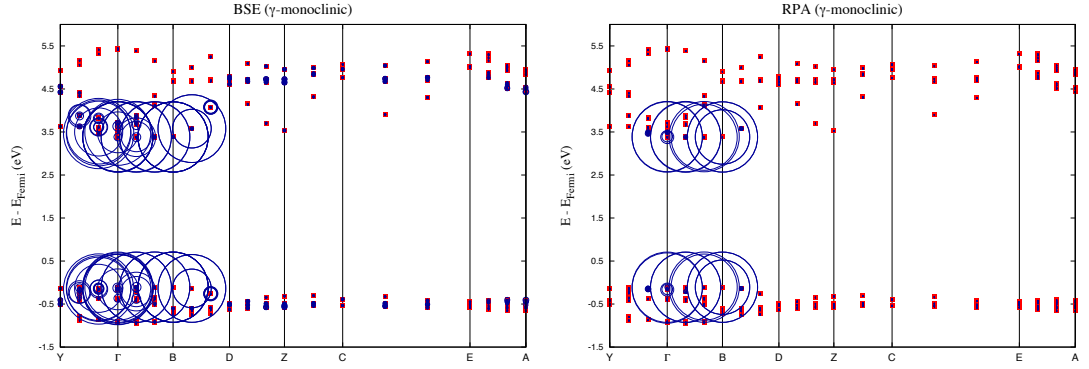
Figure 4.8: GW band structure for the room temperature monoclinic phase of \text{WO}_3 considering the eight uppermost occupied bands and the eight bottommost unoccupied bands (red dots). The blue circles represent the contribution of the electron-hole pair at a given k-points and for a given occupied band-unoccupied band pair to the first bright excitation computed at BSE level (left) and at RPA level (right).
