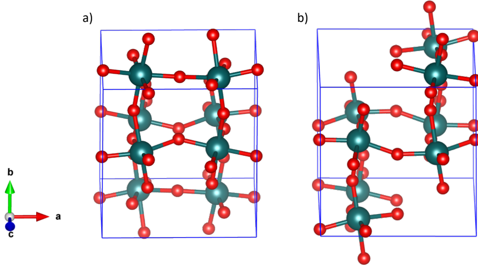
Figure 4.3: LDA relaxed crystal structure of the \gamma monoclinic phase (left) and the triclinic phase (right) of \text{WO}_3
