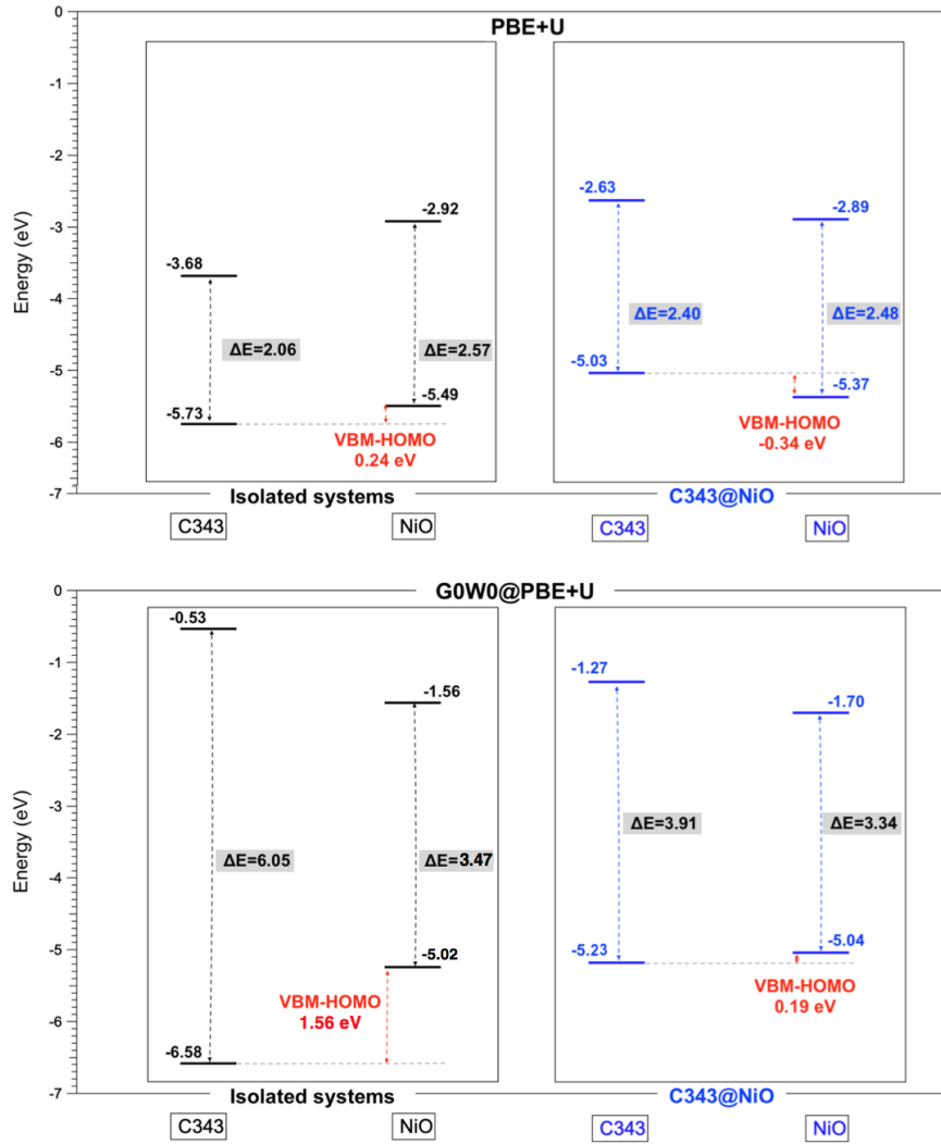
Figure 3.9: PBE+U (top panel) and G_0W_0 @PBE+U (bottom panel) energy levels with respect to the vacuo of the C343 HOMO/LUMO and NiO VBM/CBM as computed for the isolated systems (data in Table 3.2) and for the C343@NiO interface model. The band gaps and driving forces for the hole injection from the dye to the Semiconductor (VBM-HOMO) are also reported.
