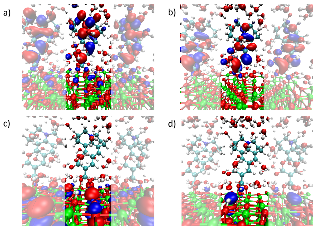
Figure 3.13: Calculated isosurfaces of the HOMO (a), LUMO (b), VBM (c) and CBM (d) Kohn-Sham orbitals of the Interface system in water solution calculated from a snapshot extracted at the early stage of the MD simulation
