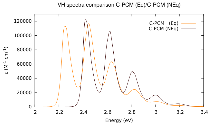
Figure 2.25: PDI static vibronic spectra in ACN calculated by considering both the Equilibrium (Eq) and the Non-Equilibrium (NEq) C-PCM model.
