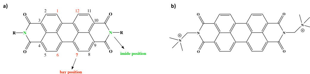
Figure 2.1: a) Chemical structure of a generic PDI sensitizer: the bay and imide positions are evidenced in red and green, respectively. b) N,N'-bis(2-(trimethylammonium)-ethylene)-perylene-3,4,9,10-tetracarboxylic acid bis-imide PDI molecule investigated in this thesis.
