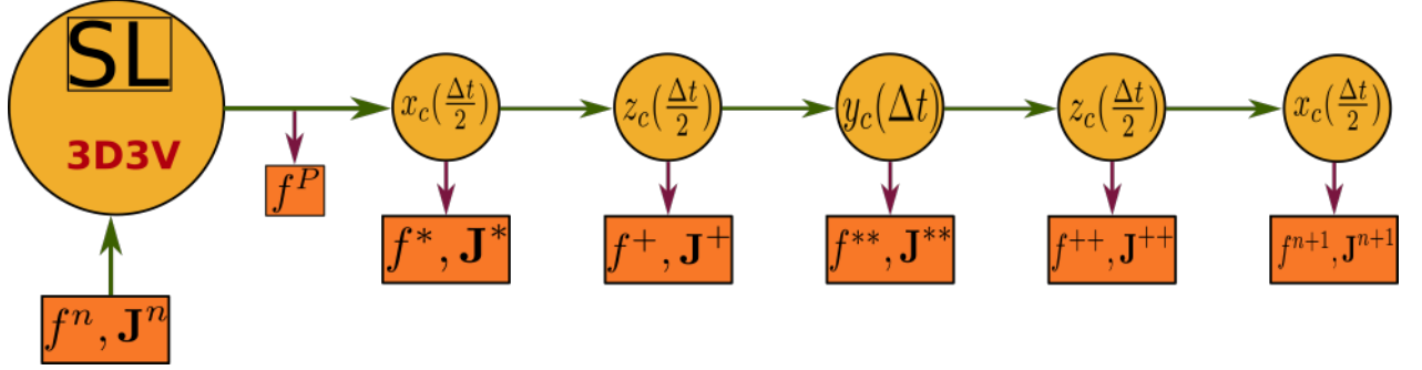
Figure 3.5: Strang Splitting for 3D3V phase space. At each advection step, the updated values of the distribution function and of the current density are stored to be used later with Esirkepov correction method.
