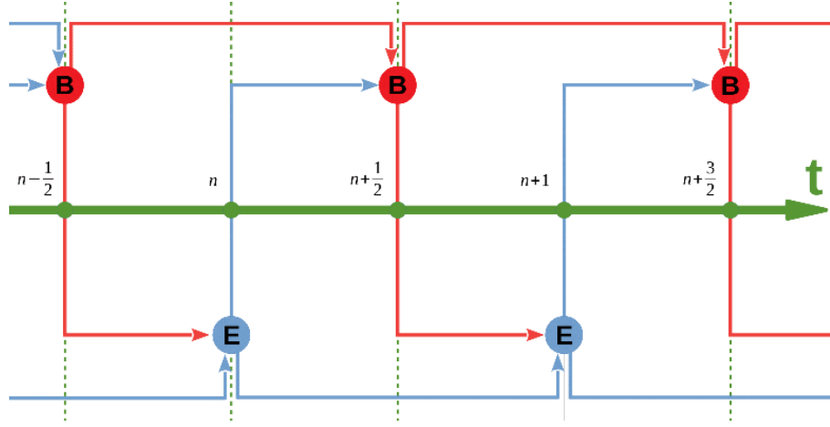
Figure 3.1: Temporal part of Yee algorithm. As shown, estimating magnetic field \mathbf{B} at time step n + \frac{1}{2} requires providing the values of fields \mathbf{E} , and \mathbf{B} at steps n and n - \frac{1}{2} , respectively.
