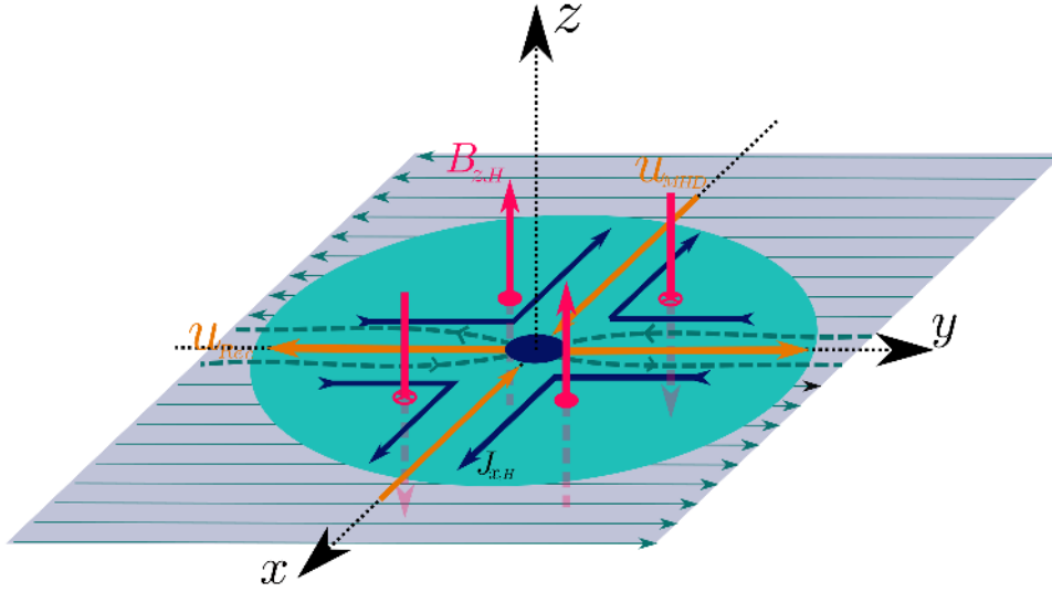
Figure 5.2: Effects of Hall term on reconnection: the outer circle represents the width of the collisionless current sheet where the motion of the ions starts to decouple from that of electrons. Black arrows denote the Hall current which is opposite to the electrons convective motion (orange arrows) toward X point shown as a small black circle. Hall term generates a Hall magnetic field (red arrows) in a direction perpendicular to the reconnection plane.
