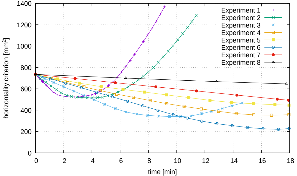
Figure 4.13: Values of the expected horizontality criterion (Eq. (4.7)) throughout time for the simulations of the design of experiments (Fig. 4.12) to find the effective material properties inside the analogue model.
