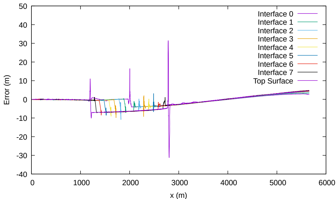
Figure 3.13: Error on the restoration of the interfaces in the simplified graben model. The lower the number of the interface, the lower the interface it corresponds to. For example, interface 0 is the interface between the salt and the lowest sediment layer.
