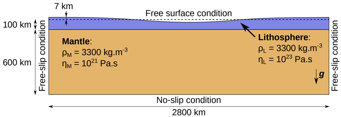
Figure 2.11: Model setup for the 2D free surface benchmark.
