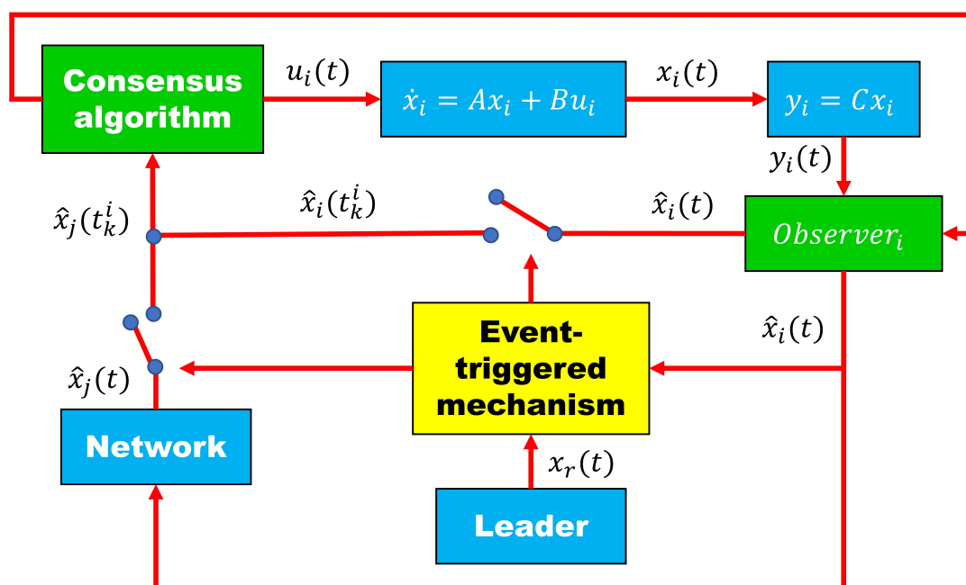
Fig. 3.1: Event-triggered control scheme in multi-agent systems.
