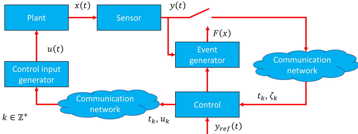
Fig. 2.10: Event-based control loop [101].
