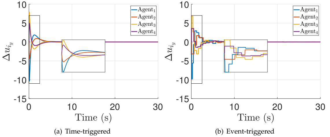
Fig. 3.7: Comparison of the control profile \Delta u_{i_y}(t) between time- and event-triggered control.
