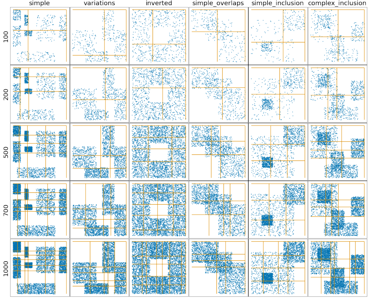
Figure 5.9: The results of IPD discretization for the synthetic data
