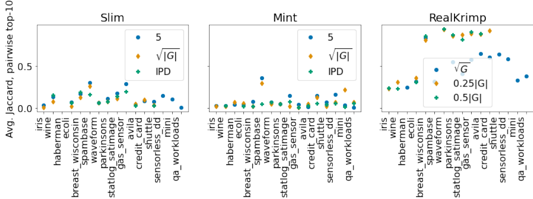
Figure 5.5: The average Jaccard similarity computed on the top-10 Jaccard-similar pairs for each pattern, repetitive pairs are discarded
