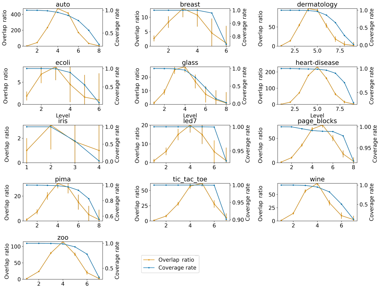
Figure 3.14: Coverage rate and mean overlap ratio of the cells by levels. The vertical lines show the standard deviation of the overlap ratio over cells within a given level
