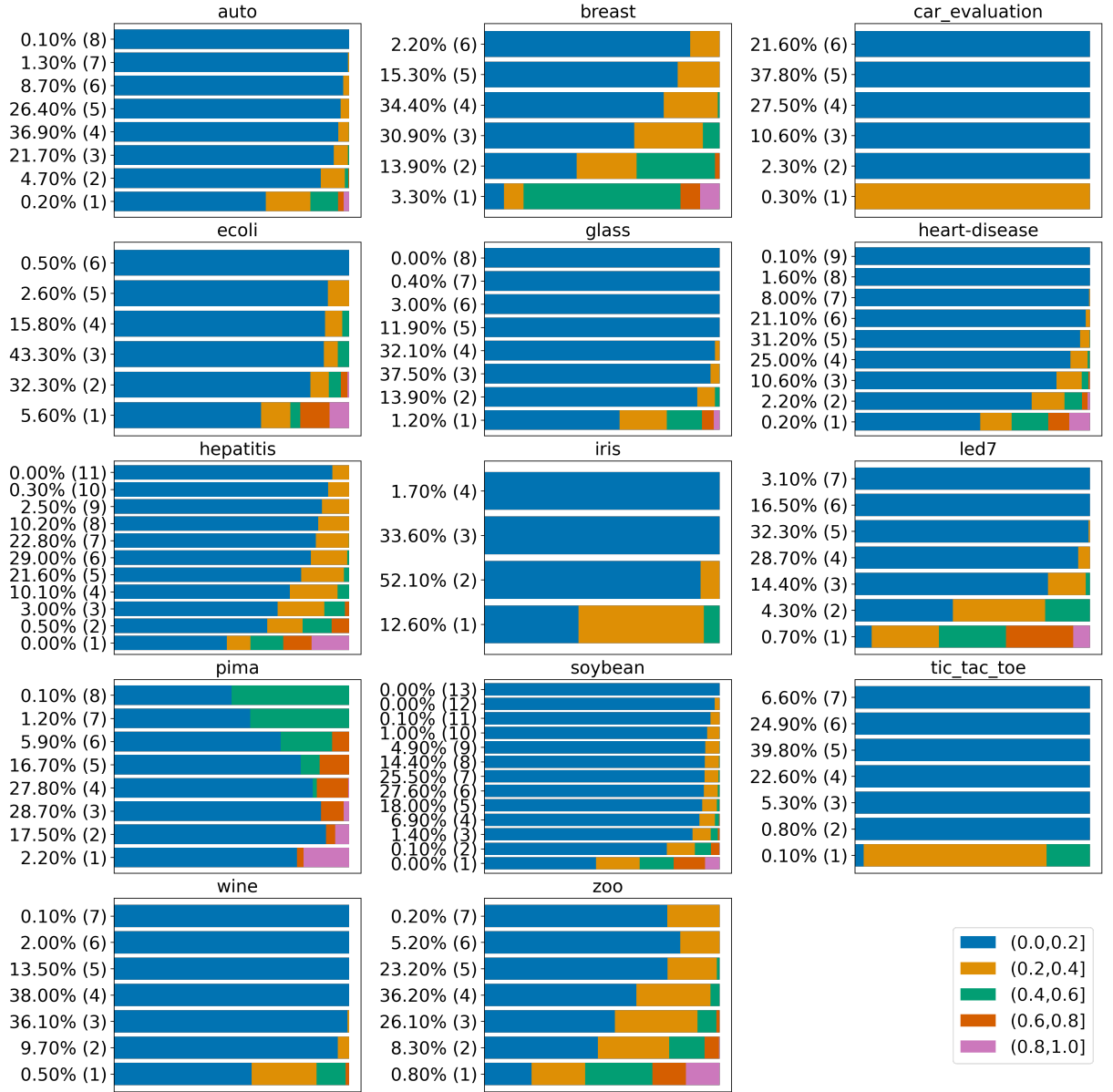
Figure 3.12: Distribution of closed itemsets within 5 frequency bins by the closure levels. The horizontal bars represent closure levels, the level number is given in parentheses. The rightmost value is the percentage of closed itemsets |\mathcal{C}_k|/|\mathcal{C}| . The width of the bar is proportional to the ratio of \mathcal{C}_k of frequency (v_1, v_2] among \mathcal{C}_k
