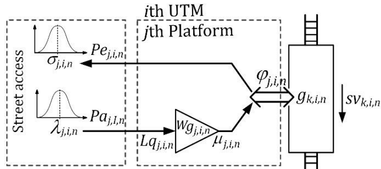
Figure 4.1. Metro queuing model of a single platform.
