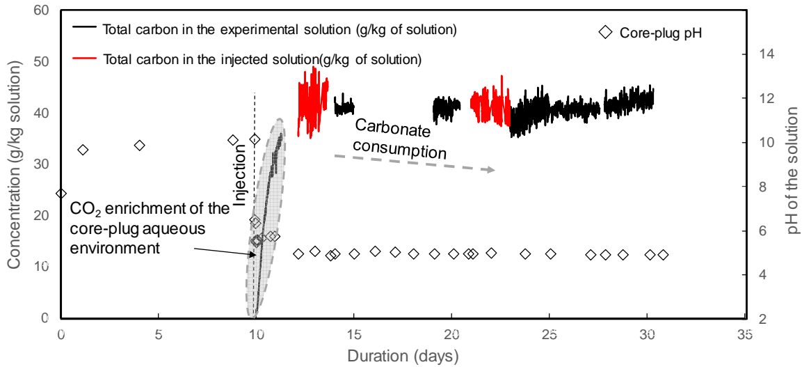
Figure 67: 21d experiment of injection of CO 2 laden equilibrated solution without salt: Evolution of the pH values and total inorganic carbon concentrations at the inlet and outlet of the core-plug with time (in kg per kg of solution).
