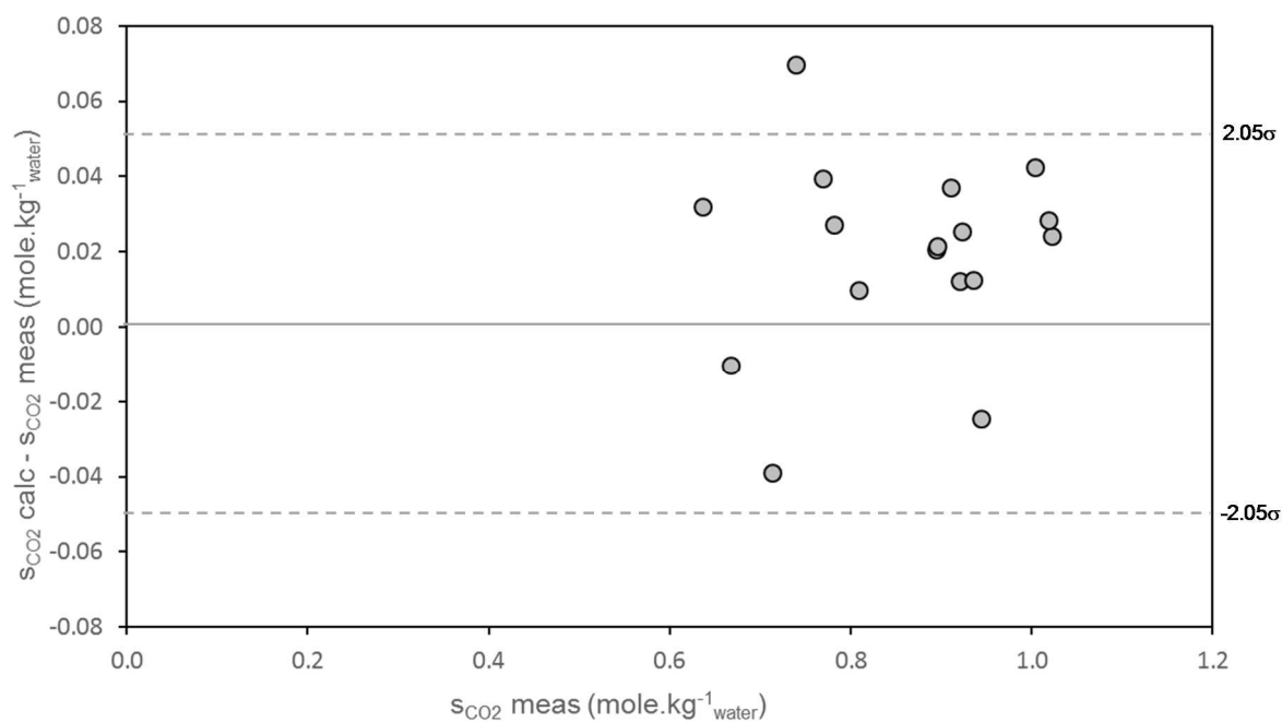
Figure C.4: Differences between the gravimetrically measured concentration of dissolved \text{CO}_2 and the dissolved \text{CO}_2 concentration calculated using the Duan and Sun (2003) model in the \text{CO}_2\text{-H}_2\text{O} system.
