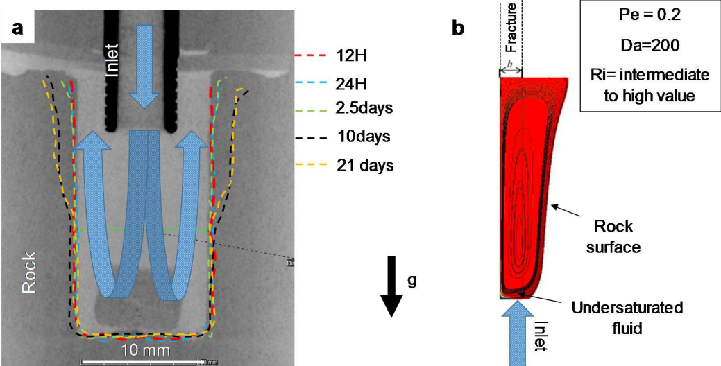
Figure 86: (a) Time dependent evolution of the well geometry. The large blue arrows indicate the fluid inlet within the injection well. The background photo illustrates the well shape of an initial sample. The different color dotted lines show the final geometry of the well for several time of acidic injection. (b) Example of Numerical buoyancy-dominated dissolution patterns obtained for Pe - Da numbers expected at the injection well after the core-plug breakthrough for intermediate to high value of the Richardson dimensionless number which reflects the significance of the buoyancy force [218]. g is defined as the gravity vector ( L \cdot T^{-2} ).
