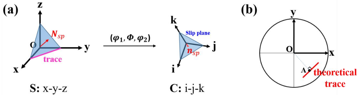
Fig. 2-9 Theoretical slip trace displayed in (a) sample coordinate system and (b) pole figure.
