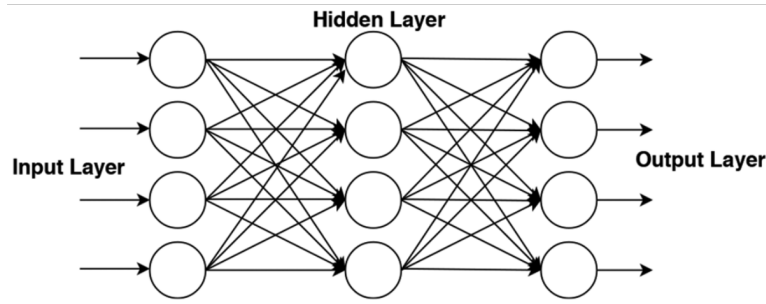
Figure 2.4: MLP concept [57].
