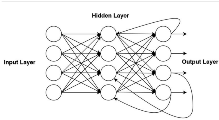
Figure 2.5: RNN concept [57].
