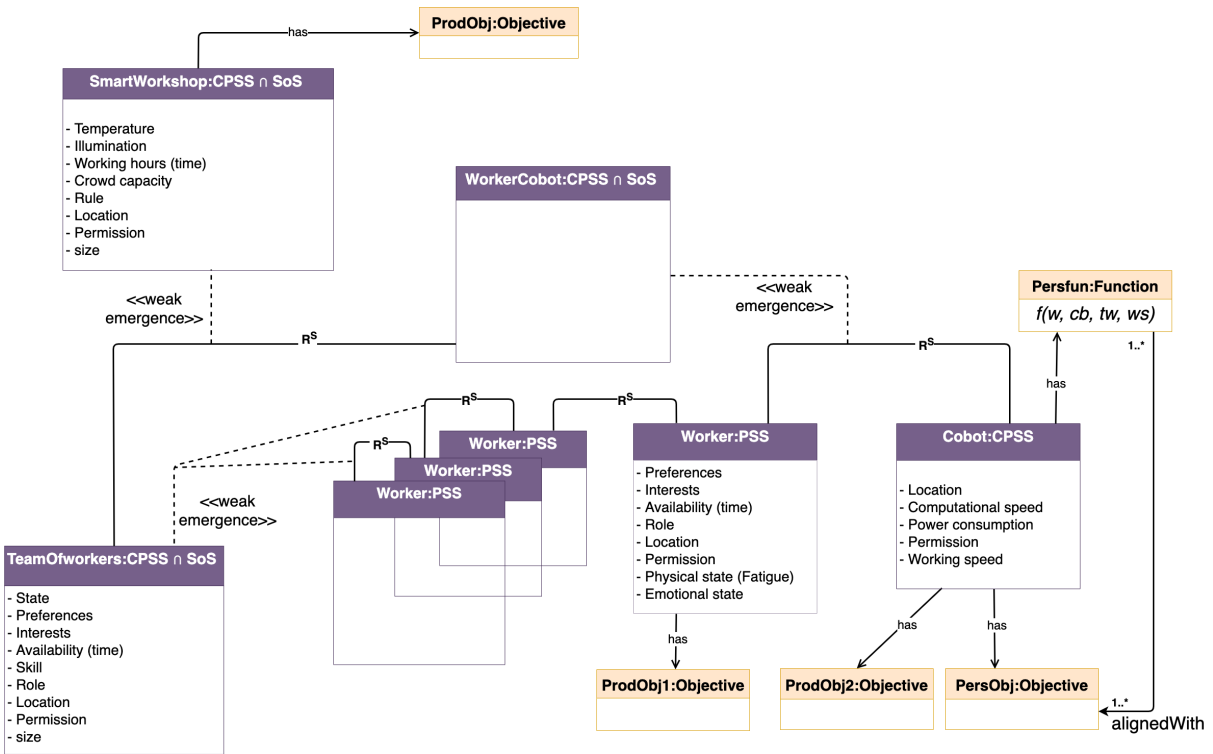
Figure 3.12: Partial instantiation of the CPSS meta-model in the context of smart workshop
