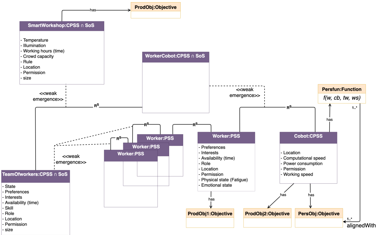
Figure 3.12: Partial instantiation of the CPSS meta-model in the context of smart workshop
