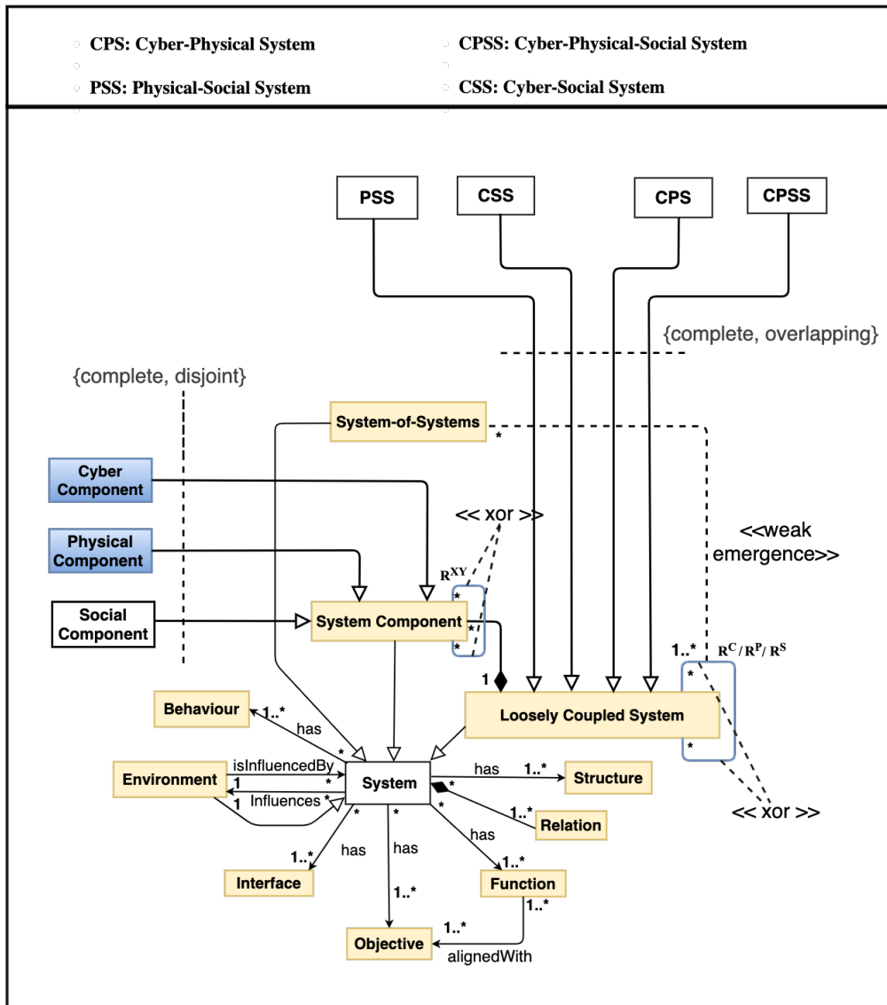
Figure 2.3: The CPSS Meta-Model Part I: systemic core.
