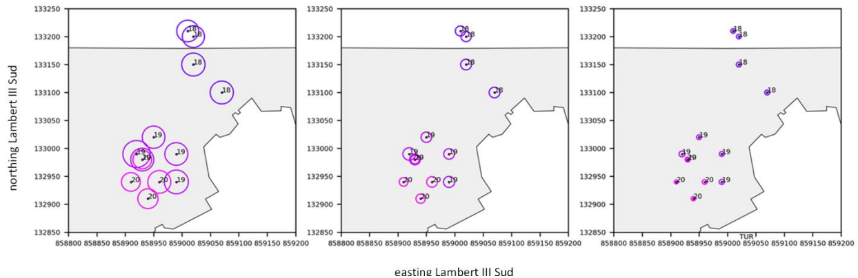
Figure 12.3 Figure shows events of northern clusters families and corresponding source radii, depending on three different assumed stress drops: a) stress drop of 0.1 MPa, b) stress drop of 1 MPa and c) stress drop of 10 MPa. Colours of events in each family match colours in Figure 11.3 and Figure 11.4.
