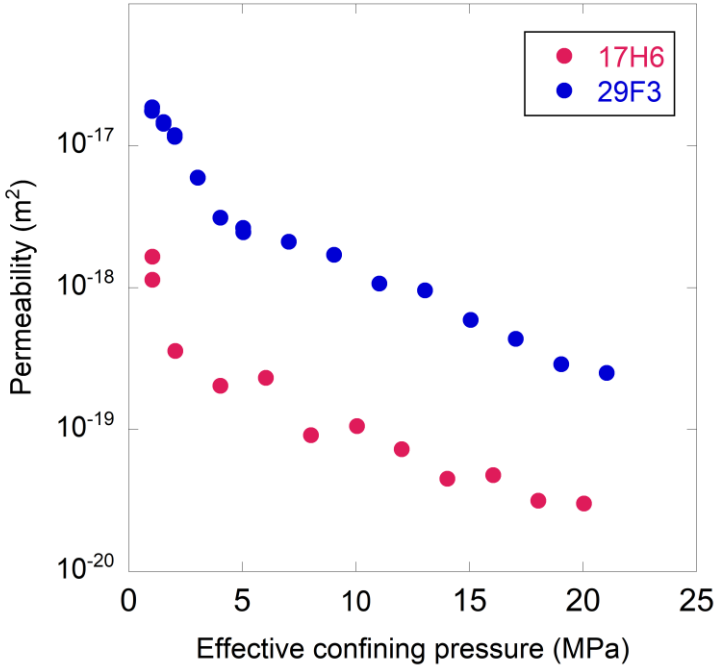
Figure 9. Permeability k as a function of effective confining pressure P_{eff} at in situ pore pressure conditions for samples 17H6 (97.43 mbsf; clayey silt) and 29F3 (157.83 mbsf; alternating sand and mud layers) from Site U1517.
